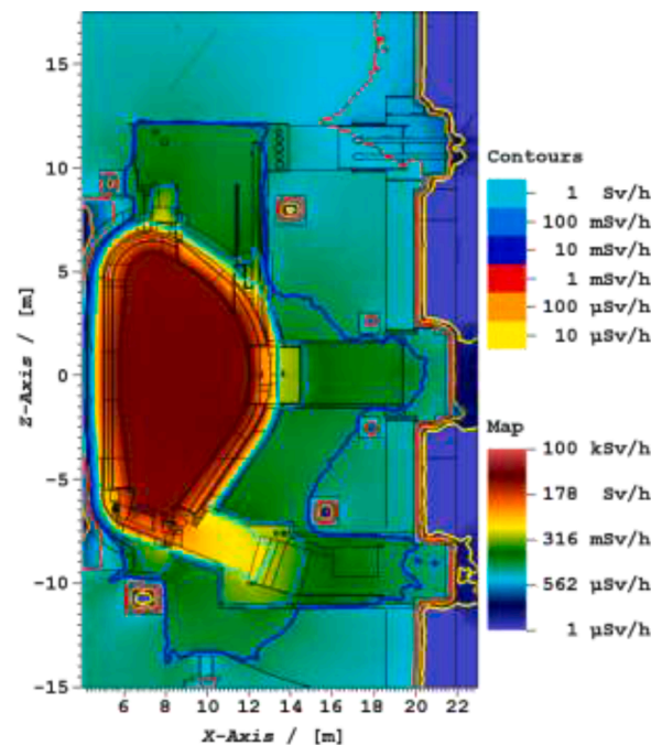
Fig. 3. Estimated dose rate in DEMO in a vertical plane through the port centre at the start of maintenance, approximately 1 month after deuterium-tritium plasma operations.
