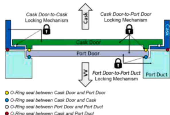
Fig. 21. Contamination Control Door (CCD) concept applied to a vessel cask
