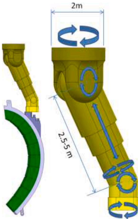
Fig. 11. Crane-lifted in-line manipulator concept.
