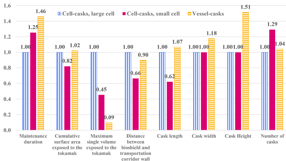
Fig. 20. Comparison of metrics for the large cell, small cell and the vessel cask approaches for the maintenance of the Lower Port.
