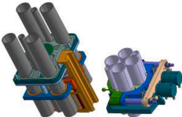
Fig. 24. –Mechanical Pipe Connector designs: concept design 1 (left), concept design 2 (right).
