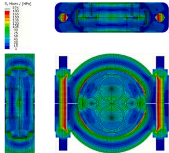
Fig. 25. Finite Element study of MPC concept design 2. Mid-plane equivalent stress distributions at 550°C and 96 bar (third angle view).
