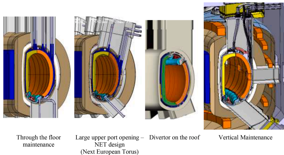
Fig. 2. DEMO port configurations considered for down-selection in 2013
