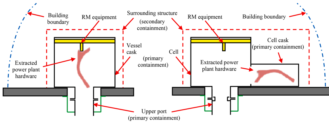
Fig. 18. Illustration of alternative confinement approaches: vessel cask (left), cell cask (right)
