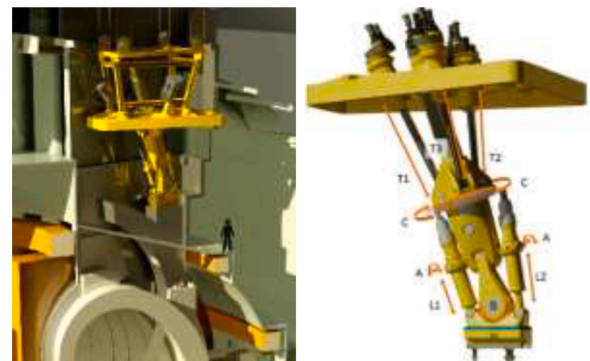
Fig. 13. Left: concept of HKM blanket mover operation (crane lift of HKM attached to Outboard Breeding Blanket segment); right: Detail of the six degrees-of-freedom of the HKM
