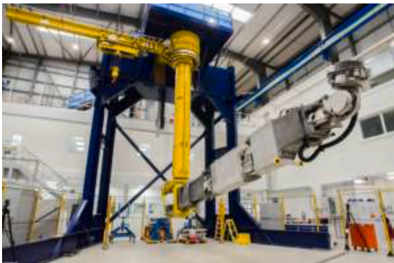
Fig. 28. Refurbished TARM installed on a bespoke remote maintenance testing stillage at UKAEA.
