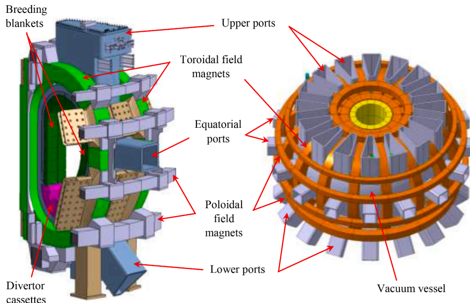
Fig. 1. Left: section view of one machine sector; right: the magnetic cage, vessel, and ports
