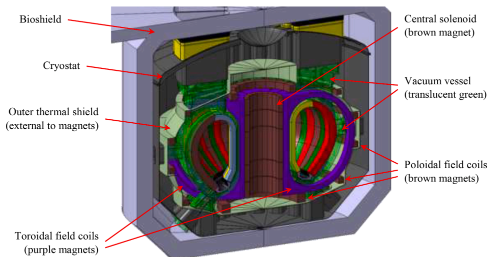
Fig. 4. Cross-section of DEMO within the bioshield.
