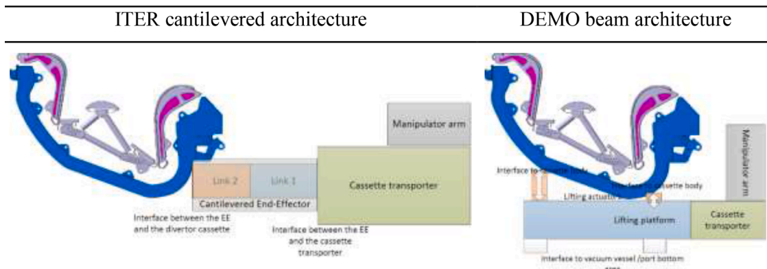
Fig. 14. Divertor transporter architecture comparison
