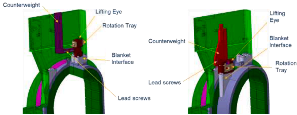
Fig. 10. Crane-lifted counterbalance concepts
