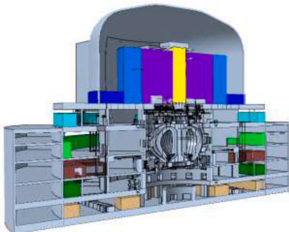
Fig. 17. DEMO space requirement analysis: maintenance volumes are shown as coloured blocks
