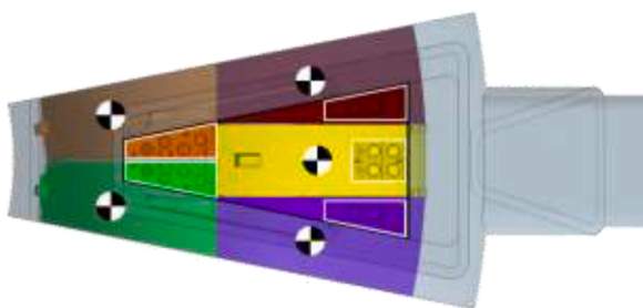
Fig. 7. Plan view on one sector (22.5°) of the vessel (grey), showing 5 blanket segments (coloured) together with their pipe connections and centres of mass relative to the port.
