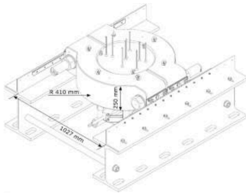
Fig. 26. Mechanical Pipe Connector proof-of-principle test bench isometric views
