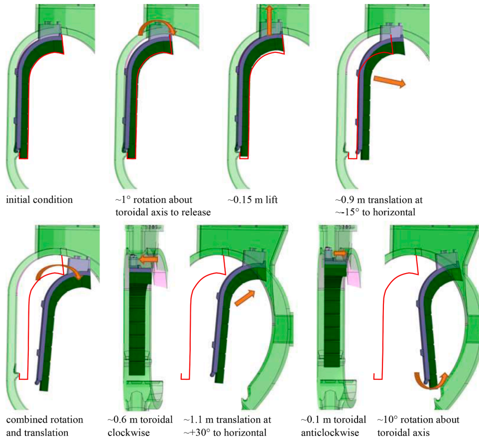
Fig. 8. Typical sequence of operations for Inner Breeding Blanket (IBB) removal, with adjacent blanket indicated in red outline
