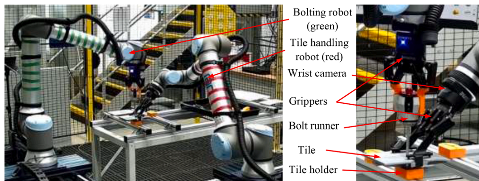
Fig. 30. Automated tile replacement
