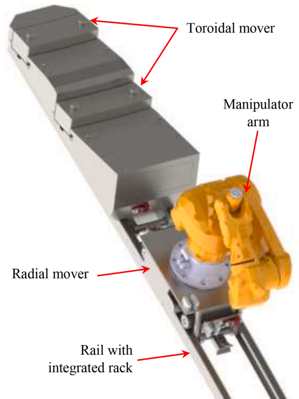
Fig. 15. Divertor Cassette Transporter.
