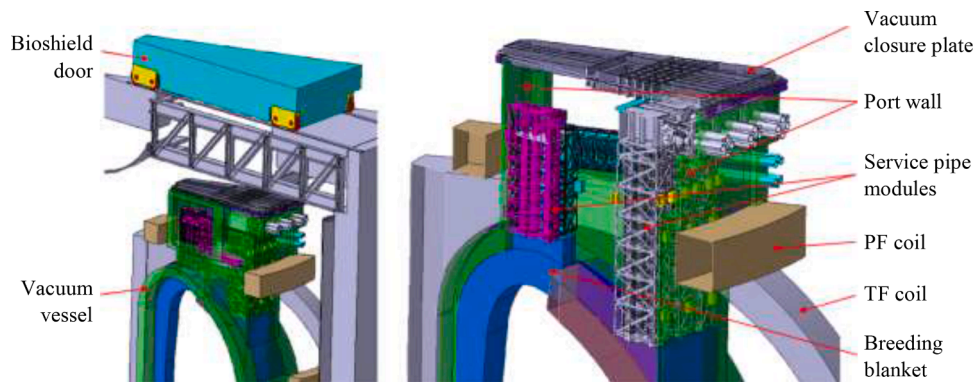
Fig. 6. DEMO upper port architecture from the 2017 proposal
