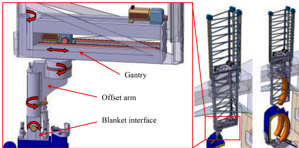
Fig. 9. Gantry crane with end-effector on a telescopic frame.
