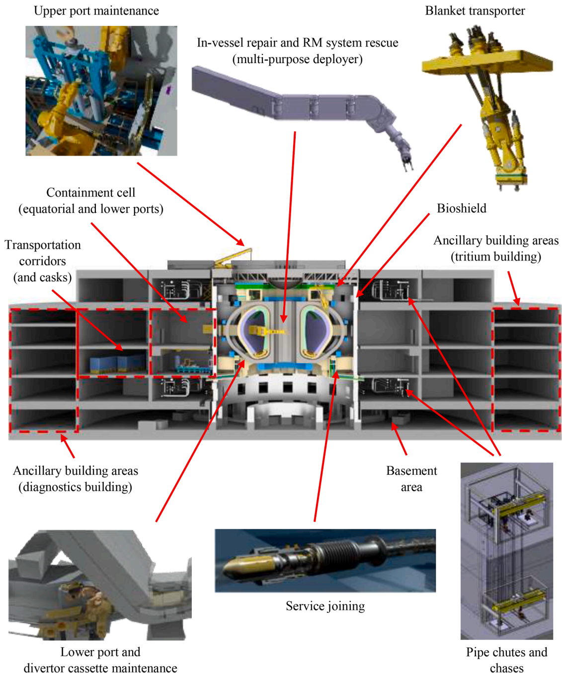
Fig. 16. Cross-section of DEMO reactor building concept accounting for remote maintenance space requirements (upper maintenance hall omitted for clarity)
