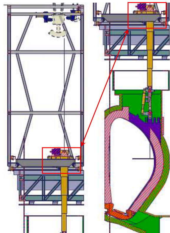
Fig. 12. End-effector mounted on a telescopic mast.
