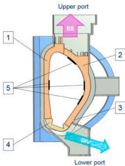
Fig. 5. Key in-vessel components to be exchanged and their entry-egress routes
