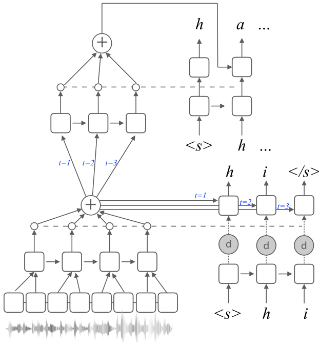
Figure 4: Attention-passing model.
