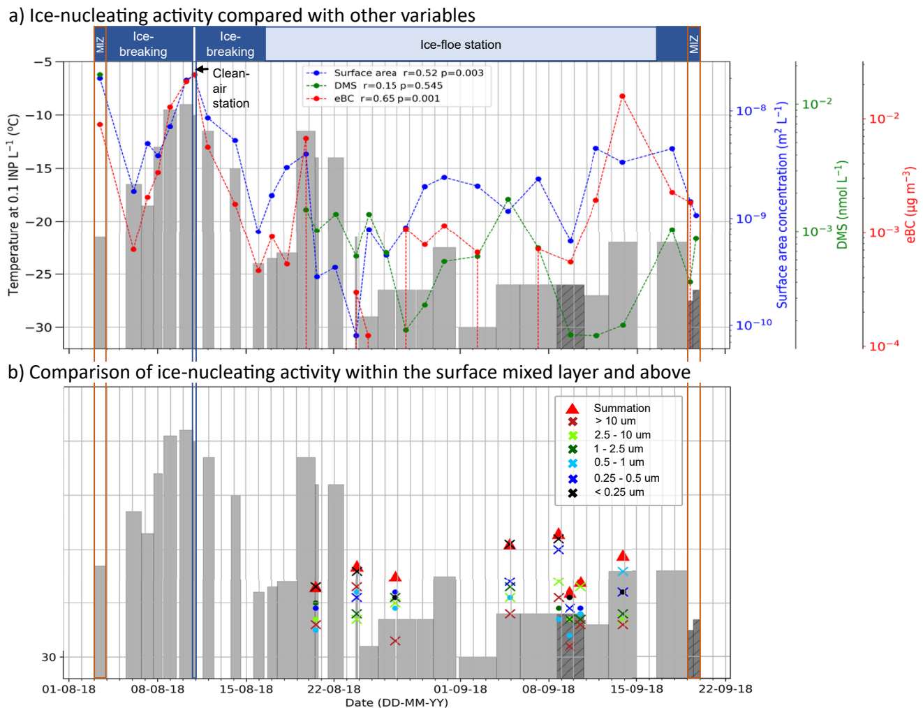
Figure 3. Time series showing the ice-nucleating activity (expressed as the temperature at which a concentration of 0.1 INP L -1 ( T_{\text{INP}=0.1} ) was observed) throughout the campaign alongside dimethyl sulfide (DMS), aerosol surface area and equivalent black carbon (eBC). In both panels a and b, the tops of the gray bars represent T_{\text{INP}=0.1} in the surface mixed layer (i.e., at ship level, 25 m above mean sea level), with the width of the bar representing the period over which air was sampled. The hatched gray bars are limiting values (where droplet freezing was indistinguishable from the control experiments). (a) The time series of the daily average surface area of aerosol per liter (blue), the DMS concentration (green) and the eBC concentrations (red) measured in the aerosol are shown. We also show the Pearson's r coefficient between ice-nucleating activity and each quantity in the figure legend. (b) The values of T_{\text{INP}=0.1} measured above the surface mixed layer (using the SHARK balloon-borne sampler) are shown against T_{\text{INP}=0.1} measured at ship level (gray bars). The red triangles are the T_{\text{INP}=0.1} for the summed INP concentrations across all size categories (comparable to the measurements at ship level), while the crosses indicate the T_{\text{INP}=0.1} associated with each size category (circles indicate limiting values). The dates for the respective periods are: MIZ 02/08/18–03/08/18, Clean-air station 10/08/18–11/08/18, Ice-breaking 03/08/18–16/08/18, Ice floe station 16/08/18–15/09/18, Ice-breaking 15/09/18–19/09/18, MIZ 19/09/18.
