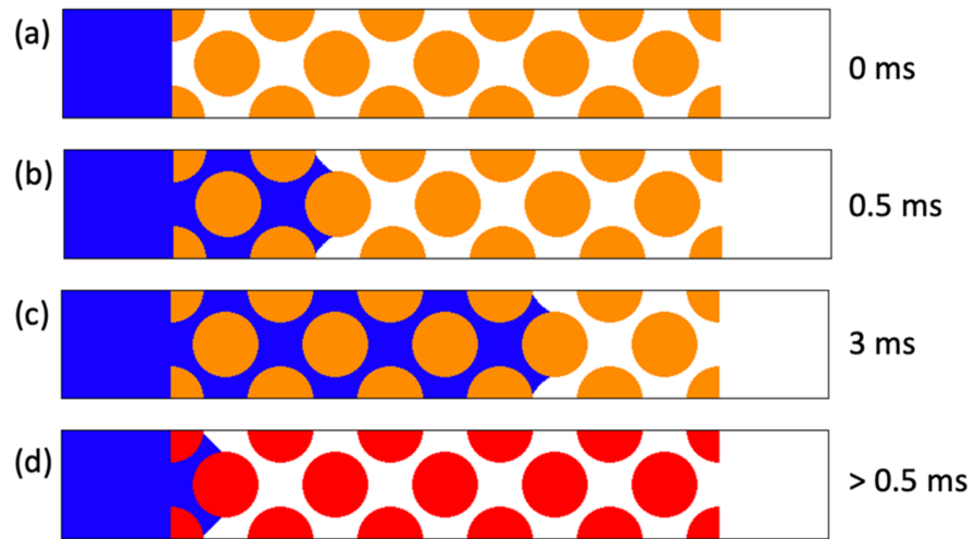
Figure 10. Infiltration for homogeneous coating with CA = 50° at (a) simulation start, (b) 0.5 ms, (c) 3 ms as well as (d) the equilibrium state for homogeneous coating with CCA (red) 54° for >0.5 ms.
