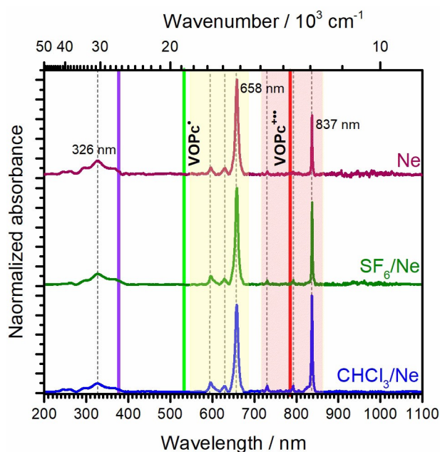
Figure 2. UV/Vis-NIR absorption spectra obtained upon depositing cationic VOPc into Ne matrix at 5 K (top panel). Assignments and positions of the main spectral features are indicated. Spectral features in the yellow and pink shaded regions are assigned as the signatures of VOPc* and VOPc*** respectively. Note the presence of both neutralized and cationic VOPc in the same matrix. Electron scavengers SF 6 and CHCl 3 were used to enhance the relative concentration of the cationic species w.r.t the neutrals (bottom panels). Dashed gray lines highlight the positions of absorption bands common to all three spectra. Purple, green, and red lines denote the central wavelengths of laser diodes used for LIF (see text).
