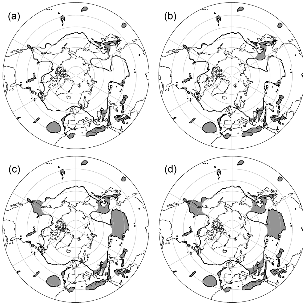
Figure 5. Sensitivity of the identification process to the width threshold w . Here, w equals (a) 500 km, (b) 1000 km, (c) 1500 km, and (d) 2000 km, using the example of the 330 K isentropic from the ERA5 reanalysis on 14 July 2015, 00:00 UTC. Results are not filtered to highlight the effect of the parameter. Our default configuration is (c).
