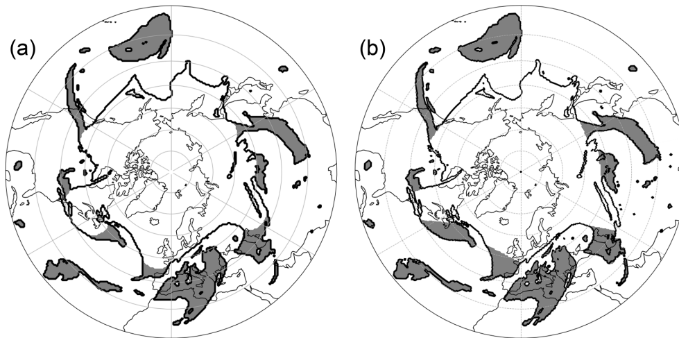
Figure 7. Comparison of the identified PVSs based on the 340 K isentrope from the ERA5 data set on 24 July 2015, 00:00 UTC. (a) Results of our strategy using the default configuration and (b) by the algorithm from Wernli and Sprenger (2007). The anomaly over East Asia will be investigated in the case study later on.
