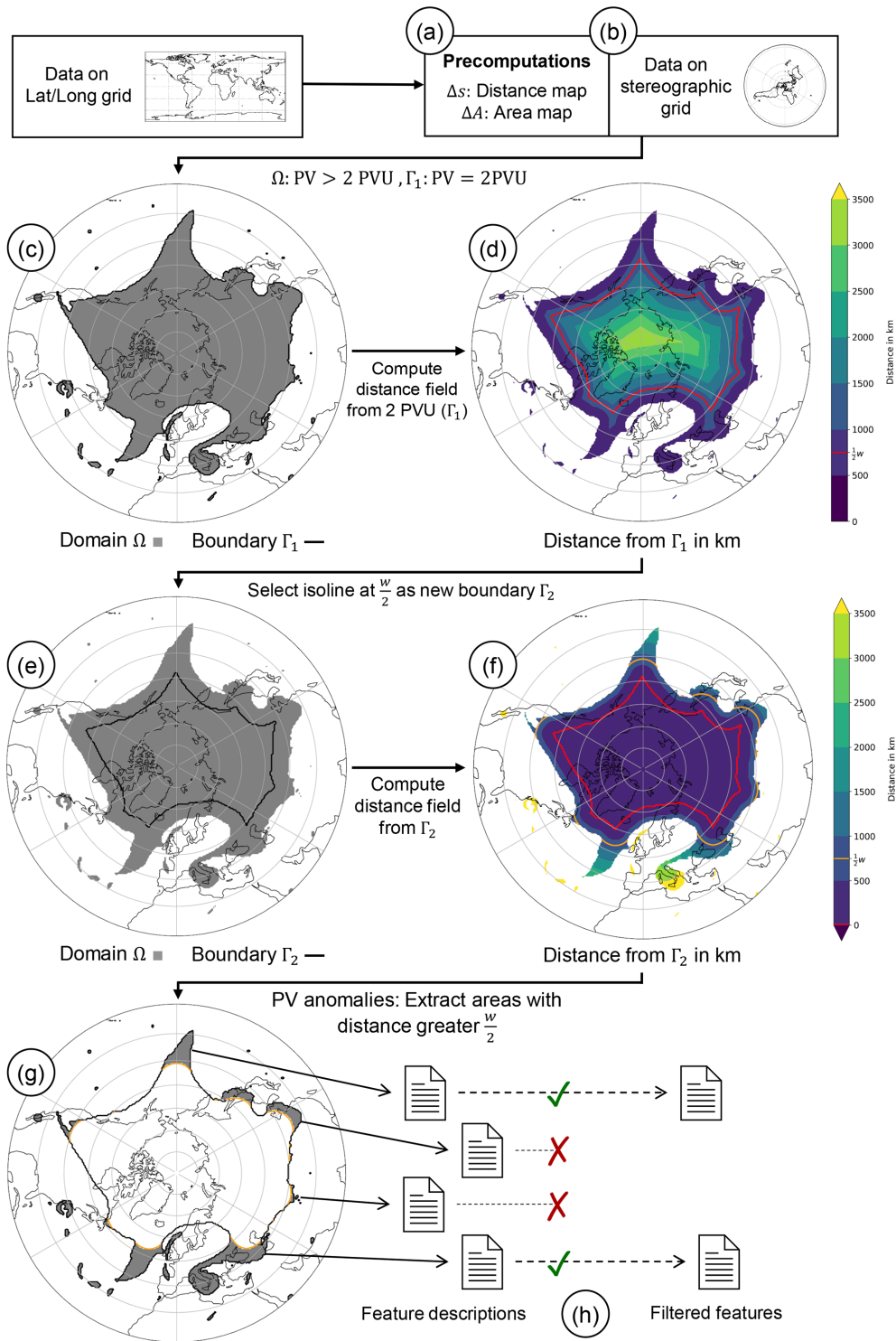
Figure 4. Illustration of the algorithm to identify PVs. (a, b) Input data are mapped to a stereographic grid; precomputations are performed. (c, d) The distance field from the 2 PVU boundary is computed (cf. Sect. 3). Points at a distance equal to half the width threshold \frac{w}{2} are denoted by the red isoline. (e, f) From this isoline, distances outwards are computed. Again, the isoline corresponding to \frac{w}{2} is drawn with respect to the new distance field (orange). (g) Regions with a distance greater than \frac{w}{2} from (f) are extracted. They form anomalies in the field. (h) The anomalies are labeled and filtered, yielding a set of identified PVs. Visualized is the 335 K isentrope from the ERA5 reanalysis on 7 September 2016, 00:00 UTC.
