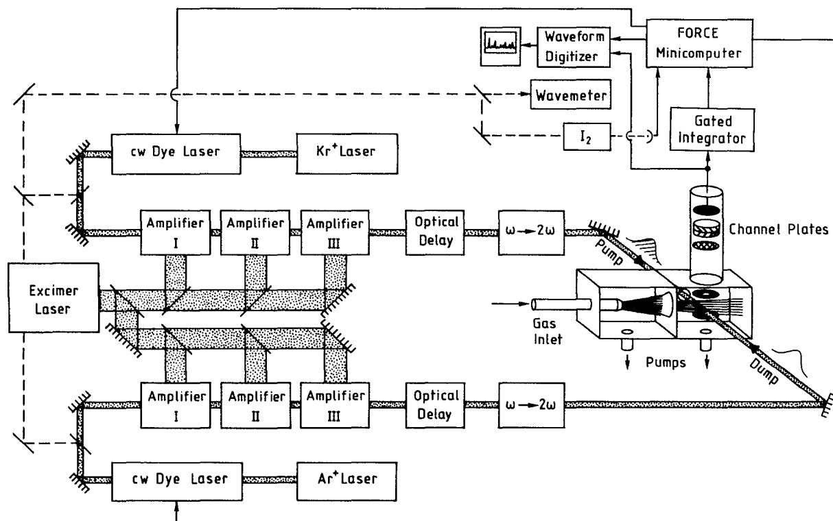
FIG. 1. The experimental setup for recording of rotationally resolved ion dip spectra of single rovibronic states of benzene. A spectral resolution of the pump and the dump lasers of \Delta\nu_{UV} < 100 MHz (FWHM) is obtained by pulsed amplification of the cw light of two single-mode dye lasers and subsequent frequency doubling. The counterpropagating pump and dump laser beams are crossed with the molecular beam produced in a skimmed supersonic jet.
