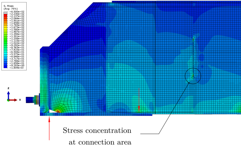
Figure 6.6: Side view of config. 2 at case 3, f_y = 223.00 \text{ N/mm}^2
