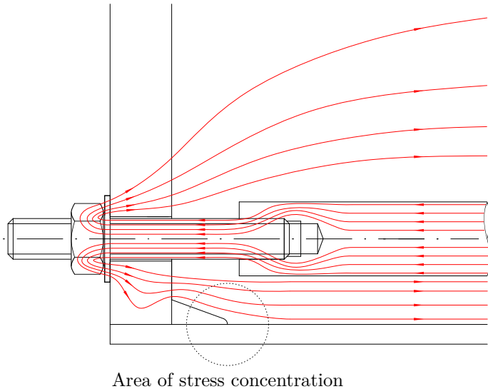
Figure 3.22: Section view of the preload zone, expected stress concentrations
