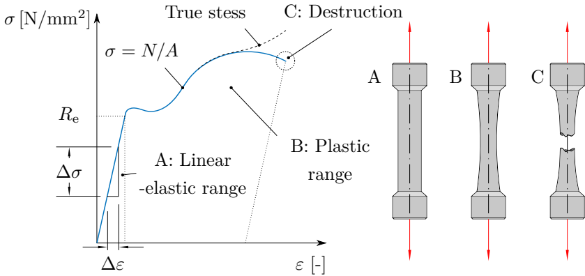
Figure 2.5: Stress-strain curve of a loaded axial rod [2, p. 15]
