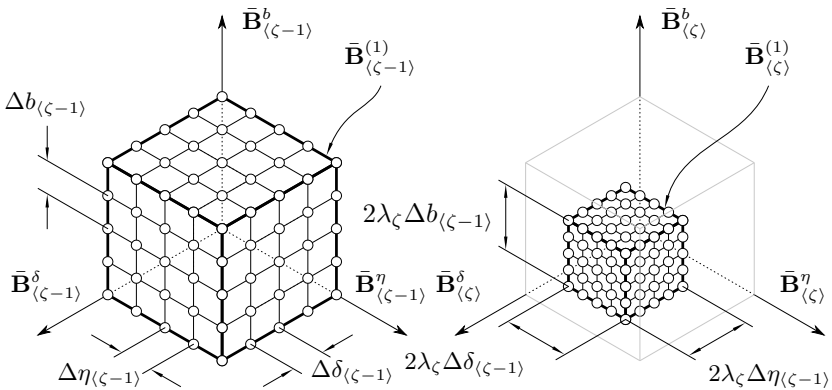
Figure 5.12: Recursive interval limitation
