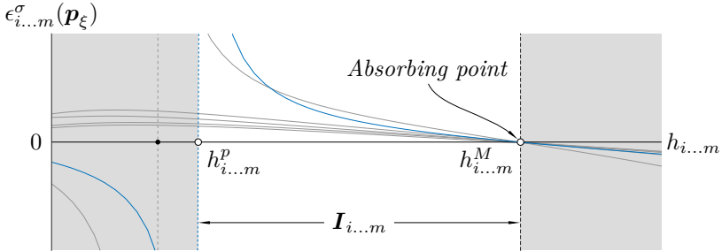
Figure 5.8: Qualitative representation of the poles
