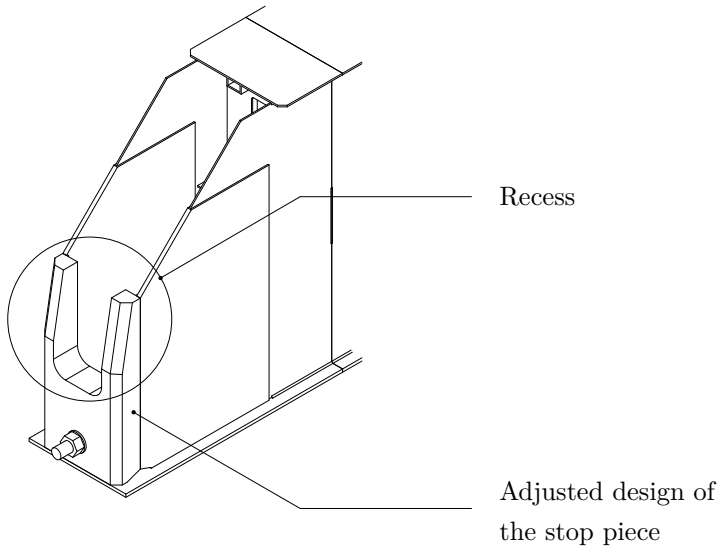
Figure 6.12: Isometric view of the improved reference configuration 3
