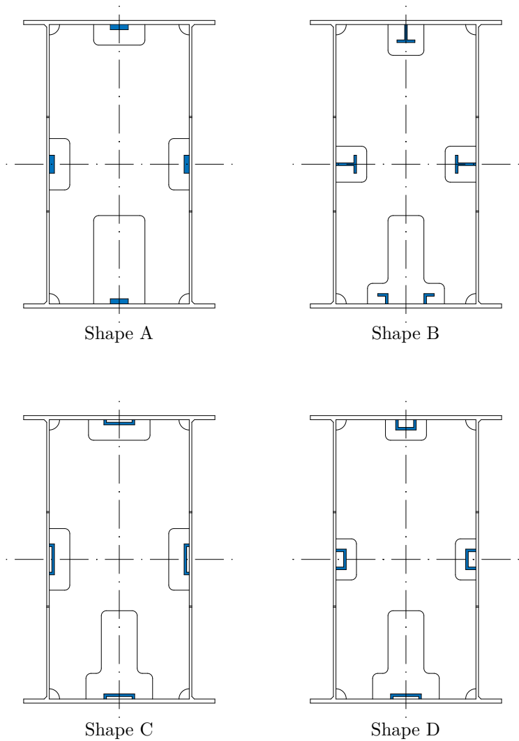
Figure 3.11: Different shape designs of stiffening ribs in order to reinforce the plates
