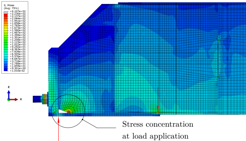
Figure 6.4: Side view of config. 1 at case 3, f_y = 223.00 \text{ N/mm}^2
