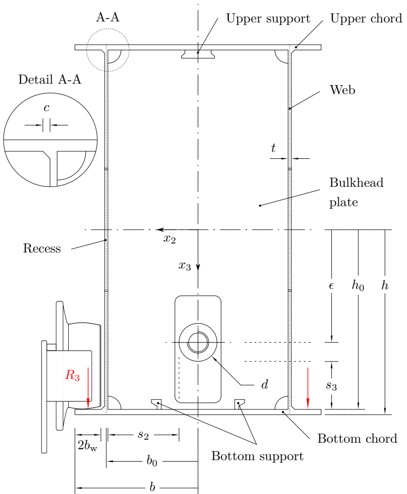
Figure 3.9: Dimensions of the main segment (front view)
