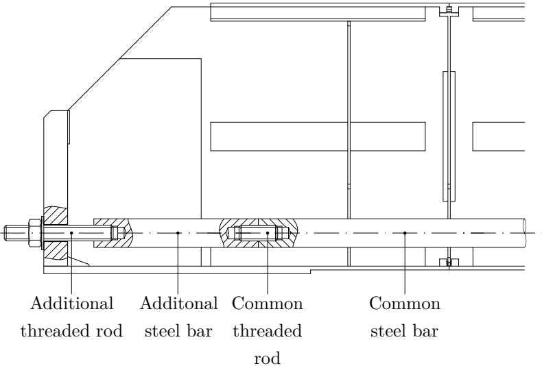
Figure 3.21: Section view of the preload zone
