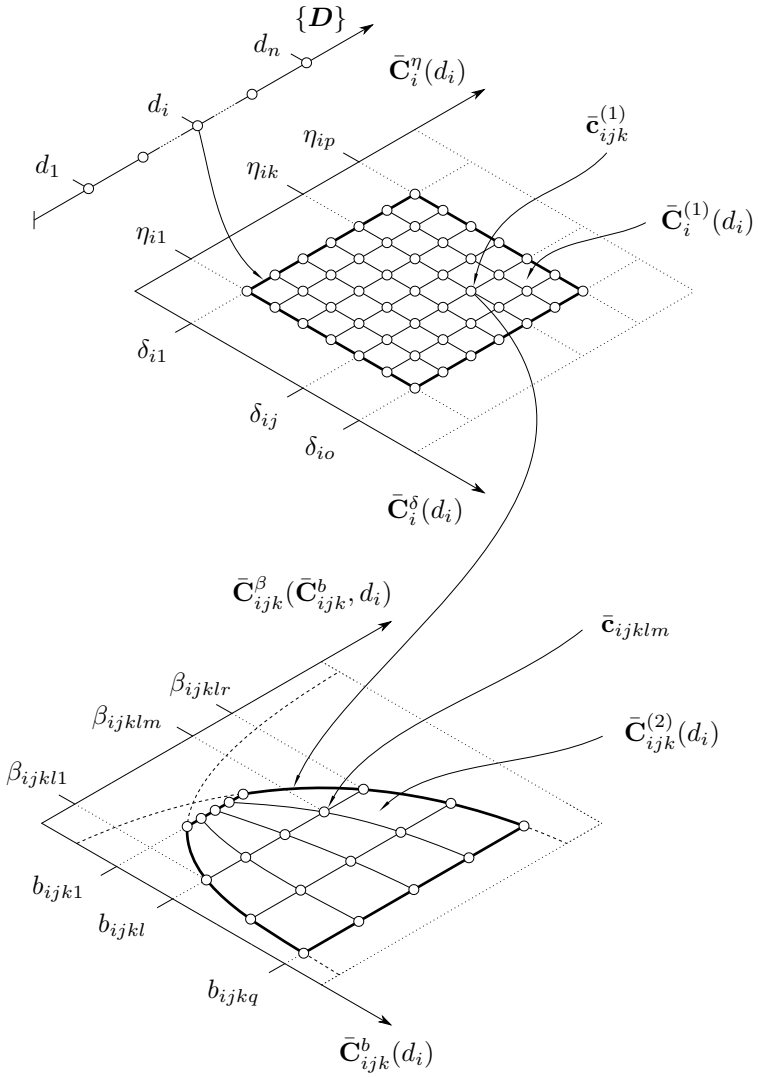
Figure 5.5: LOA - Identification of possible combinations of design variables
