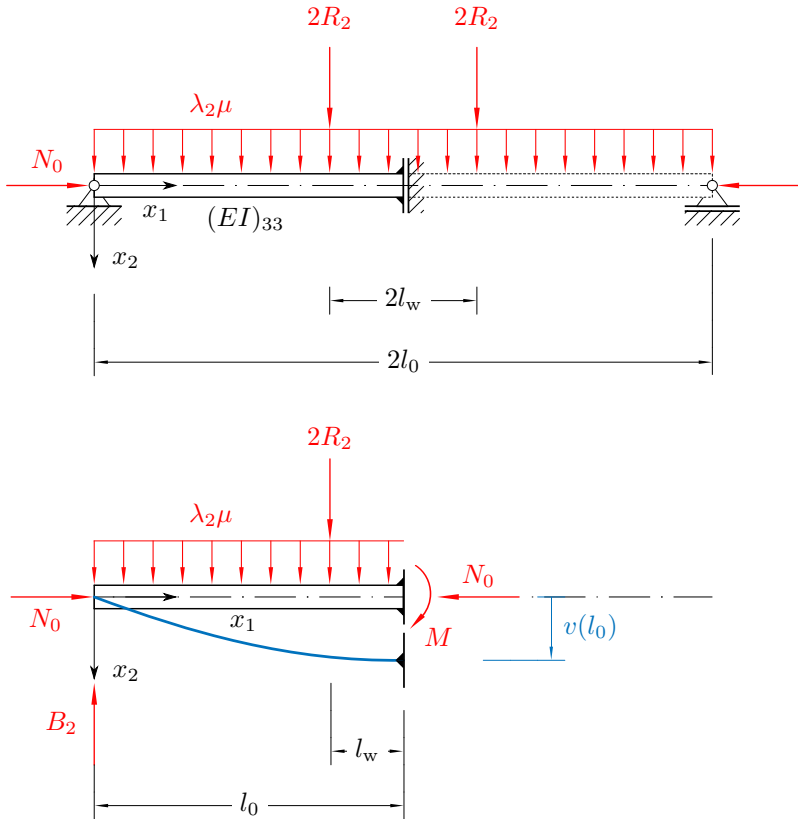
Figure 4.13: Deflection due to bumper impact in x_2 -direction
