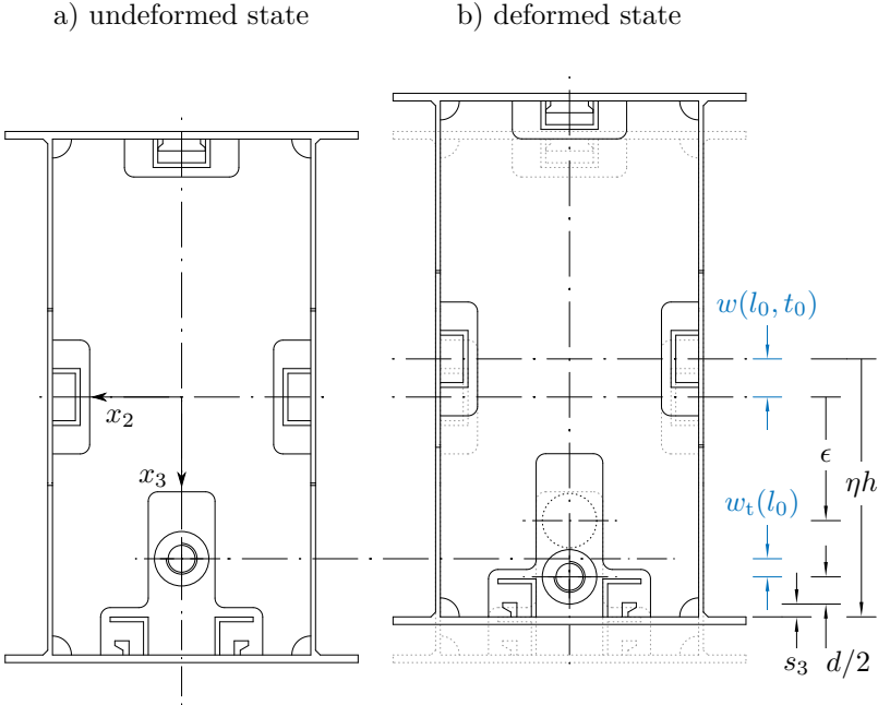
Figure 4.11: Undeformed and deformed state of the girder and the traction mechanism
