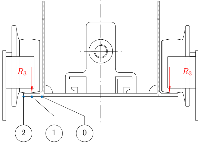
Figure 4.10: Local stresses defined in [9], parallel flange considered
