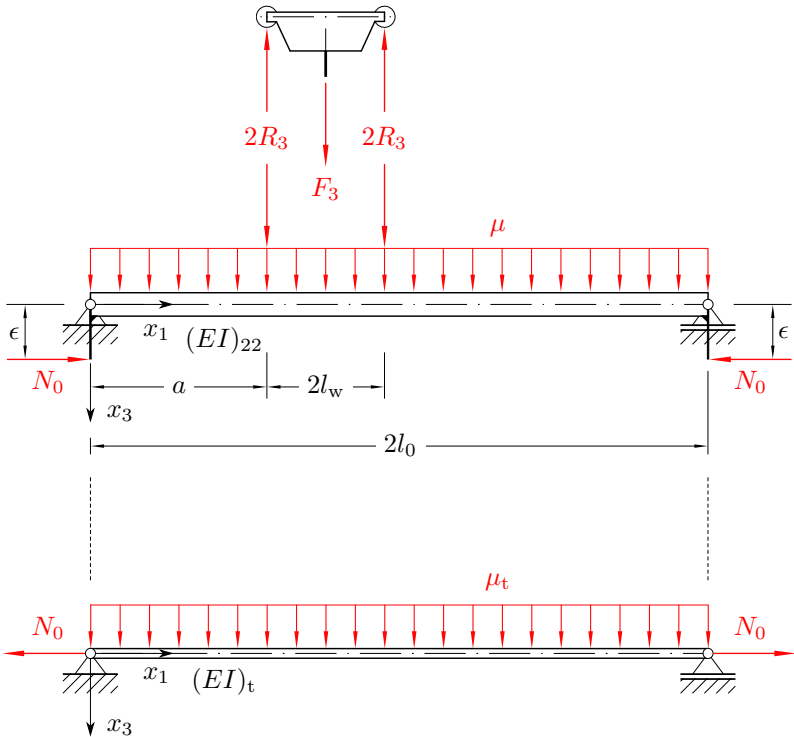
Figure 4.1: Basic mechanical model
