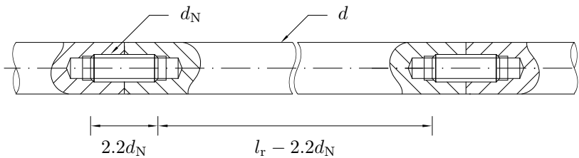
Figure 4.16: Corresponding lengths regarding the common rod connections
