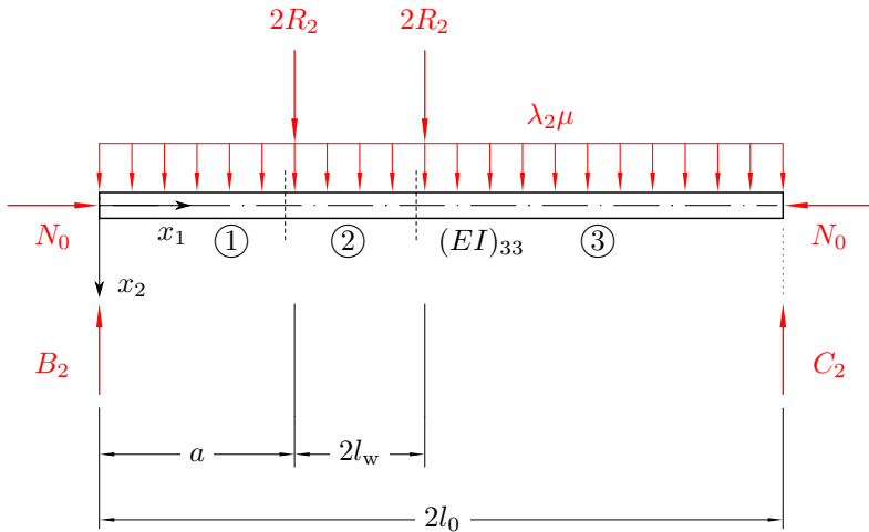
Figure 4.3: Free body diagram of the girder in terms of bending about the x_3 -axis
