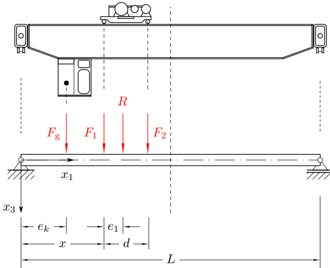
Figure 2.17: Considered crane configuration in [6] and [7]
