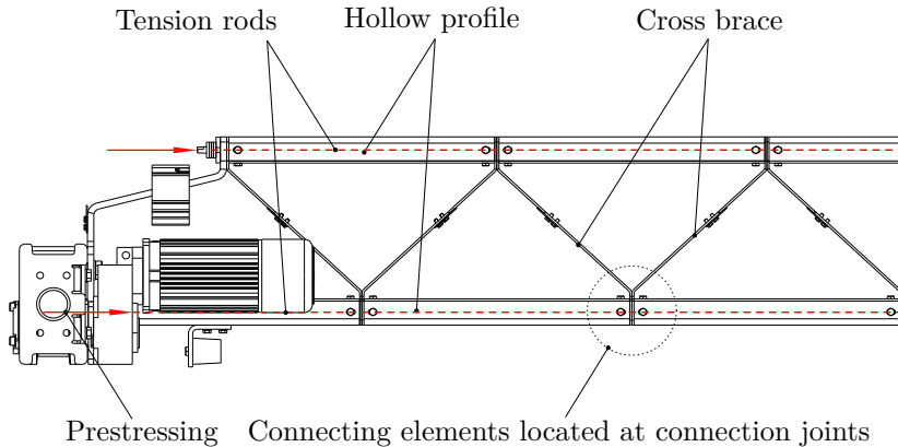
Figure 2.13: Detailed view of the scalable, modular, segmented crane [3]
