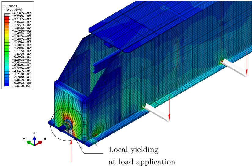
Figure 6.5: Isometric view of config. 1 at case 3, f_y = 223.00 \text{ N/mm}^2
