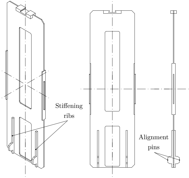
Figure 6.10: Structural improved connecting element
