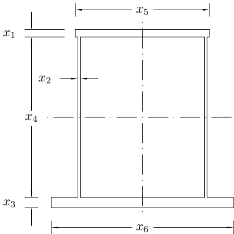
Figure 6.1: Considered design by M. SAVKOVIC et al. [10]
