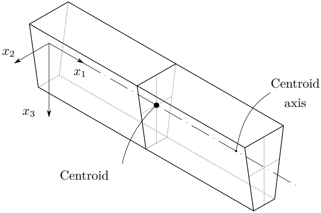
Figure 2.6: Coordinate system and defined beam axes
