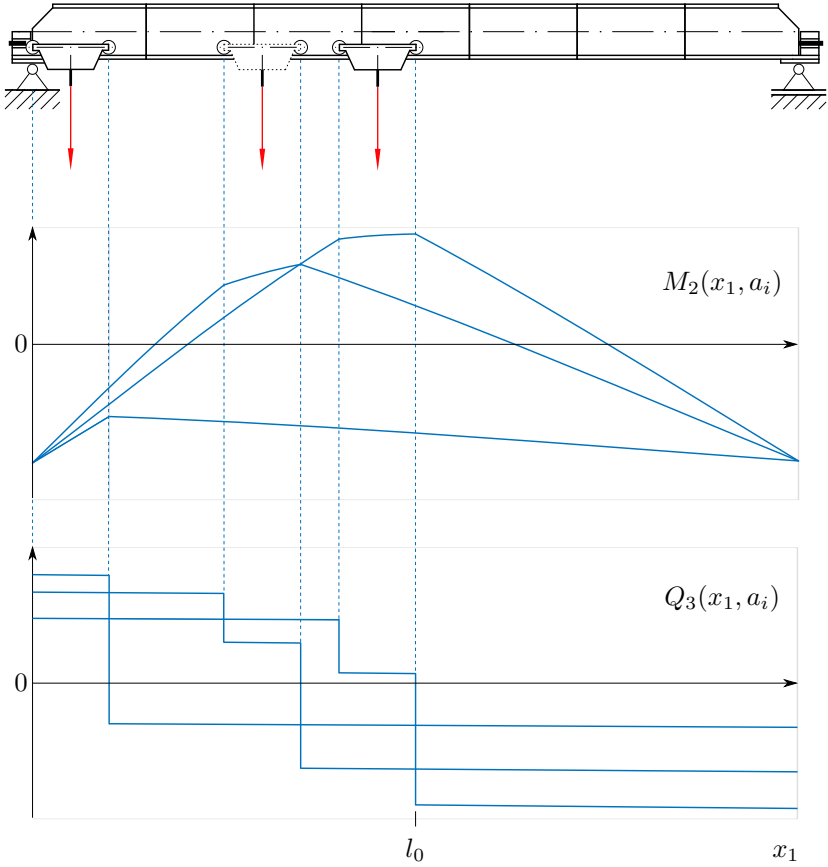
Figure 4.4: Qualitatively depicted load curves considering bending about the x_2 -axis
