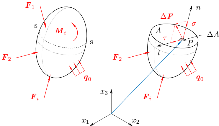
Figure 2.4: Loaded body, based on [2, p. 43]
