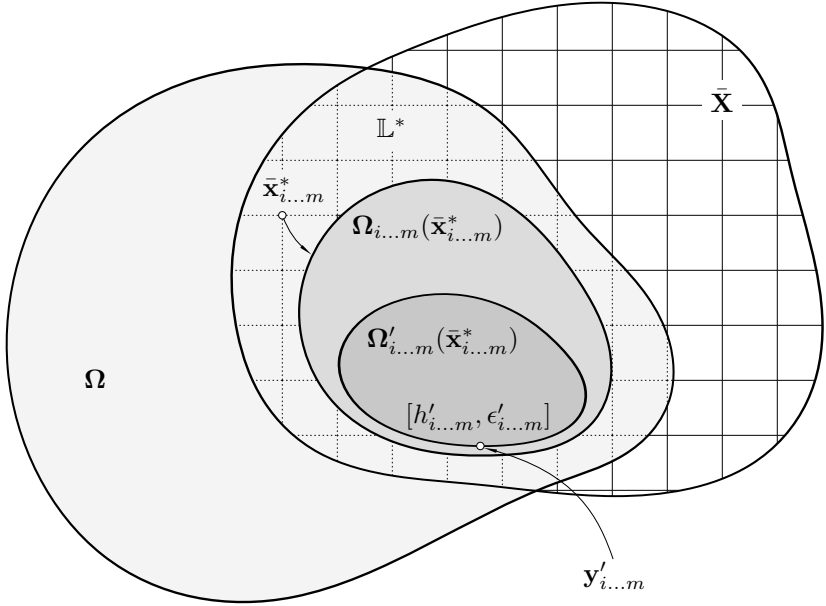
Figure 5.10: Solution approach
