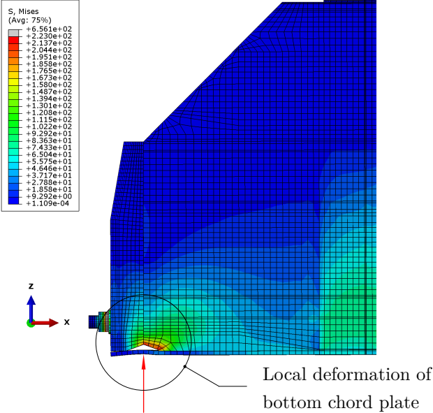
Figure 6.14: Local deformation of the bottom chord plate at the support
