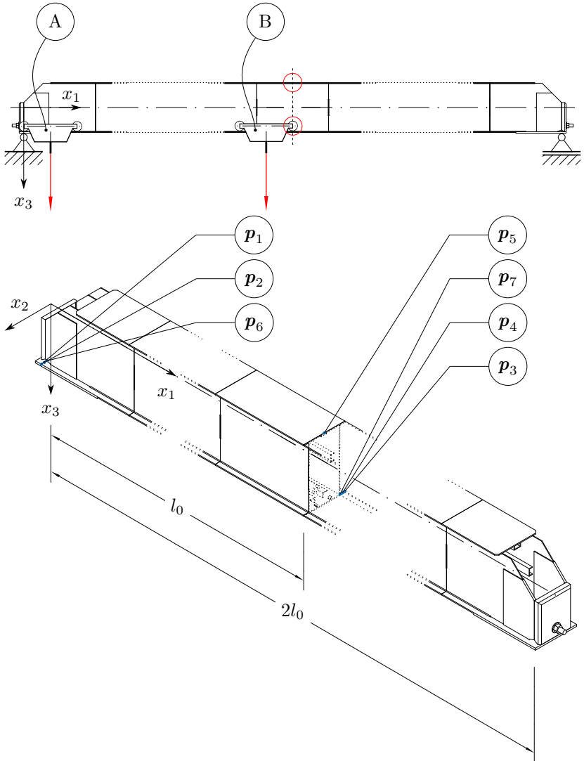
Figure 4.9: Operating conditions and identification of critical points in terms of mechanical stresses
