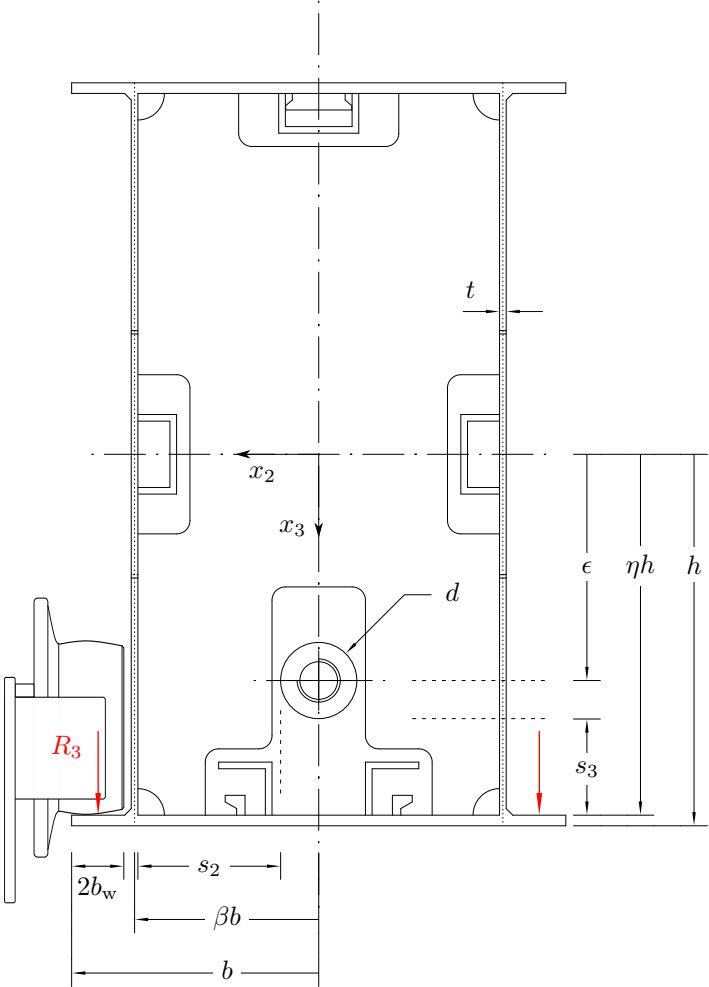
Figure 4.8: Section view of the main segment
