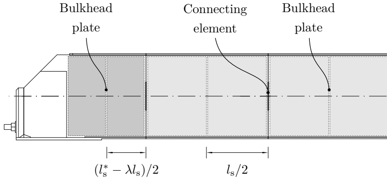
Figure 4.14: Identification of the underlying crucial plate length
