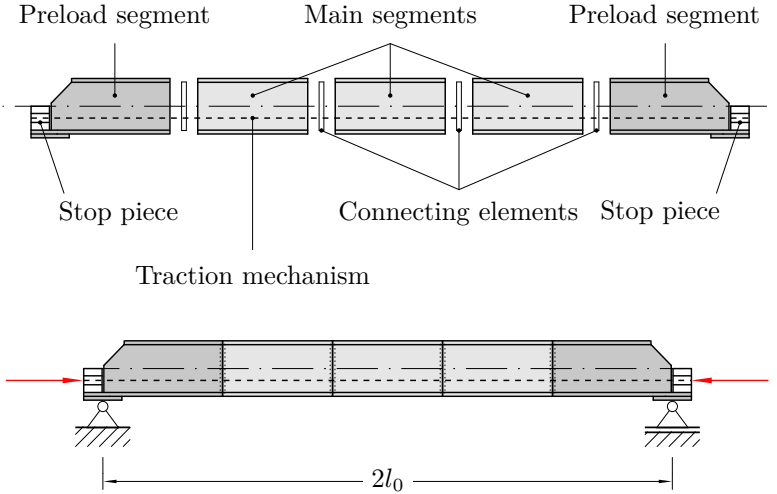
Figure 3.1: Conceptual design of the segmented, prestressed crane bridge
