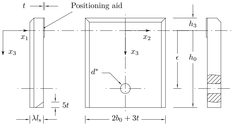
Figure 3.19: Major dimension of the stop piece
