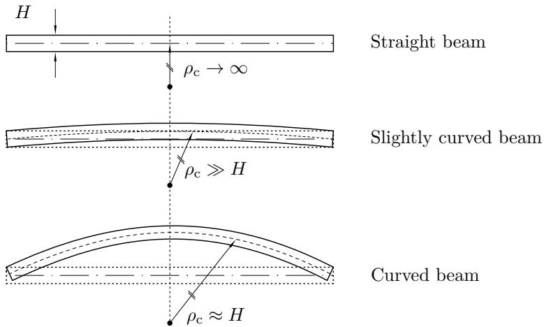
Figure 2.8: Classification of beams with respect to geometry
