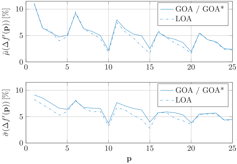
Figure 5.14: Expected values and according standard deviations in terms of relative deviations
