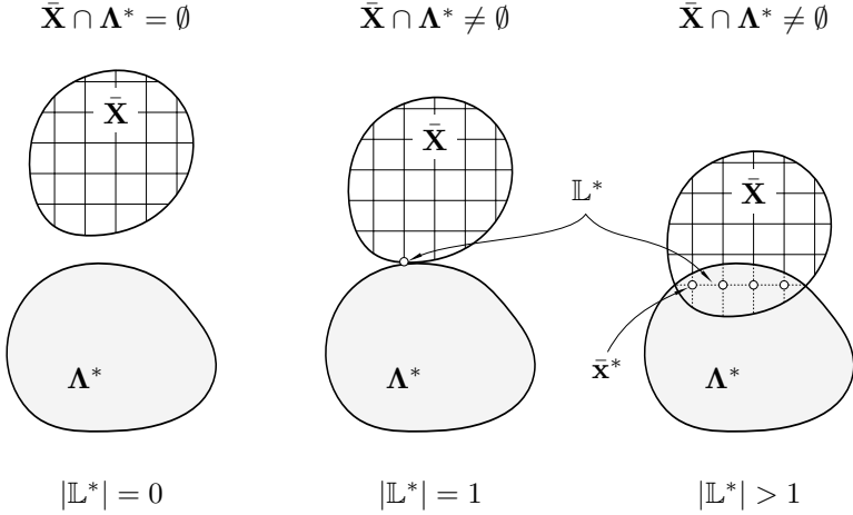
Figure 5.7: Discretization and corresponding sets
