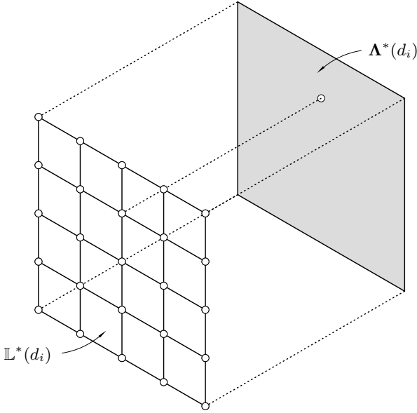
Figure 5.4: Discretization strategy
