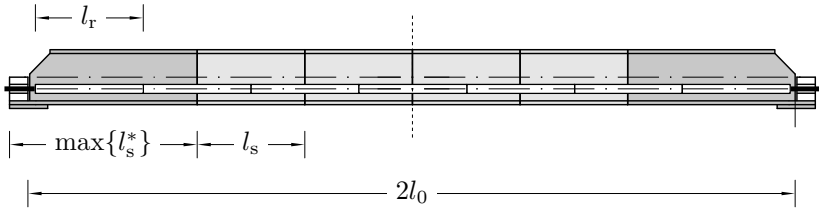
Figure 3.3: Segmentation type 2
