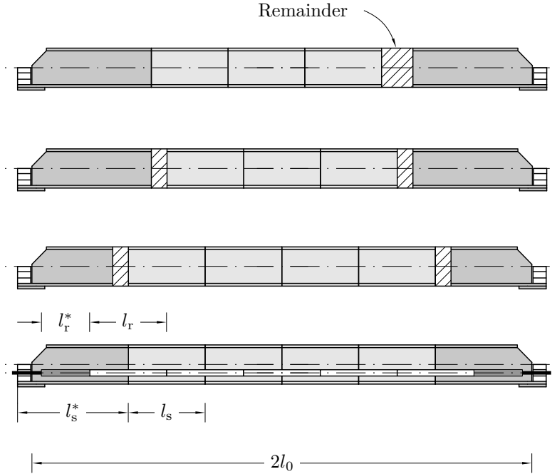
Figure 3.4: Segmentation type 3
