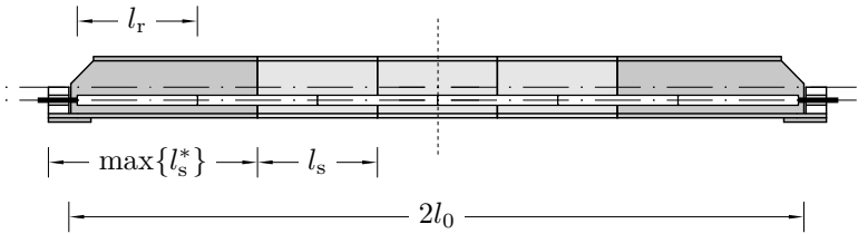
Figure 3.2: Segmentation type 1
