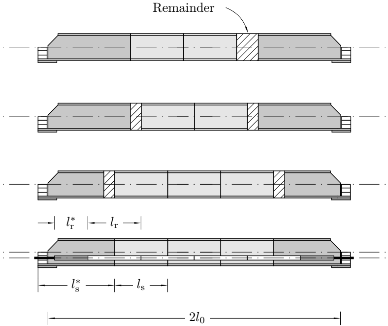
Figure 3.5: Segmentation type 4
