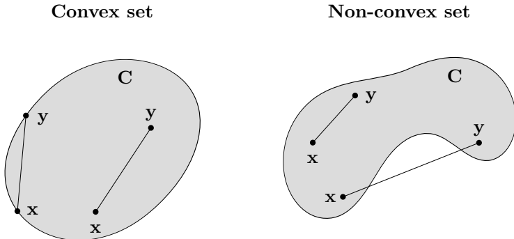
Figure 2.15: Illustration of a convex and a non-convex set in \mathbb{R}^2 [5, p. 39]
