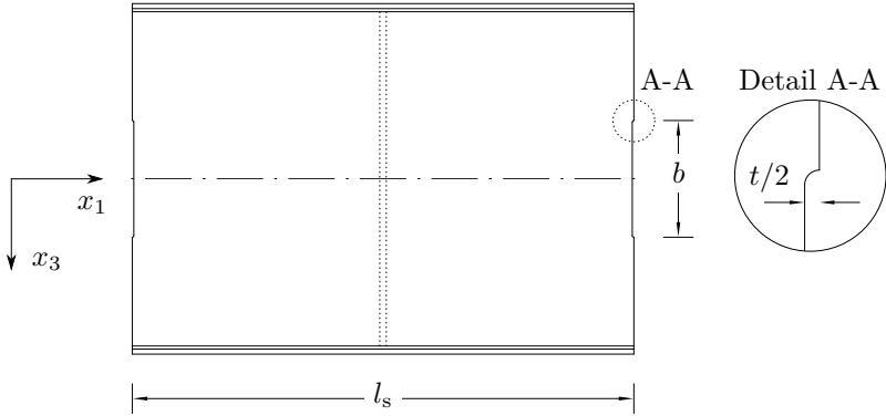
Figure 3.10: Dimensions of the main segment (side view)
