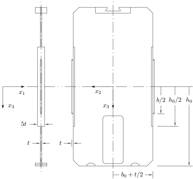
Figure 3.15: Major dimensions of the connecting element
