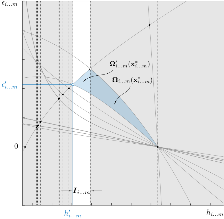
Figure 5.9: Interval limitation
