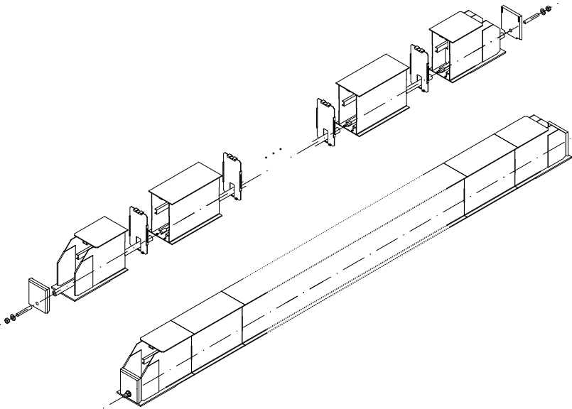
Figure 3.23: Assembly sequence
