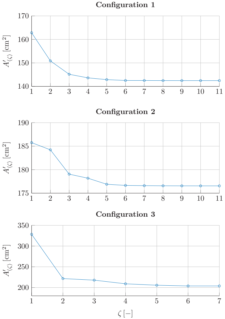
Figure 6.2: Calculated minimum cross-sectional areas depending on the recursion step
