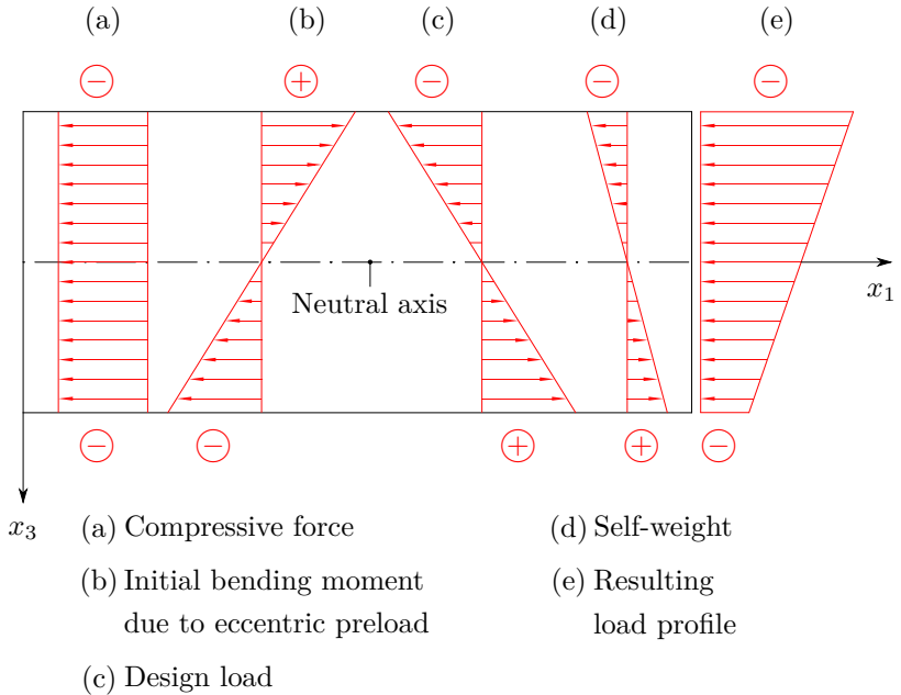
Figure 3.6: Expected load profile regarding a load application at x_1 = l_0
