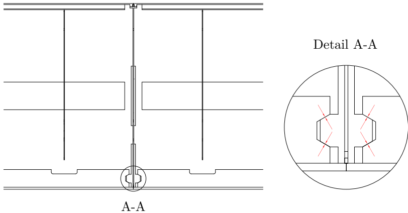
Figure 6.11: Detailed view of the connecting zone
