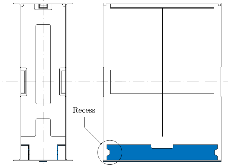
Figure 6.9: Structural improved main segment
