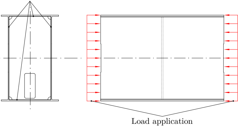
Figure 3.12: Supporting conditions during stability analyses
