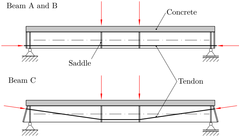
Figure 2.14: Considered configurations of tensile members according to [4], beam type specified in table 2.1
