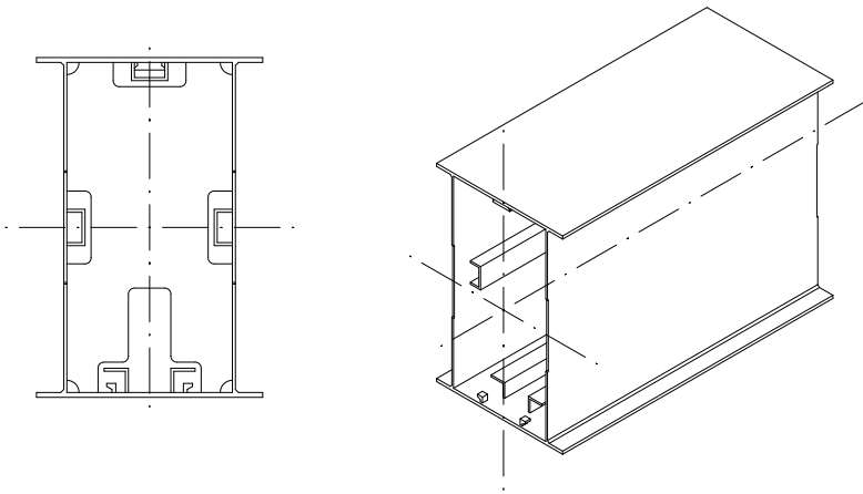
Figure 3.14: Final design of the main segment
