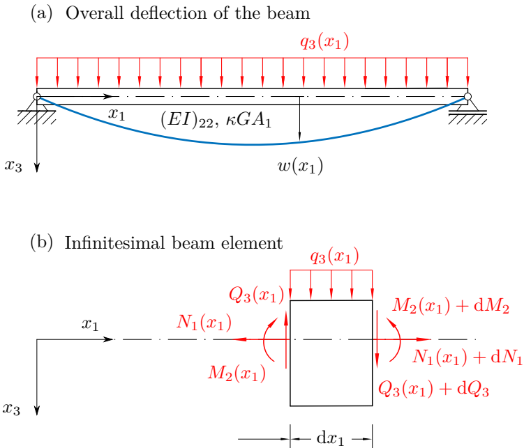
Figure 2.9: Basic deflection of a beam
