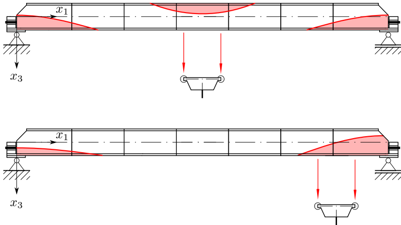
Figure 3.7: Estimated highly loaded areas during operation
