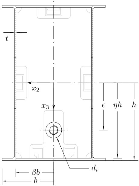
Figure 5.1: Considered cross-section in terms of optimization
