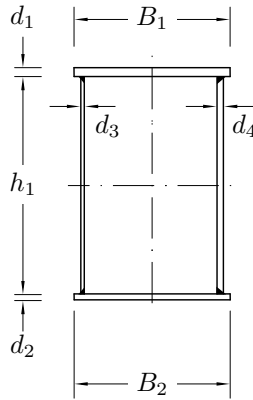
Figure 2.18: Box section and relevant design parameters considered in [8]
