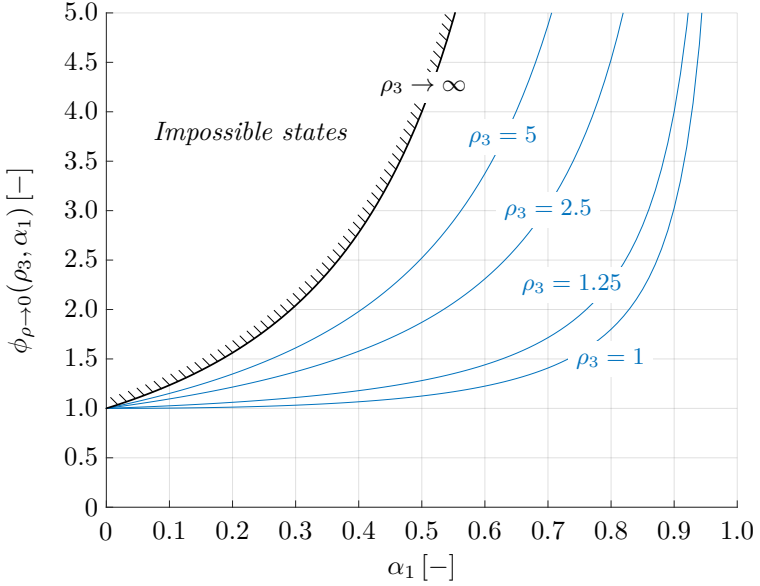
Figure 4.7: Amplification factor for different \rho_3
