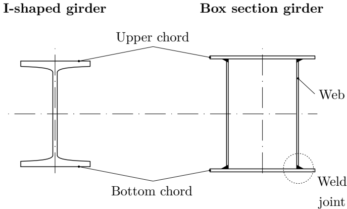
Figure 2.2: Dominating cross-sections in bridge crane systems
