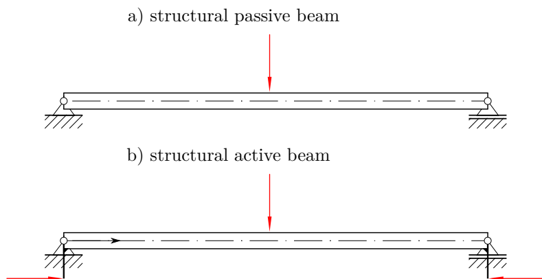
Figure 2.12: Structural passive and active beam
