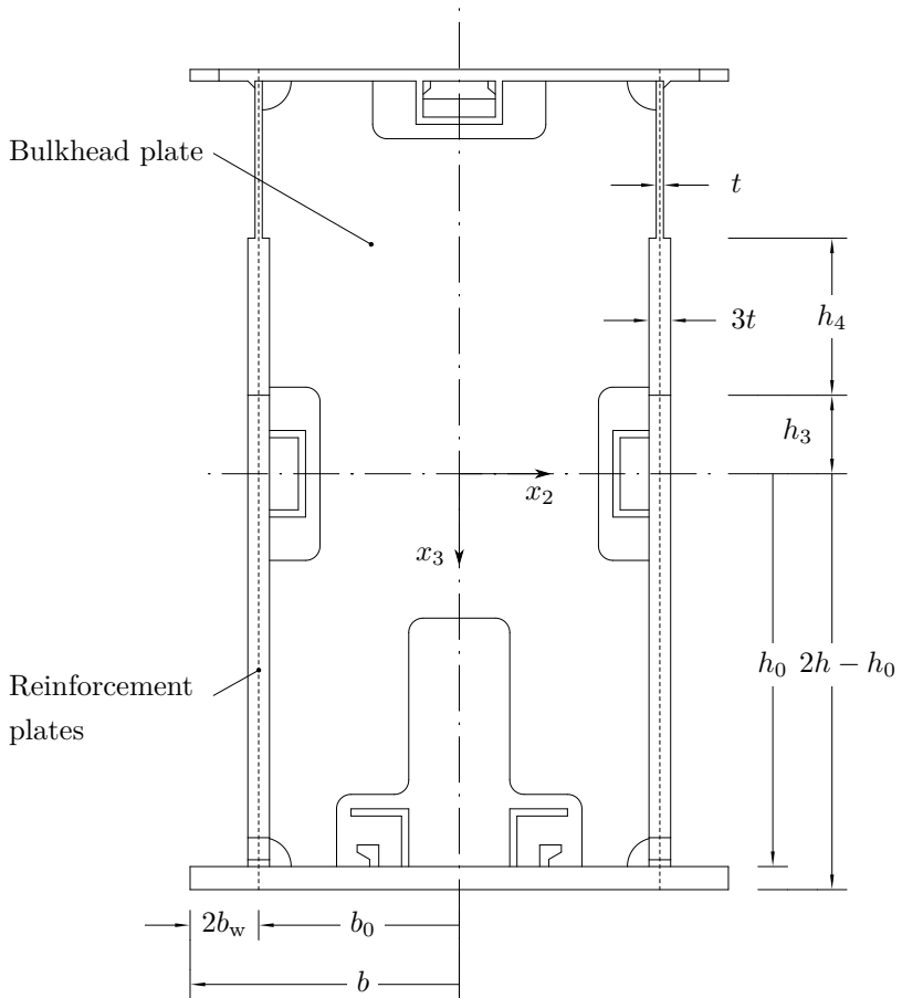
Figure 3.17: Dimensions of the preload segment (front view)
