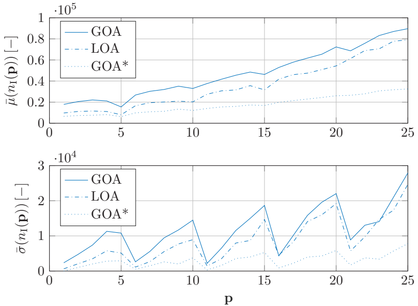
Figure 5.15: Expected values and according standard deviations in terms of necessary iterations
