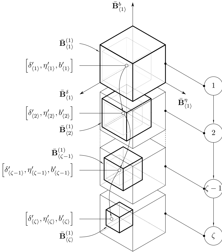
Figure 5.11: Recursive limitation of the initial search space
