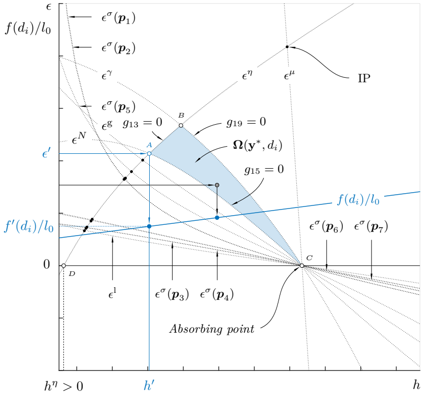
Figure 5.3: Qualitative illustration of the solution space (assuming \delta > 0 )
