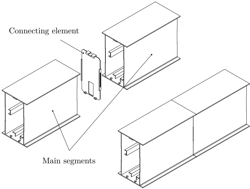
Figure 3.16: Insertion of the connecting element
