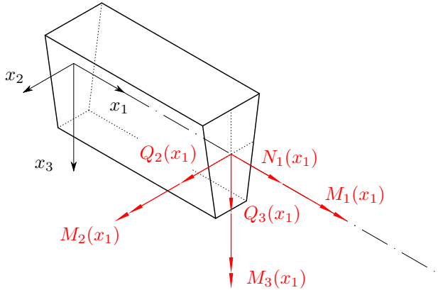
Figure 2.7: Visualization of inner forces and moments at x_1
