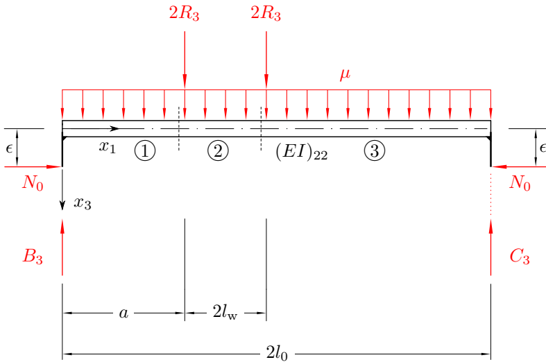
Figure 4.2: Free body diagram of the girder in terms of bending about the x_2 -axis
