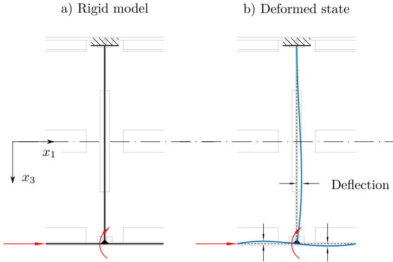
Figure 6.8: Qualitative illustration of the deformation of the connecting areas
