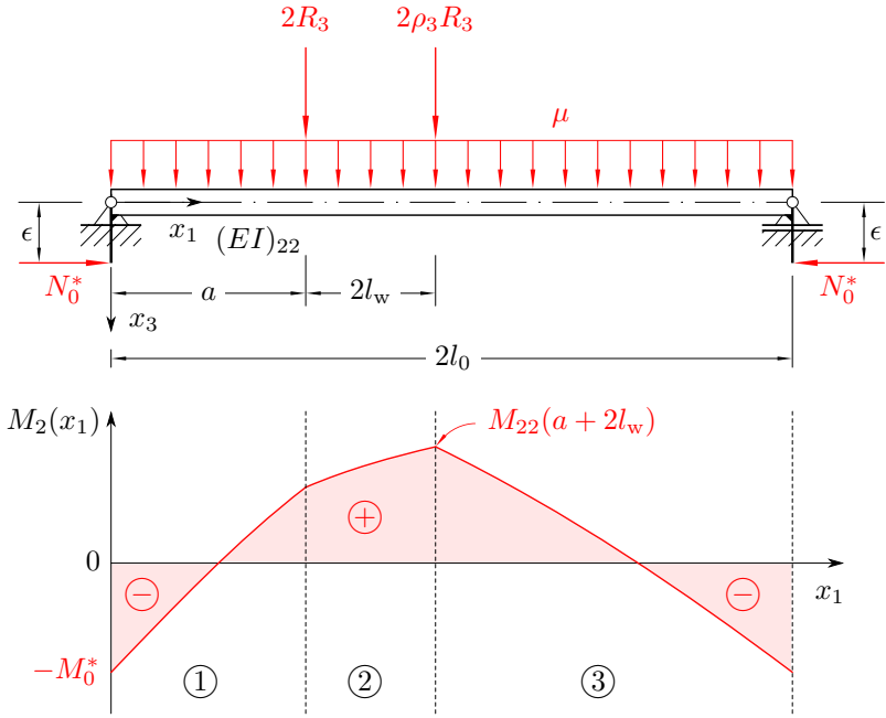
Figure 4.6: Maximum bending moment during vertical load application
