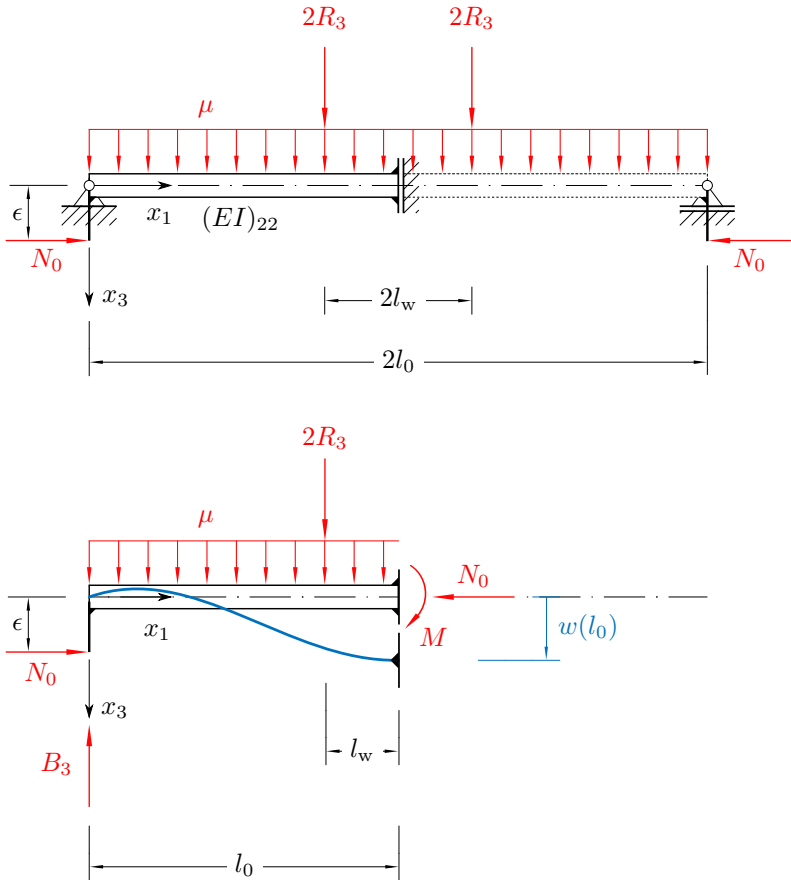
Figure 4.5: Maximum deflection during operation in x_3 -direction
