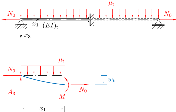
Figure 4.12: Freebody diagram of the traction mechanism
