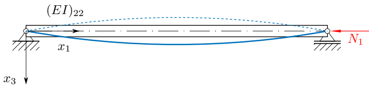
Figure 2.10: Buckling of a (slender) beam
