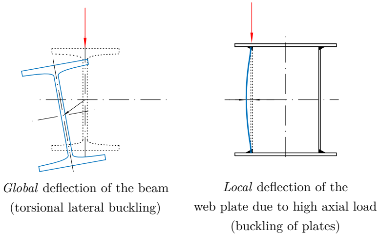
Figure 2.3: Failures of elastic stability of the considered cross-sections
