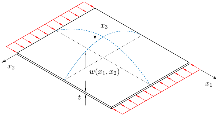
Figure 2.11: Exemplary buckling of a plate
