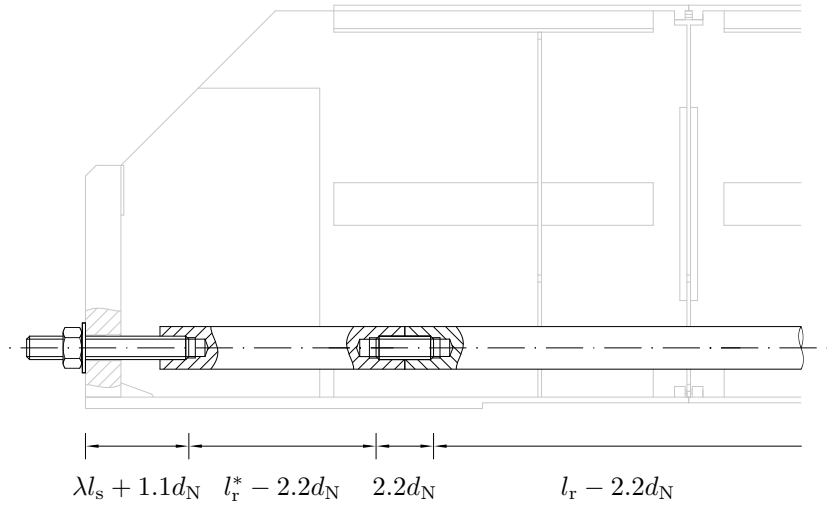
Figure 4.15: Corresponding lengths of the bolted area
