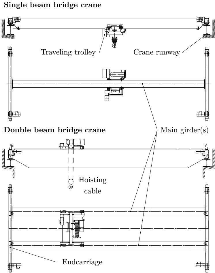
Figure 2.1: Common configurations of bridge crane systems [1, p. 8]
