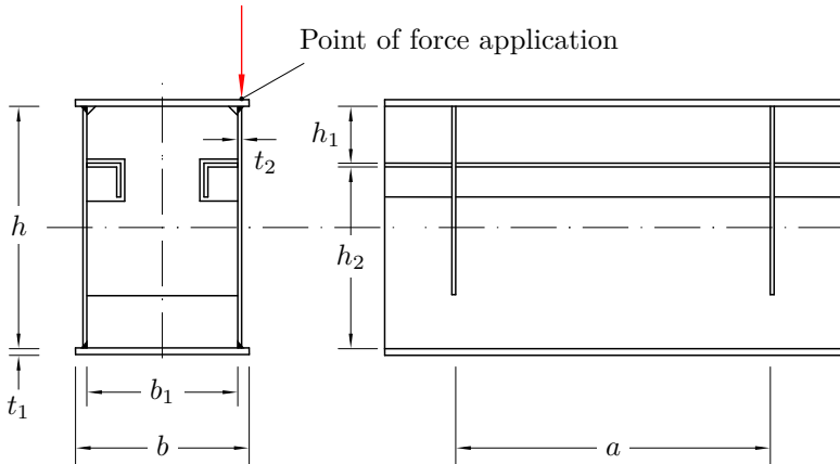
Figure 2.16: Considered box section in [6] and [7]
