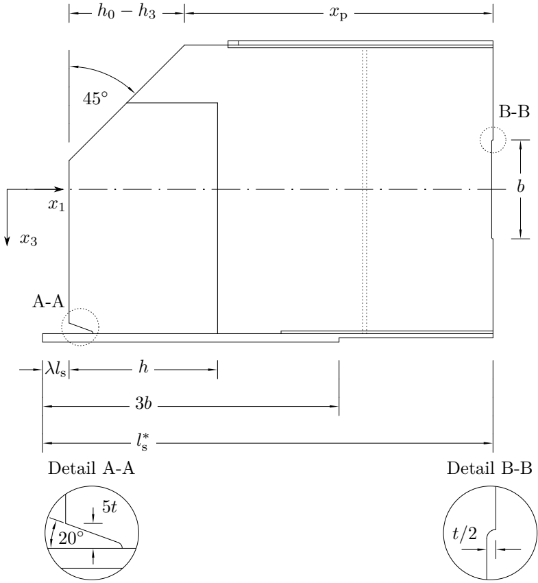
Figure 3.18: Dimensions of the preload segment (side view)
