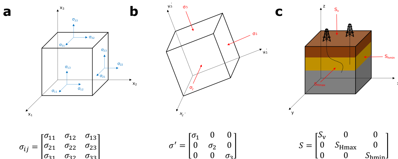
Figure 2. The nine stress tensor components define the stress state at any point and enable the determination of a stress vector on any surface within a given body (a). Based on the momentum conservation, a stress tensor has to be symmetric, which means that a coordinate system exists where shear stresses are negligible along the cube faces (b). In this, so-called, principal axis system remaining stresses are called principal stresses. With an assumption that vertical stress, S_V , is a principal stress, which is a common assumption within the Earth crust, minimum, S_{hmin} , and maximum, S_{Hmax} , horizontal stresses are also considered to be principal stresses (c). As a result, the, so-called, reduced stress tensor can be fully determined with only four components including S_{Hmax} orientation and magnitudes of S_{hmin} , S_{Hmax} , and S_V .
