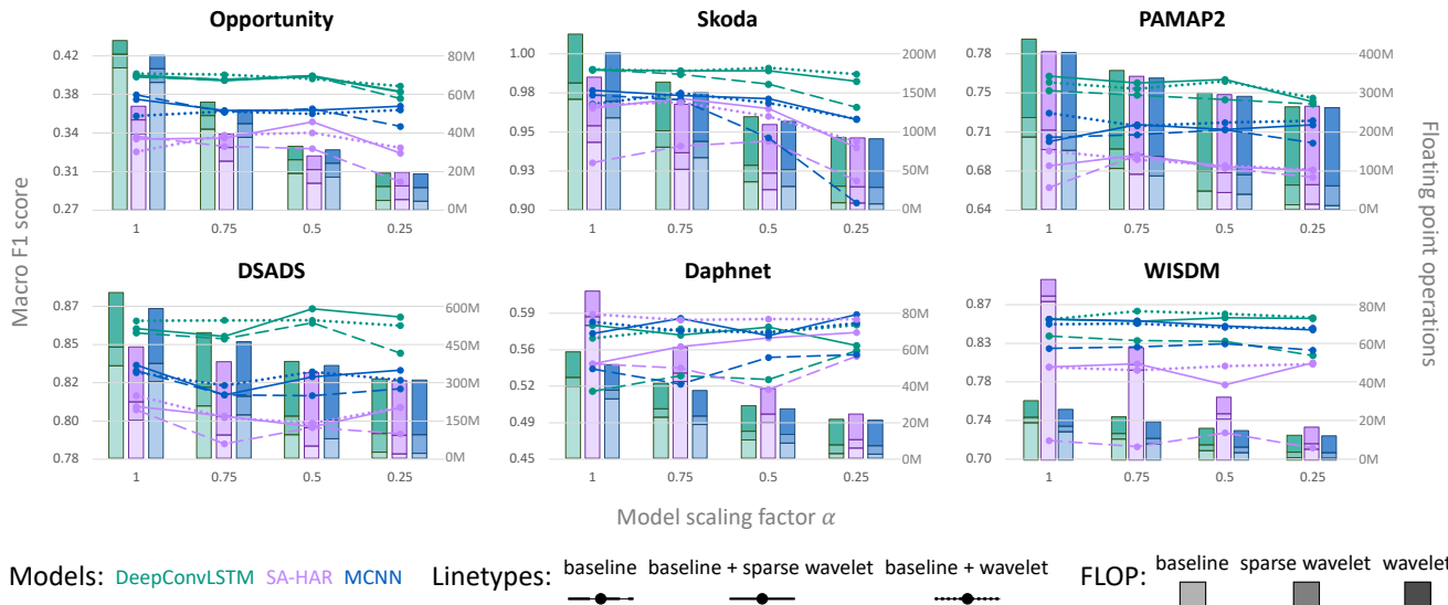
Figure 2: Result of the experiment. Different colors indicate different HAR models (green for DeepConvLSTM, purple for SA-HAR, and blue for MCNN). Different linetypes denote the macro F_1 -scores from different setups (dash lines for baselines, solid lines for learnable sparse wavelet layers , and dot lines for learnable wavelet layers without pruning ). The bars with different intensities refer to the number of floating point operations required by different setups, namely light colors for baselines, normal colors for learnable sparse wavelet layers , and dark colors show learnable wavelets without pruning .
