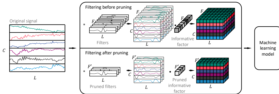
Figure 1: Pipeline of the proposed algorithm. Left: exemplary original data. Middle: the proposed learnable sparse wavelet layer. Right: a machine learning model for HAR. C = number of channels, L = length of sliding window, F = number of initially selected filters, F' = number of filters after pruning.
