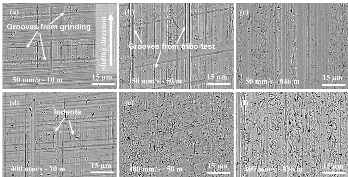
Fig. 6 SEM images of discs after constant speed experiments: (a) sliding 10 m at 50 mm/s; (b) sliding 50 m at 50 mm/s; (c) sliding 846 m at 50 mm/s; (d) sliding 10 m at 400 mm/s; (e) sliding 50 m at 400 mm/s; and (f) sliding 846 m at 400 mm/s.
