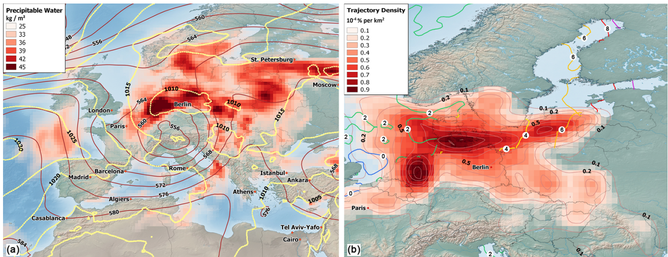
Figure 2. (a) 500 hPa geopotential (solid contours in gpm), mean sea level pressure (dashed contours in hPa), and total precipitable water (shading in kg m -2 ) on 14 July 2021 12:00 UTC (ERA5). (b) Density of air parcels (based on trajectories analysis) in the PBL (planetary boundary layer) over the entire 10 d period (shading and red contours every 0.1 % per area of 10 4 km 2 starting at 0.1 % per area of 10 4 km 2 ; ERA5); the outermost contour encloses 67 % of all air parcels. SST anomaly relative to the climatology (ERA5, 1971–2000; averaged from 8 to 15 July 2021; colored contours in K). Both backgrounds made with © Natural Earth.
