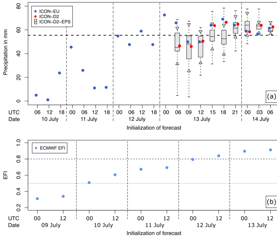
Figure 4. (a) 24 h precipitation totals over LReg (14 July 06:00 UTC to 15 July 2021 06:00 UTC) as forecasted by ICON-EU, ICON-D2, and ICON-D2-EPS for different initialization times and observed precipitation total as reference based on RADOLAN: 55.4 mm (stippled black horizontal line). For the EPS, the boxes represent the median and 25 % or 75 % percentiles, the triangles the 10 % or 90 % percentiles and the whiskers the total ensemble range. (b) Extreme forecast index (EFI) for precipitation on 14 July 2021 based on the ECMWF-EPS for different initialization times. Horizontal lines at 0.5 and 0.8 denote the limits for classification of an unusual (EFI between 0.5 and 0.8) and very unusual or extreme event (EFI greater 0.8).
