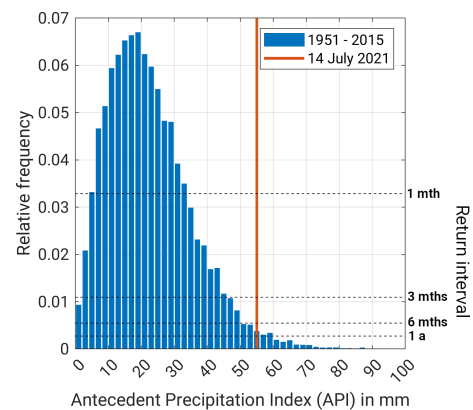
Figure 5. Frequency distribution of spatially averaged daily API values over LReg based on HYRAS (blue; 1951–2015). The red line marks the mean API on 14 July 2021 over LReg based on RADOLAN; the dashed black lines represent exemplary selected empirical return intervals.
