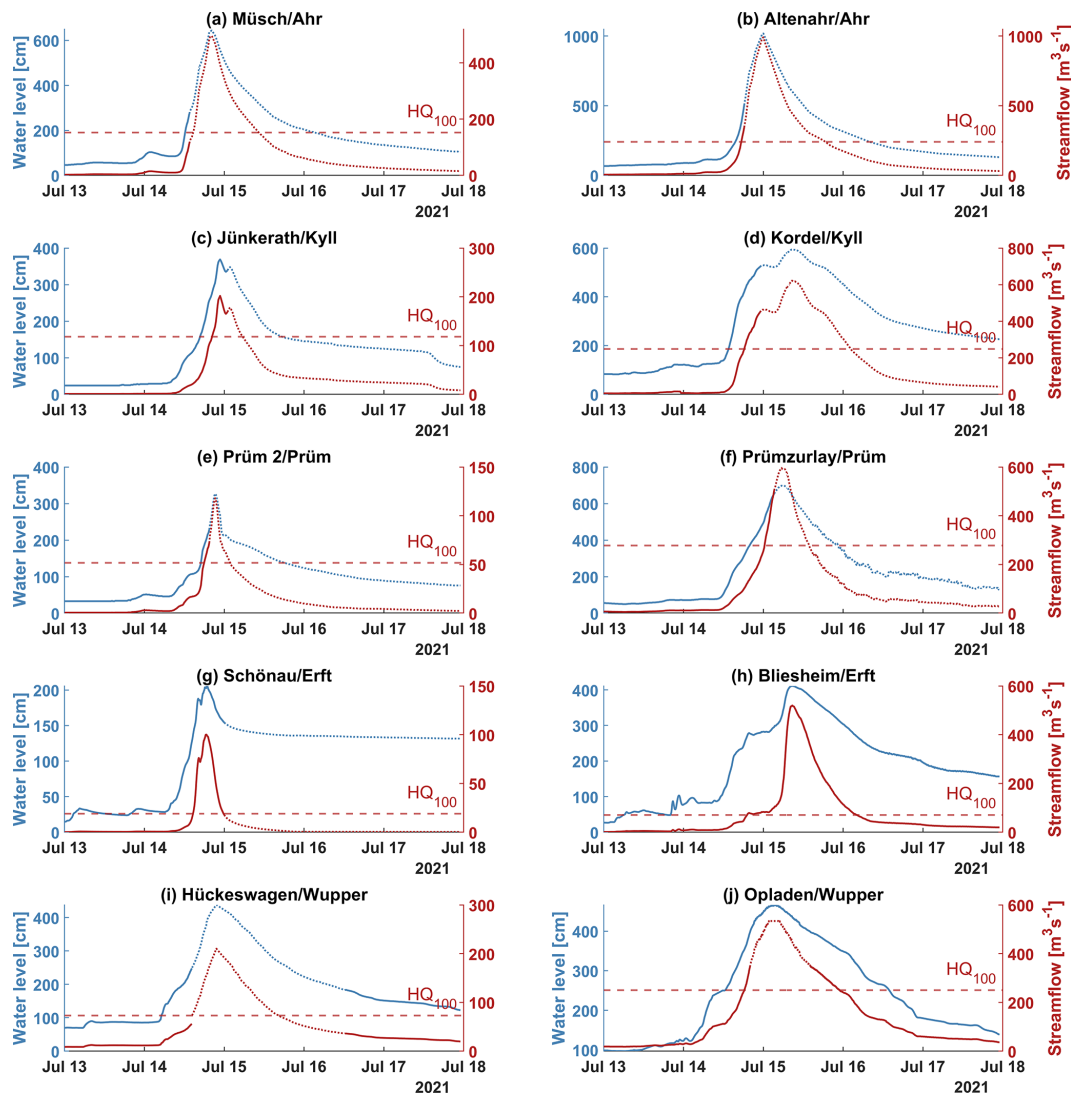
Figure 6. Time series of water level (blue) and streamflow (red) for river gauges in the Ahr, Kyll, Prüm, Erft, and Wupper river basins (13 July 00:00 UTC to 17 July 2021 23:00 UTC; resolution: 15 min). Solid lines indicate values based on in situ measurements, dashed lines indicate reconstructed values (carried out by the data-providing water authorities). Dashed horizontal lines indicate the magnitude of the statistical 100-year flood in \text{m}^3 \text{s}^{-1} . Further details about the gauges are given in Table 1.
