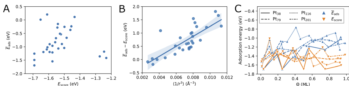
Fig. 3 Relation between the score energy E_{\text{score}} and the adsorption energy \overline{E}_{\text{ads}} (A) and between \overline{E}_{\text{ads}} - E_{\text{score}} and \langle 1/r^3 \rangle (B) for the Pt 38 nanoparticle. (C) Change of the lowest adsorption energy \overline{E}_{\text{ads}} and the lowest energy score E_{\text{score}} with oxygen coverage. The lowest coverage shown corresponds to single-oxygen adsorption for every nanoparticle. The symbols denote the data points and the lines are only added as a guide to the eye.
