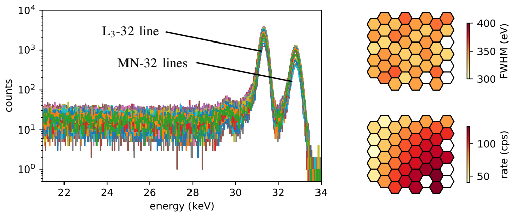
Figure 4: Energy spectra of 43 out of the 47 pixels which were read-out at the monitor spectrometer setup. The two peaks correspond to L_3 -32 and MN -32 conversion electron lines from ^{83\text{m}}\text{Kr} . The pixel maps show the energy resolution (FWHM) and the total rate of the L_3 -32 line.
