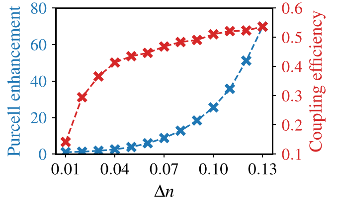
Fig. 4. Purcell enhancement and coupling efficiency for all designs at the target wavelength of 570 nm obtained from 2D effective index simulations.
