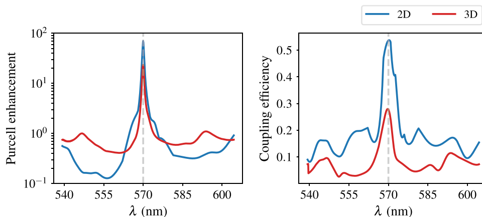
Fig. 5. Comparison of the Purcell enhancement (left) and the coupling efficiency (right) between the 2D effective index simulation and a 3D full-wave simulation. The device was optimized for an effective index contrast of \Delta n = 0.13 , which corresponds to the material platform presented in [46].
