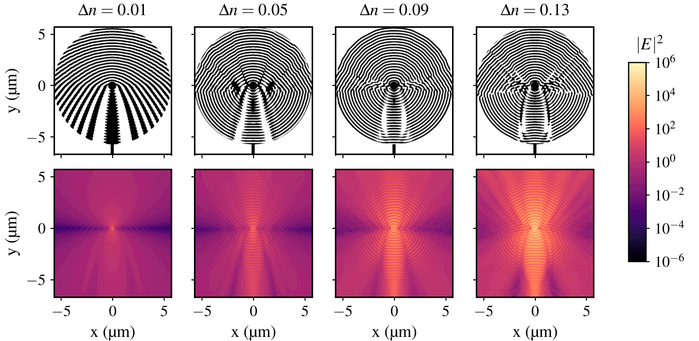
Fig. 2. Optimized device designs (top row) and corresponding electric field intensities (bottom row) in log scale at the target wavelength of 570 nm. Shown here are four selected devices designed for different effective index contrasts (columns). Note that a short length of waveguide is included for clarity but it is not part of the design region.
