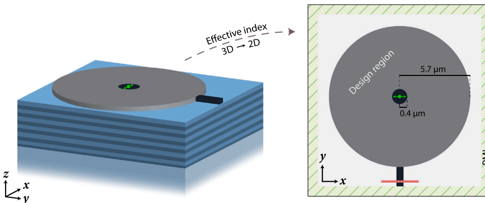
Fig. 1. Full sketch of a prototypical material platform that supports BSWs (left). A functional layer is patterned on top of a dielectric multi-layer structure sitting on a substrate in this conceptual setting. The optimization setup for the 2D effective index simulation (right) consists of a circular design region with a radius of 5.7 \mu\text{m} and a central spacer region with a radius of 0.4 \mu\text{m} and fixed material distribution. The x -polarized dipole source is embedded in the center of the spacer region. A waveguide with a width of 0.3 \mu\text{m} extends out from the lower edge of the design region. The optimization aims to maximize the power coupled from the dipole into the fundamental TM-polarized mode of the connected waveguide.
