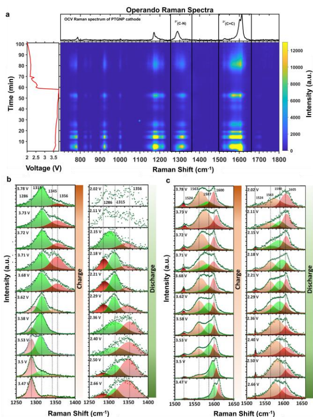
spectra in selected regions for the PTGNP cathode in the first charge/discharge cycle: (b) 1250\text{--}1400\text{ cm}^{-1} ( \nu_{(C-N)} ), (c) 1500\text{--}1650\text{ cm}^{-1} ( \nu_{(C=C)} ).
