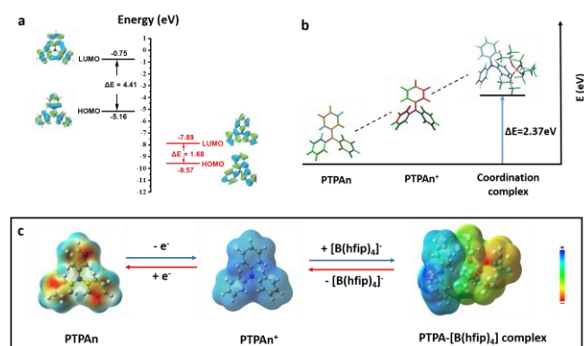
Figure 6. Density functional theory (DFT) calculations: (a) Energy level diagram of pristine PTPAn (left) and \text{PTPAn}^+ (right); (b) calculated three molecules and the corresponding formation energy changes, \Delta E (charge distribution assigned
