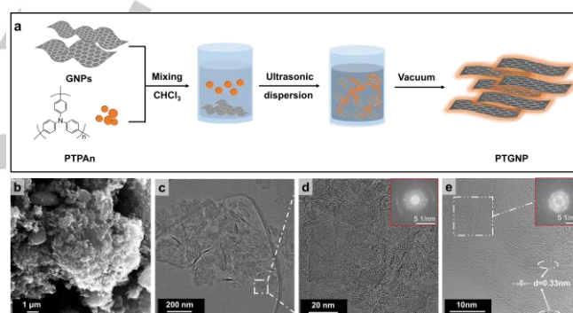
Figure 1. (a) Scheme of the PTGNP composite fabrication procedure; Morphological features of the as-prepared PTGNP composite: (b) SEM image, (c-e) TEM images (insets show the FFT patterns extracted from HRTEM images).
