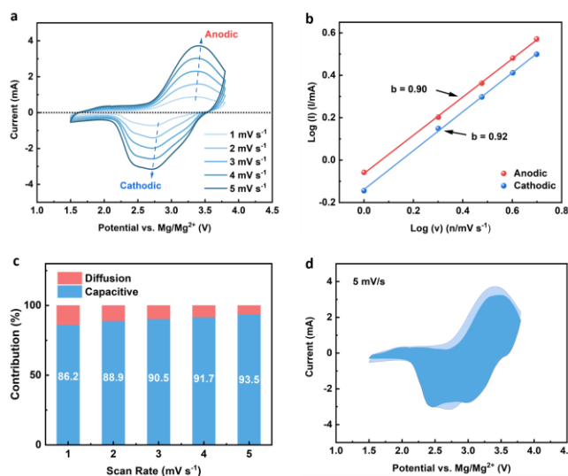
Figure 7. (a) CV curves of the Mg||PTGNP cell at various scan rates from 1 to 5 \text{ mV s}^{-1} ; (b) dependence of peak currents on scan rates; (c) diffusion and surface-controlled capacity contribution at different scan rates; (d) calculated surface-controlled (blue) and total current contribution (gray) of the PTGNP cathode at the scan rate of 5 \text{ mV s}^{-1} .
