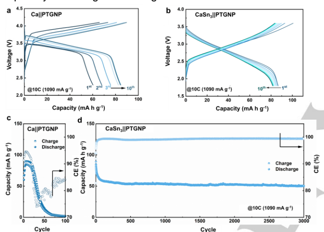
Figure 3. Electrochemical performance of the PTGNP cathode in Ca battery with 0.25 M Ca[B(hfip) 4 ] 2 /DME electrolyte. Galvanostatic voltage profiles of the composite cathode at 10C with (a) Ca-metal anode and (b) CaSn 3 -alloy anode; Cycling performance of (c) Ca||PTGNP cell and (d) CaSn 3 ||PTGNP cell at 10C (1C = 109 mA g -1 ).
