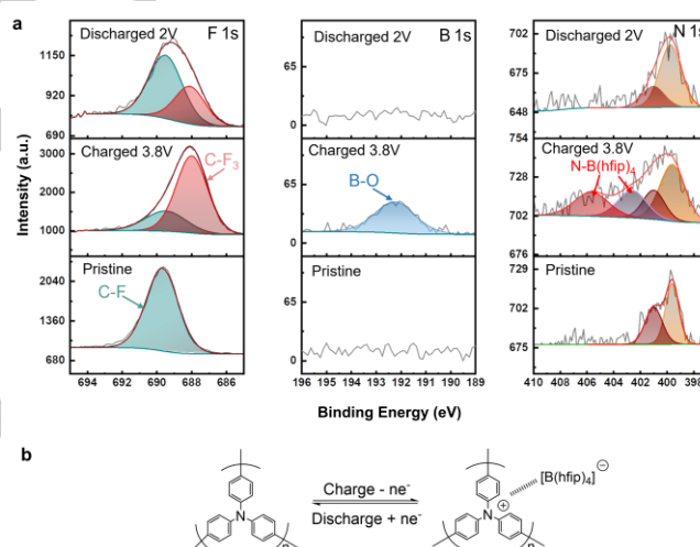
Figure 4. (a) High-resolution XPS spectra of PTGNP cathodes in different states: F 1s, B 1s, N 1s regions, (b) Schematic illustration of [B(hfip) 4 ] - anion storage mechanism based on single-electron transfer of PTPAn.
