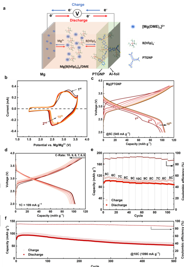
Figure 2. Electrochemical performance of the PTGNP cathode in Mg batteries
