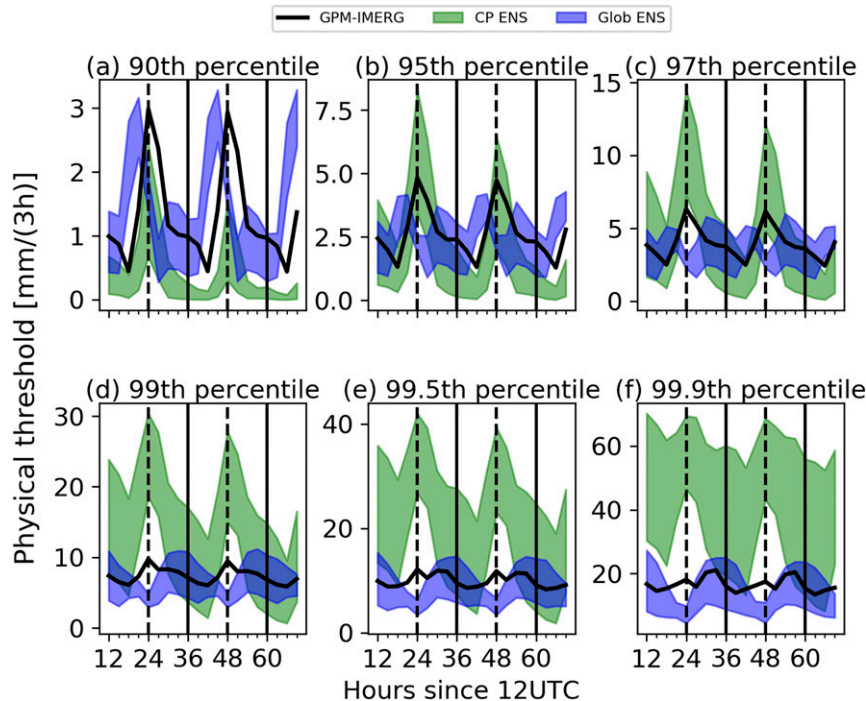
FIG. 7. Average physical thresholds [ \text{mm} (3 \text{ h})^{-1} ] over all the forecasts corresponding to (a) 90th, (b) 95th, (c) 97th, (d) 99th, (e) 99.5th, and (f) 99.9th percentile threshold as a function of the forecast hour. The physical thresholds were computed for the large domain (red dashed box in Fig. 1) for each day and for each 3-h period separately. The green and blue shadings encompass the CP and global ensembles distributions, respectively. Values on the x axis represent starting forecast hours of the 3-h accumulation periods (e.g., an x-axis value of 24 is for 3 h accumulated between 24 and 27 h).
