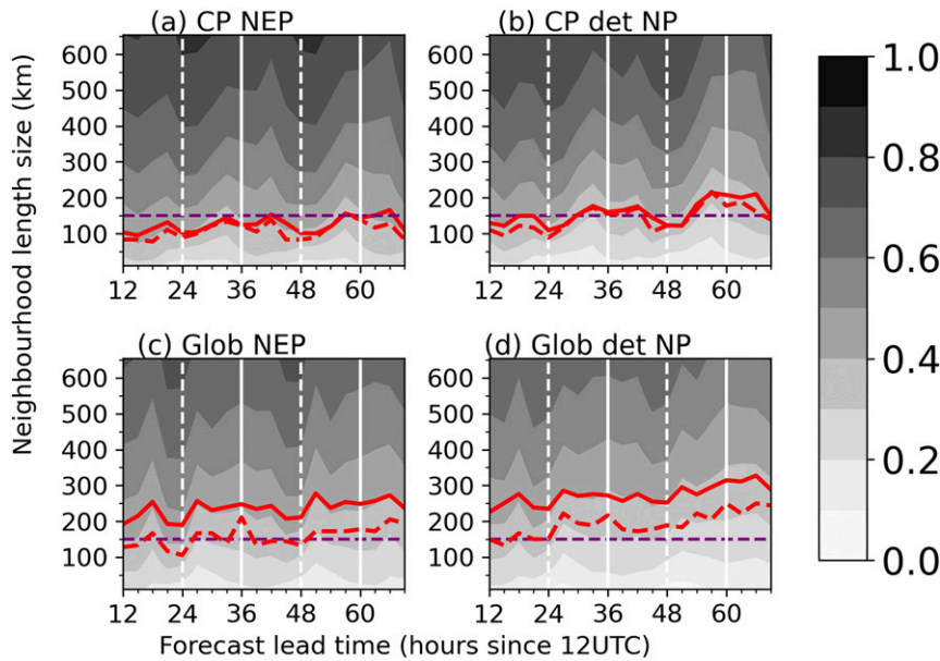
FIG. 9. Mean FSS as function of forecast hour and neighborhood length size (calculated over the large domain). The solid (dashed) red line indicates the mean (median) scale at which FSS = 0.5 over all the different forecasts. The dashed horizontal purple line indicates the 150-km scale. Values on the x axis represent starting forecast hours of the 3-h accumulation periods (e.g., an x -axis value of 24 is for 3 h accumulated between 24 and 27 h). Vertical solid (dashed) white lines indicate midday (midnight) UTC.
