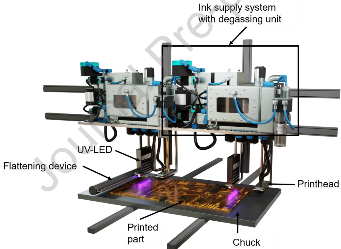
Figure 11. Schematic illustration of a material jetting printer. This multi-material printing system consists of two UV-LED sources and a flattening device for building up a high-quality 3D printed part and two printheads, each of them jetting a different material. The materials are stored and degassed in the corresponding ink supply system.
