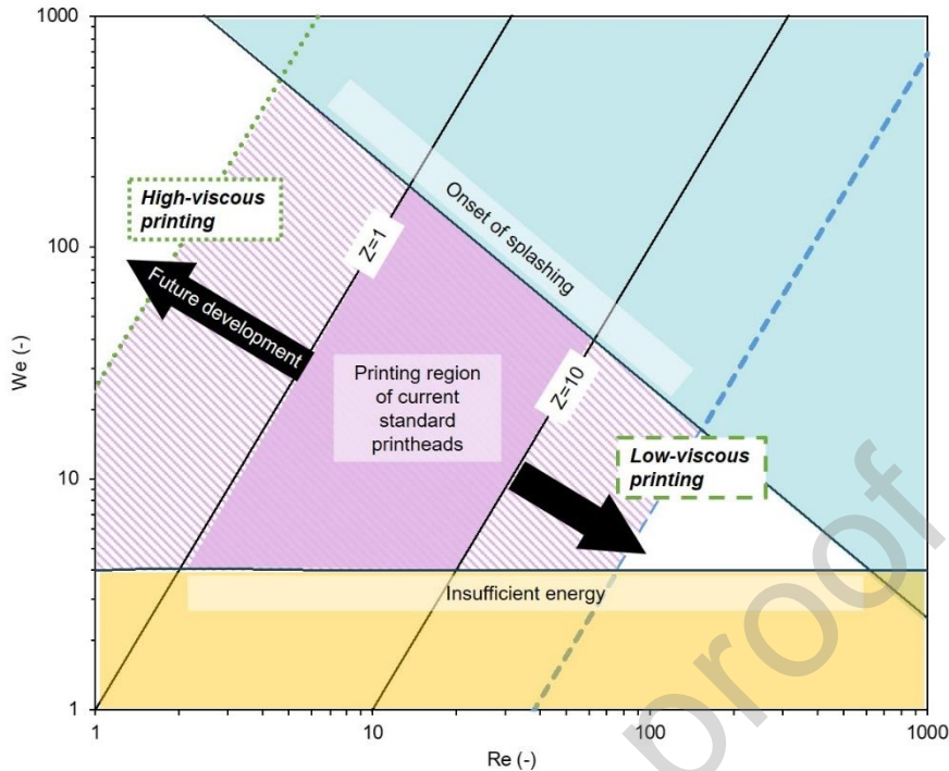
Figure 3. Printing region of current standard printheads and the future direction of development of functional inkjet printing. Adapted from illustration reported in [56].
