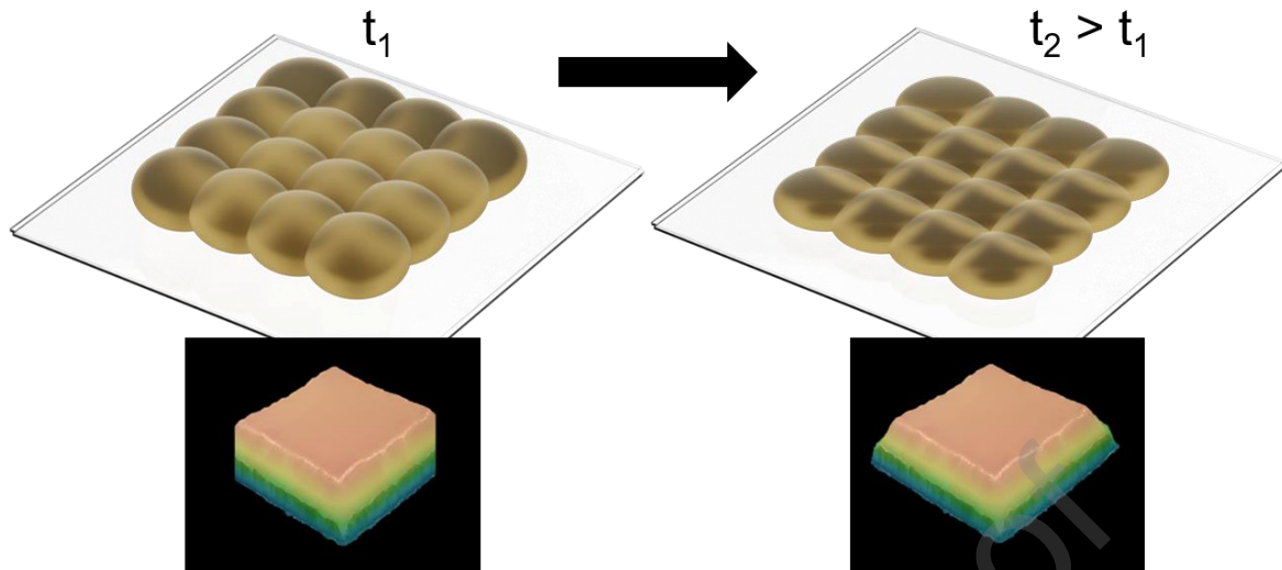
Figure 8. The effect of pinning on a layer generated by material jetting. Accuracy of a printed layer and resolution can change due to further flowing of the droplets, when not properly cured. Droplets can be prevented from further spreading by applying slight curing (pinning), however the timing and the intensity of this curing step matters.
