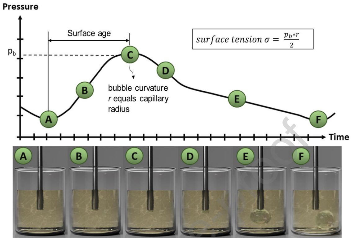
Figure 4. The course of the bubble pressure during one measurement with the maximum bubble pressure method. The surface tension is calculated based on the maximum bubble pressure reached when the bubble curvature equals the capillary radius.
