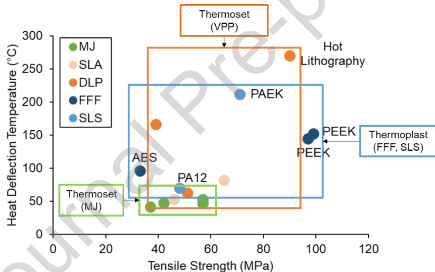
Figure 2. Mechanical and thermal properties of various plastic materials used for various additive manufacturing technologies (material jetting (MJ), stereolithography (SLA), digital light processing (DLP), fused filament fabrication (FFF) and selective laser sintering (SLS)).
