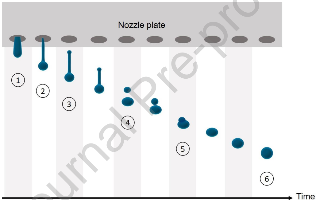
Figure 5. Droplet formation of a Newtonian fluid in DoD piezo inkjet printing. The final stable droplet is created upon the merging of the secondary droplet with the main droplet.
