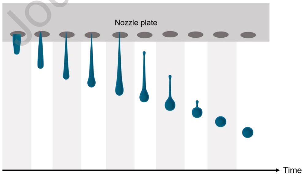
Figure 7. Droplet formation of a viscoelastic fluid in DoD piezo inkjet printing. Due to the elastic effect a separation of the tail into two droplets does not happen therefore preventing the emergence of satellite drops.
