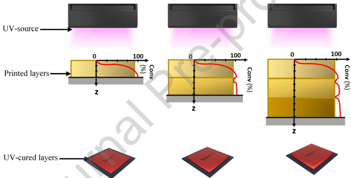
Figure 10. Oxygen inhibition and its effect on material jetting 3D parts. Each newly printed layer is subject to oxygen inhibition in the upper regime. This less-cured surface will, however, be further cured, if a subsequent layer is applied and cured so that the whole part shows an almost homogenous conversion rate with a slight dip at the height of the interface between layers (adapted from the illustrations by Taki et al. [178] and Pierrel et al. [177])
