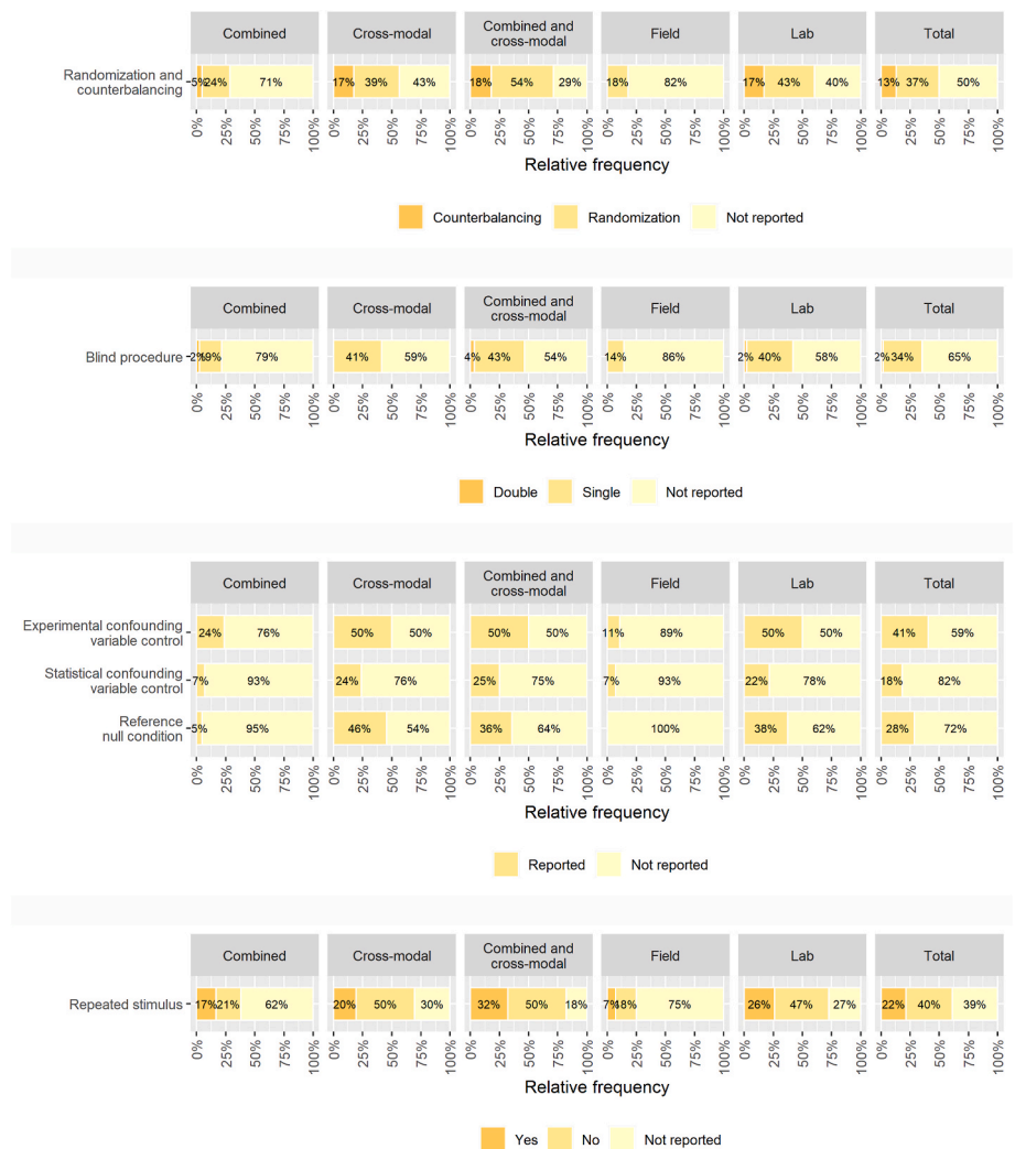
Fig. 13. Relative frequencies of information about the experimental design quality reported in the considered studies by effect type and study type.
