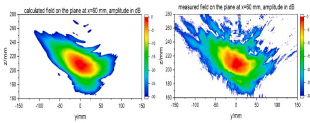
Fig. 1. Comparison between the calculated launcher output field on the left hand side and the measured field on the right hand side at 60 mm from the gyrotron axis.
