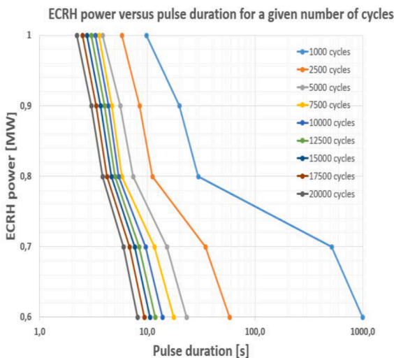
Fig. 5. Limitation of the EC launcher per line depending on cycle number, pulse duration and EC power.
