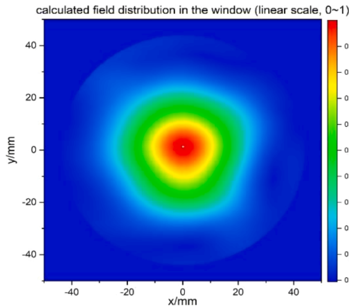
Fig. 2. Results of the field distribution at the output window with the quasi-optical converter new design for the TE 20,8 mode for the WEST gyrotron.
