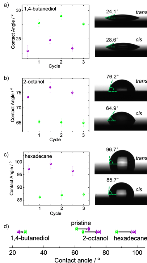
Fig. 4 The contact angle of water on the photoswitchable SURMOF loaded with (a) 1,4-butanediol, (b) 2-octanol and (c) hexadecane. The violet spheres were obtained upon violet light irradiation ( trans ) and the green spheres upon green light ( cis ). The irradiation was performed for three cycles. For each point, the contact angle measurements were repeated three times at different positions on the sample and the average values with standard deviations are shown. Photographs of the water droplet on the sample in trans (top) and cis (bottom) state are shown on the right-hand side. See also Fig. S9–S11 (ESI † ). (d) The contact angle changes of the unloaded (pristine) and loaded SURMOF sample upon irradiation with green and violet light.
