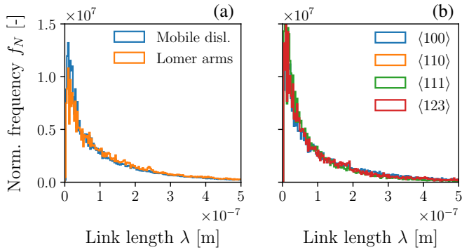
Fig. 1: Normalized link length distribution of (a) all mobile links and Lomer arms across all simulation steps of one simulation in \langle 100 \rangle orientation and (b) the normalized distribution of Lomer arms for all orientations at 0.3% total strain.
