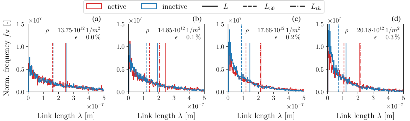
Fig. 4: Normalized frequency over link length in \langle 123 \rangle orientation for (a) 0.0%, (b) 0.1%, (c) 0.2% and (d) 0.3% total strain. The average link length L is indicated by solid, the median length L_{50} by dashed and the threshold length L_{th} by dash-dotted vertical lines.
