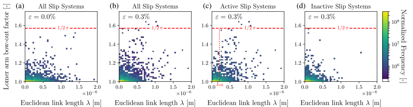
Fig. 5: Lomer arm bow-out factor versus Euclidean link length at (a) the initial state and at (b) 0.3% total strain as well as the separate evaluation of the simulation at a total strain of 0.3% for (c) active slip systems and (d) inactive slip systems for one sample with \langle 123 \rangle orientation. The color indicates the normalized frequency. The red dashed horizontal line indicates a semi-circle bow-out, which corresponds to a bow-out factor \pi/2 . The red dotted vertical line in (c) indicates the threshold length L_{th} .
