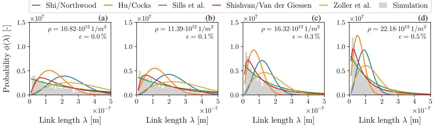
Fig. 2: Comparison of different link length distributions in \langle 100 \rangle orientation at the initial state (a) and for (b) 0.1%, (c) 0.3% and (d) 0.5% total stain with Shi/Northwood: Analytical 1 (Eq. 1), Hu/Cocks: Analytical 2 (Eq. 2), Sills et al.: Exponential (Eq. 3), Shishvan/Van der Giessen: Log-normal (Eq. 4) and Zoller et al.: Rayleigh (Eq. 5). The link length distribution of the underlying data is presented in the grey bars.
