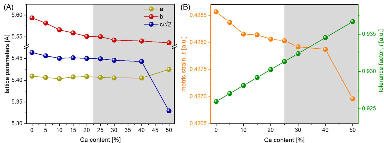
FIGURE 4 (A) Progression of the lattice parameters obtained from the Rietveld refinement and (B) comparison between tolerance factor ( t ) and metric strain ( \varepsilon ) of (\text{Gd}_{0.2}\text{La}_{0.2}\text{Nd}_{0.2}\text{Sm}_{0.2}\text{Y}_{0.2})_{1-x}\text{Ca}_x\text{FeO}_3 . The gray area indicates the compositional range where a secondary perovskite phase is observed
