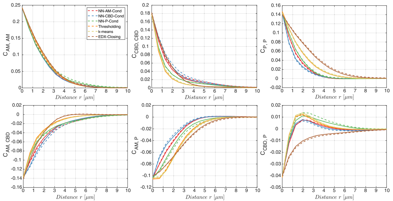
Figure 9. Top row: Centered two-point coverage probability function of active material, CBD, and pore space (from left to right). Bottom row: centered two-point coverage probability functions C_{AM, CBD} , C_{AM, P} , and C_{CBD, P} (from left to right). Note that dashed curves are used for the two-layer cathode, whereas the solid curves correspond to the single-layer cathode.
