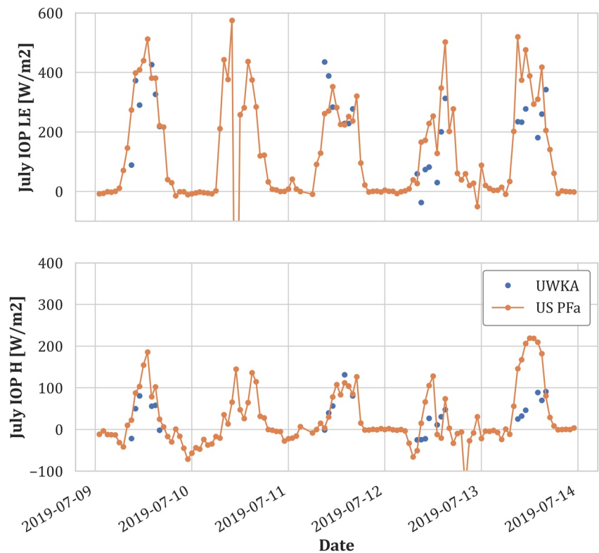
Figure 20. Hourly flux measurements from the University of Wyoming King Air (UWKA) flights and the 122 m tower measurements from the AmeriFlux regional tall tower, US Pfa, at the center of the study domain. Data shown for the July Intensive Observation Period (IOP). The UWKA flux space series was averaged to hourly data points to match the hourly time resolution of the tower measurements.
