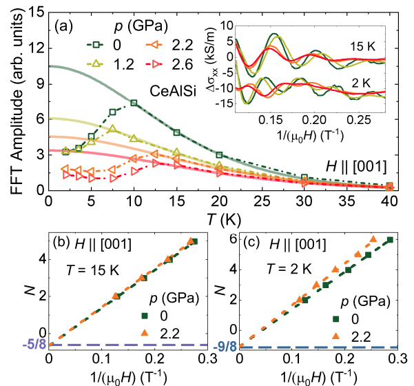
FIG. 3. (a) Fast Fourier transformation (FFT) amplitude as a function of temperature at different applied pressures. The solid lines are simulations considering the best fits using the Lifshitz-Kosevich formula. The inset shows longitudinal conductivity for H \parallel [001] after subtraction of a third order polynomial background \Delta\sigma_{xx} as a function of 1/(\mu_0 H) at 15 K (top) and 2 K (bottom) for selected pressures. The curves at 2 K were shifted by -10 kS/m for clarity. (b) and (c) Landau fan diagrams for CeAlSi at 15 and 2 K, respectively.
