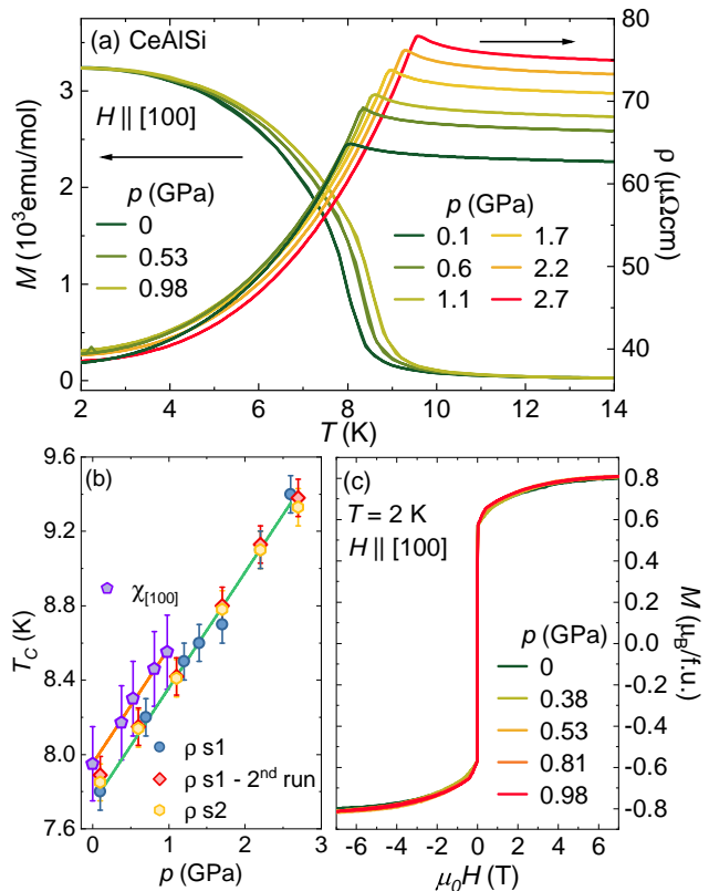
FIG. 1. (a) Magnetization ( M ) (left axis), obtained in an applied field of 50 mT along the [100] crystal axis, and electrical resistivity (right axis) as a function of temperature for selected pressures. (b) Temperature–pressure phase diagram. The solid lines are linear fits. (c) Magnetization measurements for several pressures.
