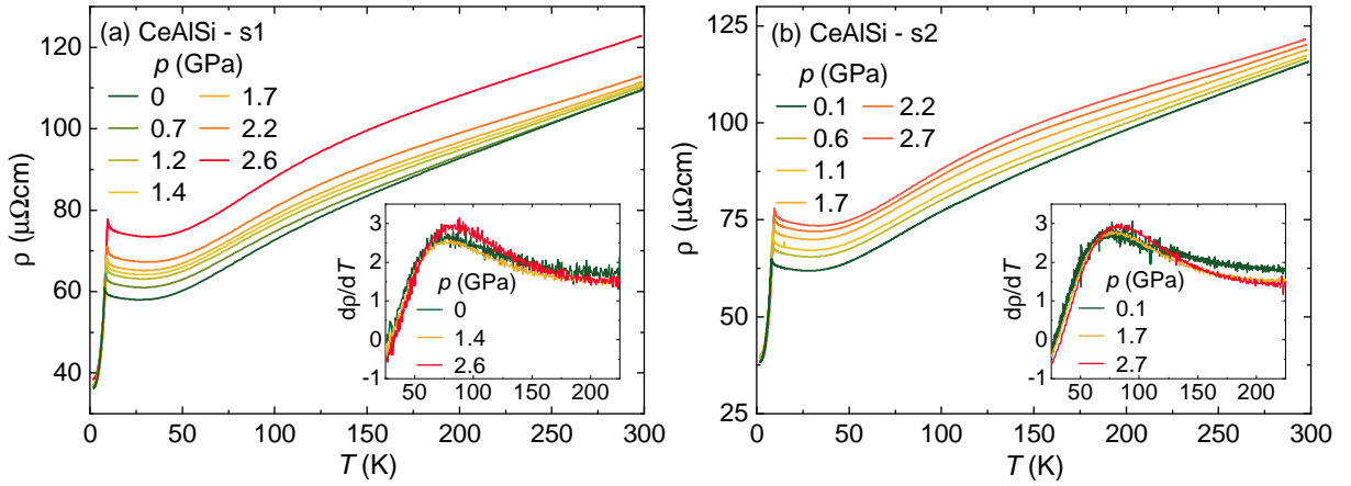
FIG. 6. (a) and (b) Electrical resistivity ( \rho ) as a function of temperature at several pressures for two different samples of CeAlSi. The insets displays a magnified view of the low-temperature range. The insets show the temperature derivative of \rho as a function of temperature at several pressures for two different samples of CeAlSi.
