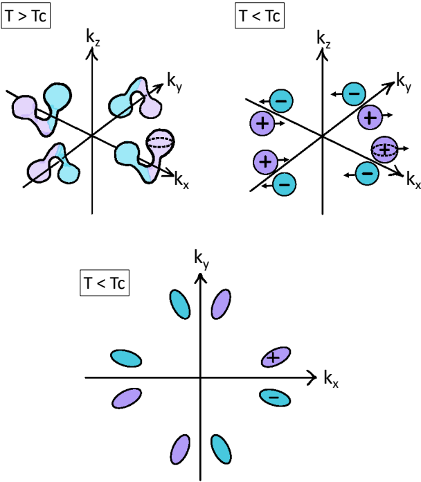
FIG. 14. Top: Illustrative example of 4 topologically trivial Fermi surface pockets for T > T_c , each enclosing a pair of Weyl points (WP) with opposite topological charge, located at momenta (K_0, \pm K_1, 0) , (-K_0, \pm K_1, 0) , (\pm K_1, K_0, 0) , (\pm K_1, -K_0, 0) . For T < T_c , the in-plane magnetization leads to a momentum space displacement of the Weyl points, leading to transition into 8 topologically nontrivial Fermi pockets. The area of certain maximal orbits (dashed lines) can remain unchanged across this transition. Bottom: Projected view of the elliptical cross sections of the topologically nontrivial Fermi surfaces for T < T_c .
