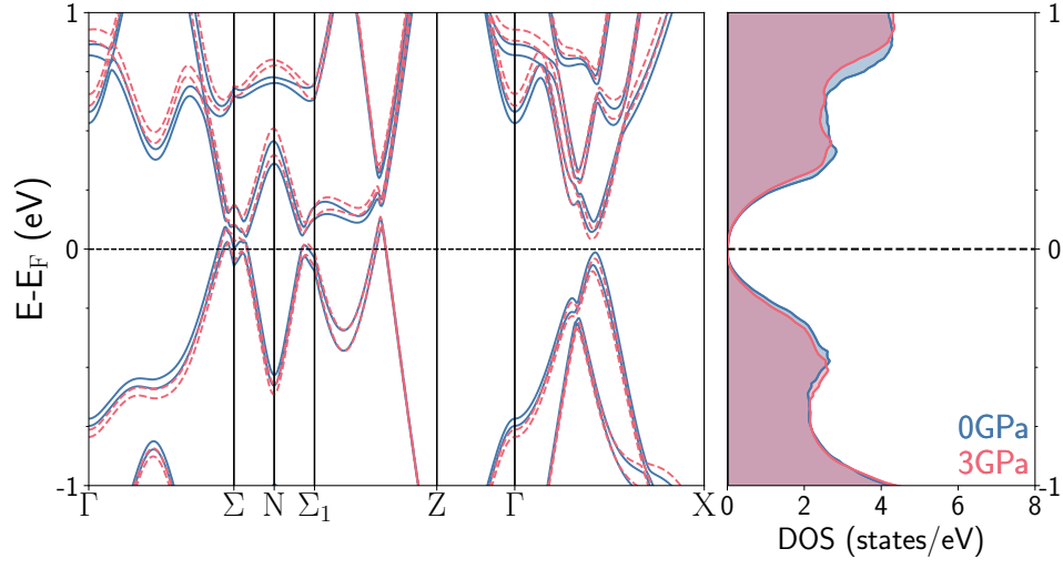
FIG. 12. Electronic bands and DOS at ambient pressure (blue) and 3 GPa (red), zoomed in the vicinity of the Fermi level.
