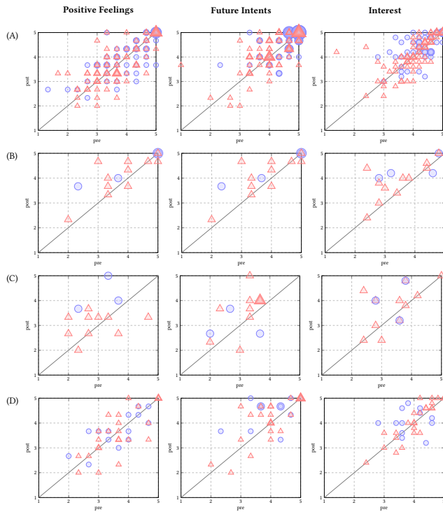
Figure 2: Scatter plots for responses in the survey and by groups (rows). The x-axis represents pre-test values and the y-axis post-test values. Red markers represent female students, and blue markers represent male students. Multiple responses with same values are indicated by multiple markers with increasing size. (A)-all, (B)-coding aversion, (C)-low initial self-efficacy, (D)-low computer affinity
