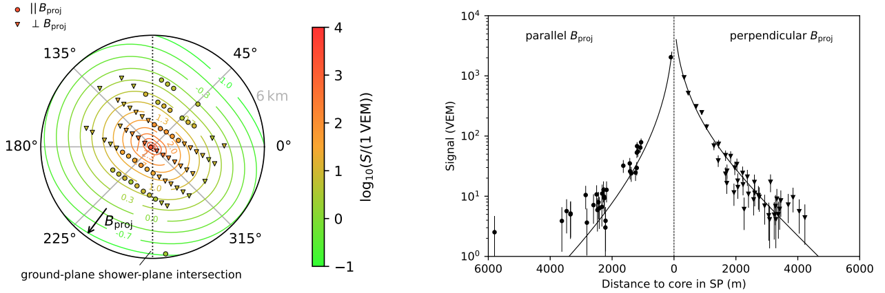
Figure 8. Left: 2D distribution of measured and expected signals in the shower plane. Station markers are colored according to the signal. The direction of the magnetic field in the shower plane ( B_{\text{proj}} ) is indicated by the black arrow. Triangular markers are stations which, seen from the position of the core, lie within \pm 45^\circ of a direction perpendicular to B_{\text{proj}} . That is, these stations are in the direction of the deflection that charged particles experience in the magnetic field. More particles therefore reach those stations (enhancing the signal) compared to stations that are at the same distance to the core but that lie along the direction of the magnetic field (circular markers). The intersection of the shower plane with the ground plane is shown by the dashed line. Right: projection of the signal distributions as a function of the distance from the shower core. The markers show the signal measured at the stations, while the curves show the expected signal. Stations in the direction parallel to the magnetic field are shown on the left, with stations in the direction perpendicular to the magnetic field on the right.
