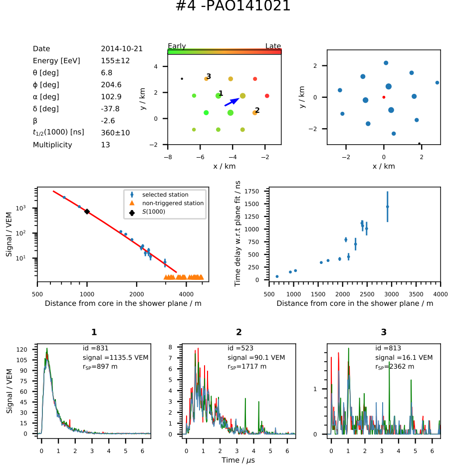
Figure 4. Features of a vertical event with a reconstructed energy of 155 EeV, (PAO141021, #4). See text for details.
