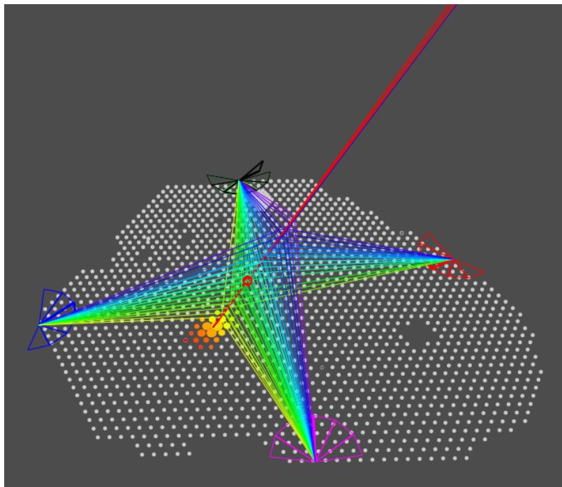
Figure 14. Three-dimensional visualization of PAO100815, #84. The lines correspond to the light rays and point to the telescopes of the fluorescence detectors. The colors of the light rays and of the SD stations represent trigger times of FD and SD PMTs, respectively.
