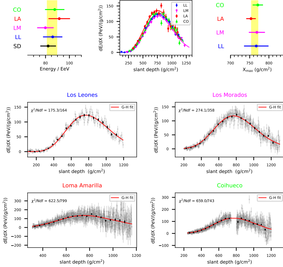
Figure 12. Reconstructed parameters of PAO100815, #84. FD stations used in the reconstruction are distinguished by different colors. The red lines correspond to fits to the profiles of the energy deposition using the universal shower profile function (Section 3.2.4). The yellow bands are centered on the combined weighted average of the measurements of X_{\text{max}} and the energy at the FD sites. The widths of the bands correspond to the statistical uncertainties of combinations. The uncertainty in the SD energy is 8% (Section 3.3).
