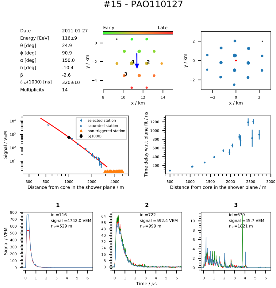
Figure 6. Features of an event, (PAO110127, #15) in which one of the WCDs is saturated. See text for details.
