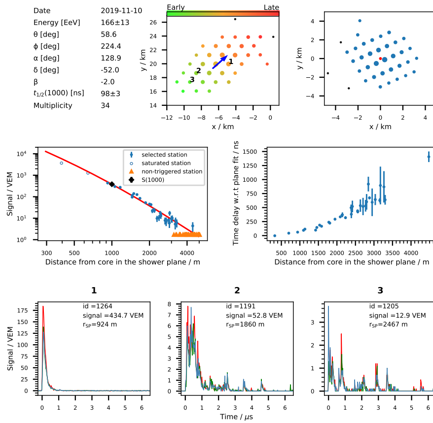
Figure 3. Features of the most energetic event, (PAO191110, #1) recorded with the Surface Detector of the Pierre Auger Observatory. See text for details.
