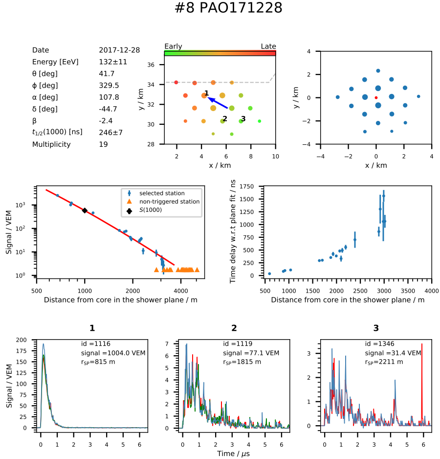
Figure 5. Features of an event, (PAO171228, #8) recorded with WCDs located at one of the boundaries of the Surface Detector. See text for details. Note that in detector #1346 only two of the three photomultipliers were operational. Reality dictates that it is impossible to keep all three photomultipliers operational 100% of the time. Failures of two, or even all three, photomultipliers inevitably occur. Typically 98% of all stations are active at any time, sending triggers at 20 Hz to the central station (Section 3.1).
