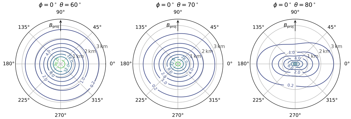
Figure 2. Parameterized densities of muons for a 10EeV proton shower at zenith angles of 60^\circ , 70^\circ and 80^\circ arriving from azimuth, \phi = 0^\circ . Radial units are in kilometers. The coordinate system is defined in the plane perpendicular to the shower direction with the y-axis parallel to the projection of the Earth’s magnetic field, B_{\text{proj}} , on that plane. The magnitudes of the muon densities are indicated (32, 16, 8... per \text{m}^2 ).
