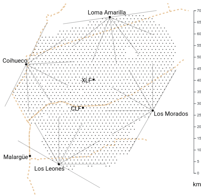
Figure 1. The layout of the Pierre Auger Observatory covering 3000 km 2 . Each small dot corresponds to a water-Cherenkov detector. Fluorescence detectors are located at Los Leones (LL), Coihueco (CO), Loma Amarilla (LA) and Los Morados (LM). The 30° azimuthal fields of view of the six telescopes at each site are shown by the radial lines emanating from them: the vertical reach of the telescopes extends to an elevation of 28.6°. Data are transmitted to the central laboratory, located at a campus in Malargüe, using a purpose-built communication network. The dashed lines show roads. Gaps in the layout of the array arise due to difficulties with landowners. Steerable lasers (see text) are located at the positions CLF and XLF.
