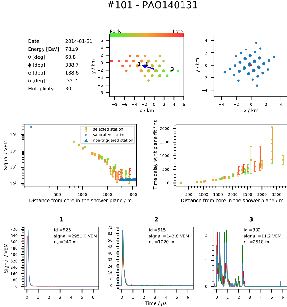
Figure 15. The parameters reconstructed using the data from the WCDs for event, PAO140131, #101.
