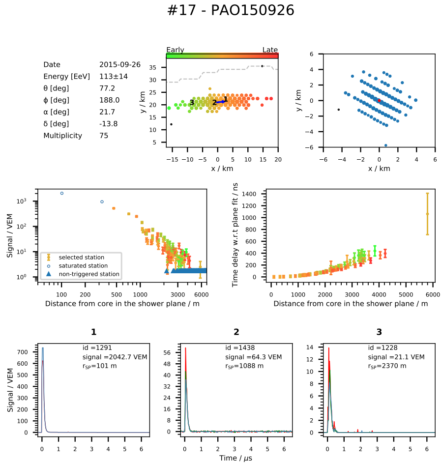
Figure 7. Features of the most energetic event, (PAO150926, #17) belonging to the set of inclined showers ( \theta > 60^\circ ). See text for details.
