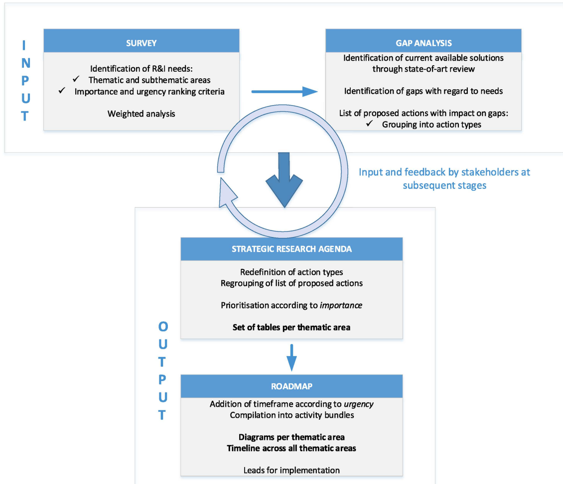
Fig. 5. SHARE methodology.
