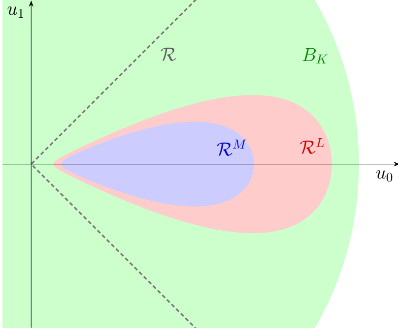
Figure 1: The sets used in the proof of Lemma 2. For this figure, we consider the M_1 case in slab geometry: V = [-1, 1] , \mathbf{m}(v) = (1, v) . In this case, the realizable set is given by \mathcal{R} = \{(u_0, u_1) : |u_1| < u_0\} , and we used M = 1 , L = 1.3 , and K = 8 .
