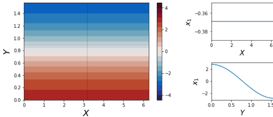
Figure A3. The background state in the Croomelin 1904 formulation of the CdV79 system. It is zonally symmetric and represents the impact of the meridional temperature gradient. Again, sub-panels show cross sections across the domain, following the dotted black lines.
