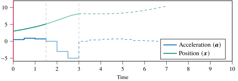
(a) Planning performed at t_0 = 0.0 . Acceleration at t \in [t_0, t_{\text{pin}}] is pinned, and t \in (t_{\text{pin}}, 2t_{\text{pin}}] will be kept fixed during the next replanning.
