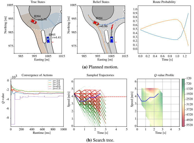
Figure 7.12: Evolution of the scenario after 1.3 s, for v_{\text{des, ego}} = 4.0 m/s and v_{\text{des, } k} = 10.0 m/s.
