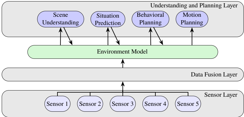
Figure 1.3: Illustration of an autonomous vehicle system architecture [Taş+17].
