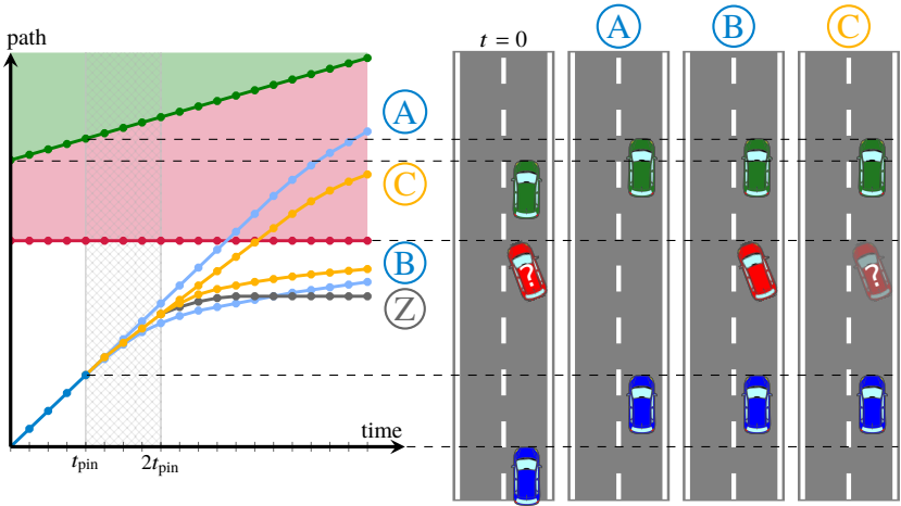
Figure 5.1: A situation where the existence of the red vehicle is unclear. The left-hand side shows the corresponding path–time diagram. Conventional motion planners choose between maneuvers A and B. With decision-theoretic MPC, a neutral maneuver C, the profile of which depends on the existence probability of the red vehicle, is planned. The hatched time interval on the path-time diagram will be driven next.
