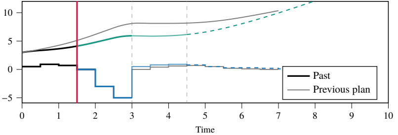
(b) Replanning performed at t_0 = 1.5 . The gray line depicts the state profile under the previous control profile, whereas the black one depicts the driven motion. The offset between them depicts the modeling errors.
