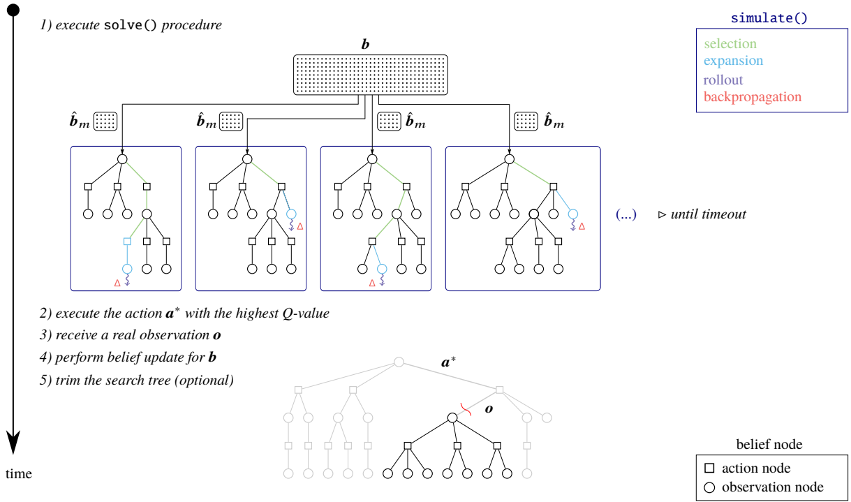
Figure 6.2: Operation steps of IPFT. In the solve() procedure the algorithm iteratively samples a weighted particle set \hat{\mathbf{b}}_m and calls the simulate() procedure until timeout. Subsequently, it executes the steps numbered from 2) to 5), where the latter is optional and by trimming the search tree from the red wavy line, it prevents building a search tree from scratch.
