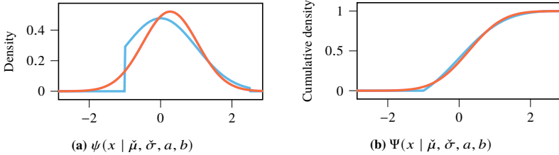
Figure A.1: Truncated univariate Gaussian distribution with \tilde{\mu} = 0.00 , \tilde{\sigma} = 1.00 bounded into the interval -1.0 \leq x \leq 2.5 . It is internally mapped into \mathcal{N}(0.27, 0.77) .
