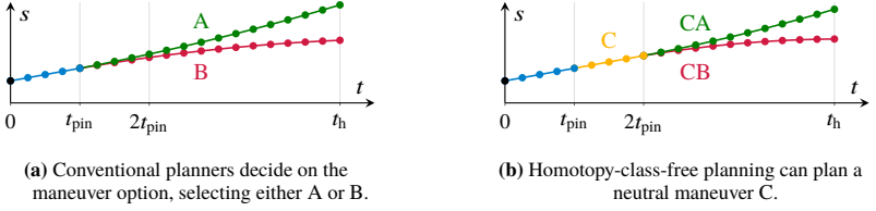
Figure 4.5: Motion profile comparison of homotopy-class-bound and homotopy-class-free planning on path-time diagram. s_{B,i} \leq s_{C,i} \leq s_{A,i} , \forall i \in \{n_{pin} + 1, \dots, 2n_{pin}\} .
