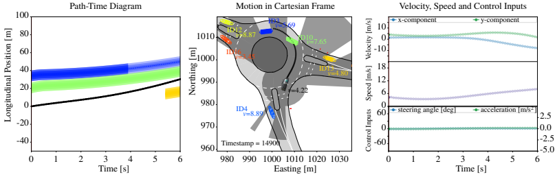
Figure 7.8: Smooth planning with decision-theoretic MPCC. The ego vehicle is depicted in black. Vehicles in the environment model \mathcal{V}_{\mathcal{E}} , i.e., inside the visible field, in gray, are represented with their position uncertainty and a semi-transparent rectangle centered at their mean position. The rectangles are opaque for vehicles in the scene model \mathcal{V}_{\mathcal{S}} .
