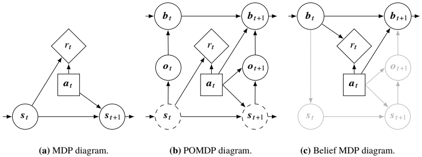
Figure 6.1: Probabilistic graphical models of an MDP, a POMDP, and a belief MDP.
