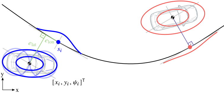
Figure 5.2: Illustration of the MPCC formulation together with uncertainty projection.
