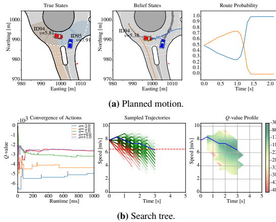
Figure A.3: Results after 2.1 s for v_{des, ego} = 6.55 \text{ m/s} and v_{des, k} = 5.0 \text{ m/s} .
