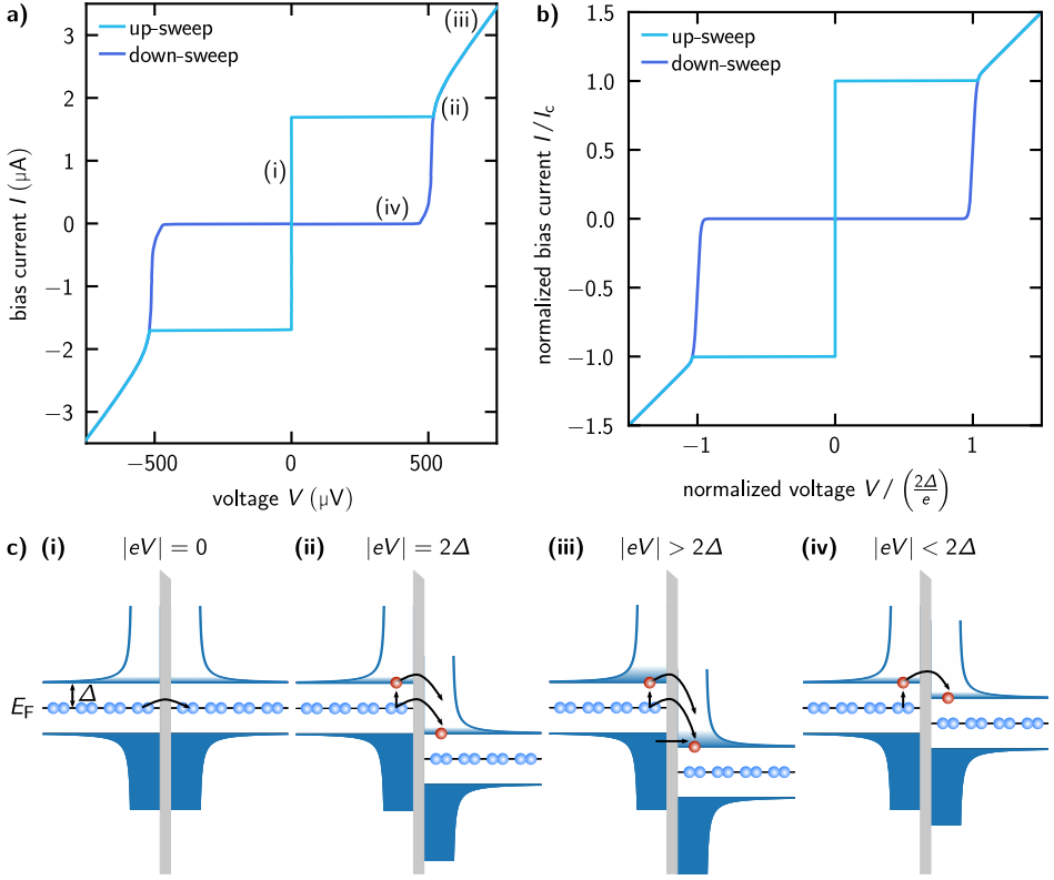
Figure 2.11: IV-characteristic of a current biased and underdamped Josephson junction. a) IVC of a 110 \mu\text{m} \times 5 \mu\text{m} wide underdamped Josephson junction with electrodes made from \text{AlO}_x and pure Al measured at T \approx 20 \text{ mK} . b) The simulated IVC by means of the nRCSJ model in eq (2.69) exhibits an almost vertical slope (conductance) around the gap voltage at the down-sweep between the critical and the retrapping current. c) Various conductance on different branches of a real junction's IVC within the scope of band diagrams of two weak link superconductors [Poo+14]. (i) Below the critical current, the junction remains in the zero-voltage state, where superconducting (s) Cooper pairs may tunnel coherently and without any dissipation ( s \rightarrow s ). (ii) At the critical current, the junction jumps to the gap voltage 2\Delta/e , while Cooper pairs are broken in two quasiparticles (q) each. These fermions may tunnel through the barrier dissipatively with a nonlinear resistance due to the quasiparticles' increased density of states ( s \rightarrow q ). (iii) Far above the critical current, and thus way beyond the gap voltage, lots of normal free electrons (n) tunnel yielding the ohmic normal state resistance ( n \rightarrow n ). When decreasing the bias below the critical current underdamped junctions remain in the running state at the gap voltage down to a retrapping current (analog to (ii) ). (iv) Close to the retrapping current, and thus below the gap voltage, a small number of not yet recondensed quasiparticles may tunnel with dissipation ( q \rightarrow q ), which is often referred to as Stewart-McCumber branch.
