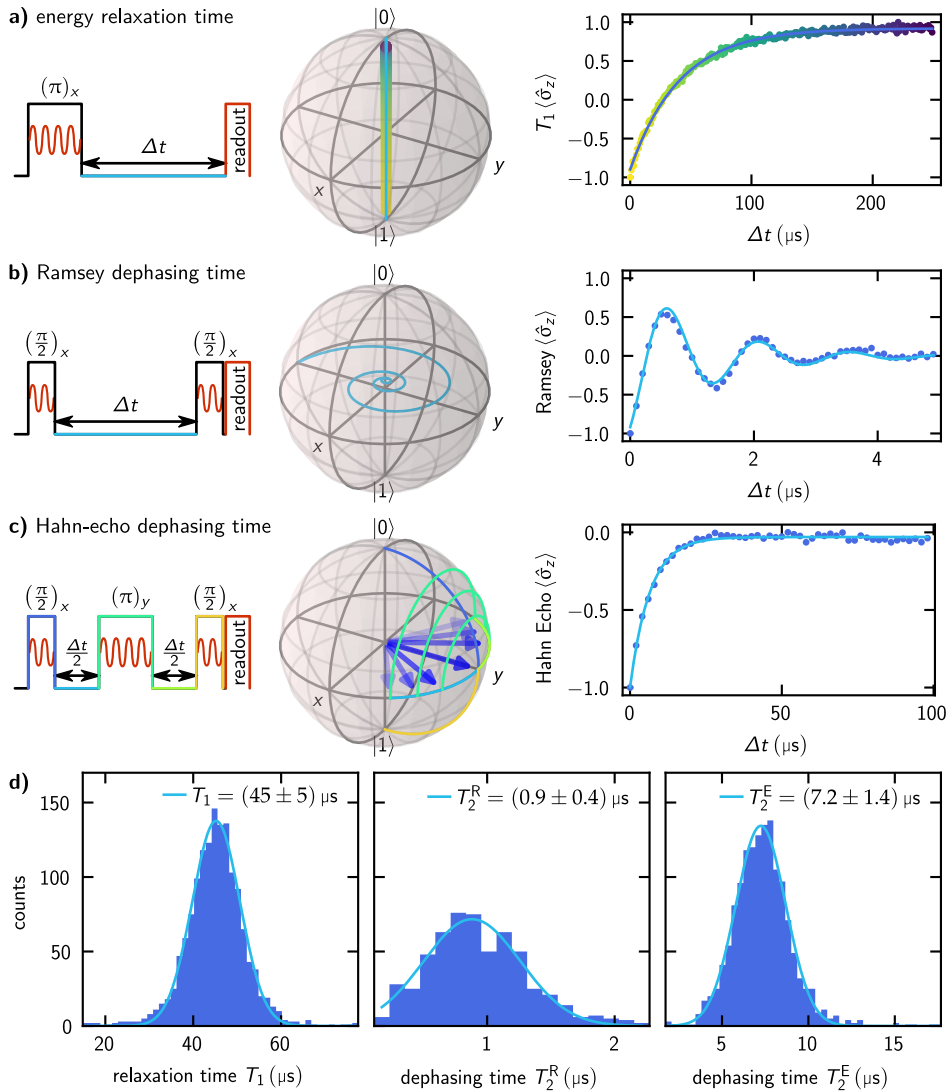
Figure 6.5: Energy relaxing and dephasing time measurements on a Josephson vortex qubit.
