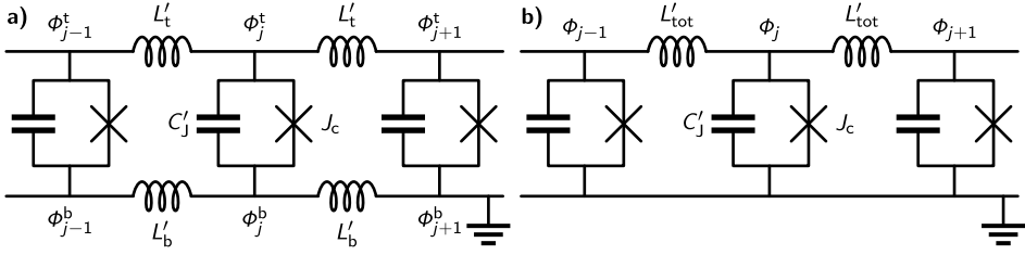
Figure A.1: Equivalent circuit of long Josephson junctions. a) A long junctions is modeled by lumped element junctions that are connected by inductive top and bottom electrodes, whose inductance may differ. b) In this circuit, the two inductance are equivalent to only one effective inductance in one electrode.
