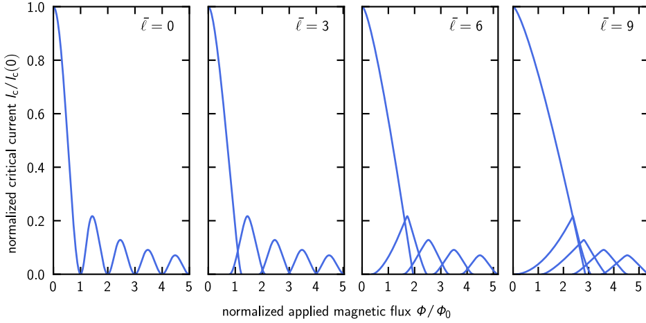
Figure 2.14: Magnetic diffraction pattern of the critical current for different junction lengths.
