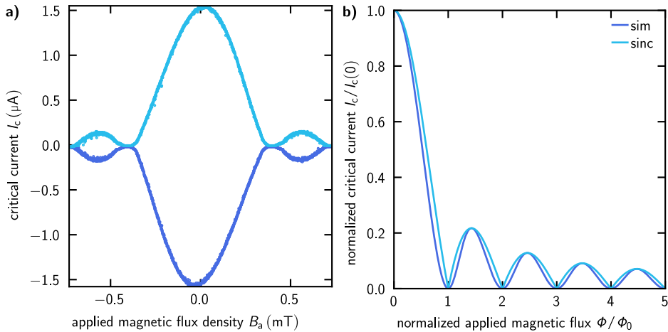
Figure 2.13: Fraunhofer-like magnetic diffraction pattern of a short junction's critical current. a) Measured diffraction pattern of a 80\ \mu\text{m} \times 5\ \mu\text{m} junction in inline geometry with electrodes made from high-kinetic inductance \text{AlO}_x and pure aluminum. The slight asymmetry arises because of the inhomogeneous bias current distribution in the inline bias scheme in combination with different inductances in the bottom and top electrode [Sch70; BJV75; Mon+13]. These experimental data resemble b) the analytically calculated sinc-shaped diffraction Fraunhofer pattern, which, however, features dissonantly sharp turns at integer multiples of \Phi_0 . More advanced simulations [PRS91], assuming a normalized junction length \ell/\lambda_J = 0.3 , cover this detail splendidly.
