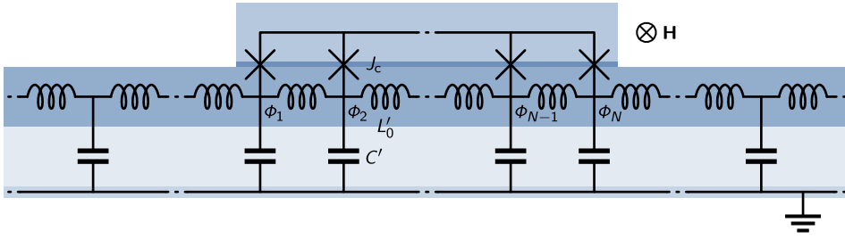
Figure 5.4: Schematic circuit of a galvanically coupled long junction to a microwave resonator. The microstrip structure forms an open-end LC transmission line with the strip's geometric and kinetic inductance L_0 = L'_0 l and the capacitance against the backside ground electrode C = C'l . The resonator's conductor is shared as the long junction's bottom electrode, which is weakly coupled with the top electrode by an insulating tunnel barrier with the critical current I_c = J_c \ell . Since the bottom electrode's kinetically dominated inductance exceeds the purely geometric inductance of the top electrode by orders of magnitude, this is dropped in the schematic circuit.
