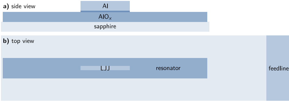
Figure 5.1: Schematic sample design for long junctions embedded in a microwave resonator. a) A open-end microstrip LC transmission line forms a distributed \lambda/2 resonator. The center part of this high-kinetic inductance resonator serves as bottom electrode of a high-impedance long Josephson junction, whose top electrode is made from a pure aluminum. b) The resonator is coupled capacitively to a microwave feedline in notch type configuration.
