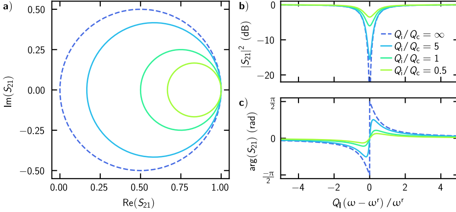
Figure 2.4: S_{21} -parameter of a notch-type resonator for different coupling regimes. In the complex plane a) , frequency sweeps around the resonant frequency feature circles, starting and ending at the off-resonant point S_{21} = 1 . The diameter of the circle increases with the ratio of Q_i/Q_c and tends to 1 for Q_i/Q_c \rightarrow \infty (dashed). The squared amplitude b) shows Lorentzian dips, the deeper the larger Q_i/Q_c and the phase signal c) maximally rolls off from -\pi/2 to \pi/2 for Q_i/Q_c \rightarrow \infty .
