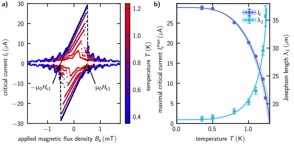
Figure 4.6: Magnetic diffraction pattern of a 110 \mu\text{m} \times 5 \mu\text{m} long junction of trilayer B in inline geometry at different temperatures. a) The linear decrease of the Meissner phase confirms reaching the LJJ limit and the extrapolated root of the main lobe corresponds to \pm H_{c1} . The asymmetric lobes of the magnetic field-dependent critical current arise because of inhomogeneously distributed bias currents in inline junctions in combination with different inductances in the two electrodes [Sch70; BJV75; Mon+13] (This figure is also published in Ref. [Wil+22].) b) The maximum of the main lobe decreases for higher temperatures according to the Ambegaokar-Baratoff model of S_1IS_2 junctions with different superconducting gaps \Delta_j(T) , whereas the Josephson length increases because of the temperature-dependent kinetic inductance.
