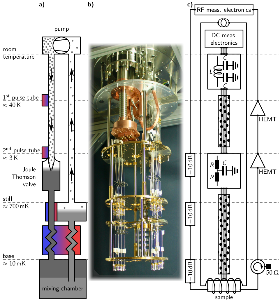
Figure 3.4: Cryogenic measurement setup. a) The cryostat is a multistep refrigerator, whose pre-cooling unit is a two-stage pulse tube generating about 40 K and 3 K, respectively, that is thermally coupled by heat exchangers to the primary dilution refrigerator. By means of a Joule-Thomson valve in this ^3\text{He}/^4\text{He} cycle, temperatures at still of about 700 mK are reached, which suffices to obtain a separation into a concentrated and a dilute phase of the ^3\text{He}/^4\text{He} and run the dilution refrigeration cycle. Thereby, ^3\text{He} is pumped down at still from the dilute phase and recondensed to ensure continuous cooling. b) The photograph of a Bluefors LD250 refrigerator shows the implementation used in this work, including the wiring. c) The measurement framework consists of low-pass filtered DC wires, coaxial RF lines, and high-current supply lines for magnetic coils.
