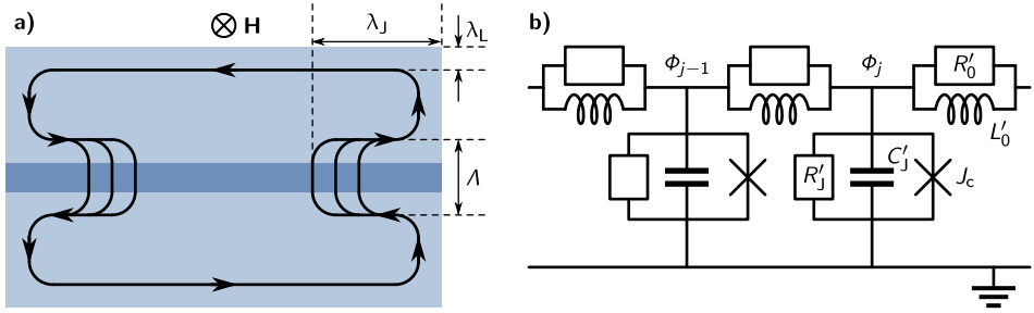
Figure 2.16: Schematic screening currents and equivalent circuit of long Josephson junctions.
