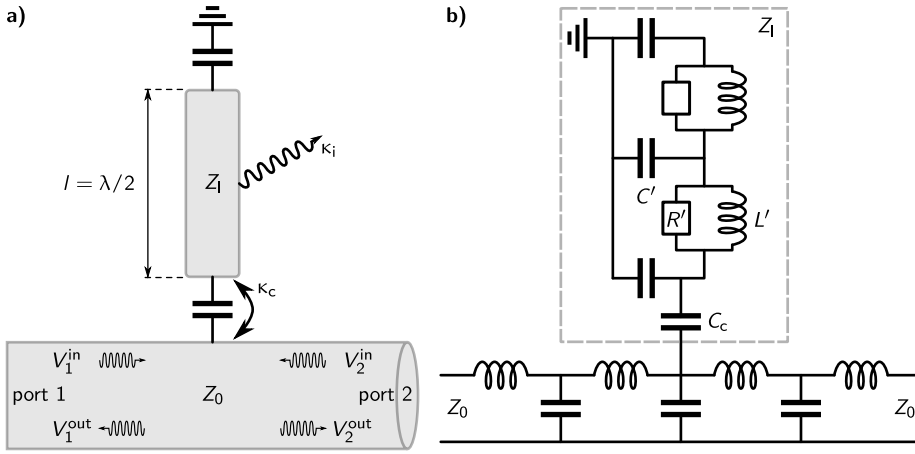
Figure 2.3: Schematic of a half-wavelength notch-type resonator embedded in a two port-network. a) The particular notch-type configuration consists of a LC transmission line with specific impedance Z_0 = \sqrt{L/C} that is shunted to ground via a load with impedance Z_1 . In the present case, this load is a terminated transmission line whose two open ends define a distributed \lambda/2 resonator. The two-port network of this assembly is characterized by relating the incident and scattered microwaves at both ports of the transmission line. The coupling between feedline and resonator is assumed to be capacitive with loss rate \kappa_c and the resonator itself has an internal linewidth \kappa_i . b) As a schematic circuit, the infinite transmission line is modeled as an inductive waveguide that is capacitively shunted to ground. The distributed RLC -resonator has a well-defined length, whose impedance mismatch at the open ends forms a resonating cavity.
