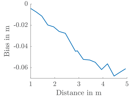
Fig. 8. Difference between the ground truth depths and the measured depths at difference distances. The negative bias means that the measured values are smaller than the ground truth.
