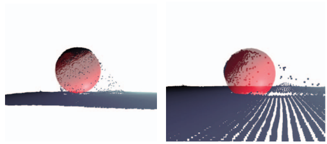
Fig. 17. Point cloud of the plastic sphere being observed by the iPad depth sensor. Best-fitting sphere overlaid in red. Floor appears wider at 2 m due to the field of view. (a) Sphere at 1 m. (b) Sphere at 2 m.
