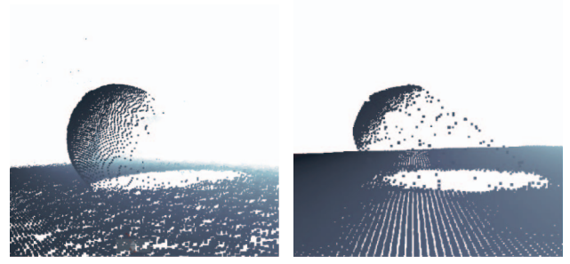
Fig. 15. Plastic sphere of radius 15 cm lying on the ground, being observed from a distance of 2 m by a Kinect 2 and an iPad depth sensor. (a) Sphere, Kinect 2. (b) Sphere, iPad.
