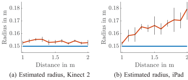
Fig. 16. Estimated radius of the sphere for the Kinect 2 and the iPad, viewed from different camera distances. Ground truth in blue, result means in red, and standard deviations in black (vertical lines). (a) Estimated radius, Kinect 2. (b) Estimated radius, iPad.
