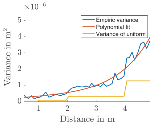
Fig. 10. Empiric variance of measurement noise at different distances, and a best-fitting polynomial fit.
