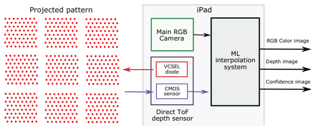
Fig. 4. Sketch of the depth capture process: a pattern of 576 dots is projected onto the scene, their distances are measured by the depth sensor, and the result is fused with the data from the RGB camera. The result are three streams: the color image, the depth image, and the confidence image.
