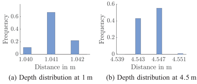
Fig. 9. Representative probability distributions for nonfringe depths values at different distances. The gaps between values are due to the discretization. (a) Depth distribution at 1 m. (b) Depth distribution at 4.5 m.
