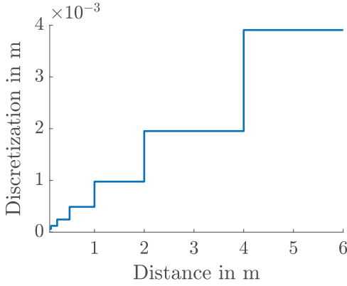
Fig. 7. Discretization of depth values, i.e., the distance between a value and the next possible one, depending on the distance.
