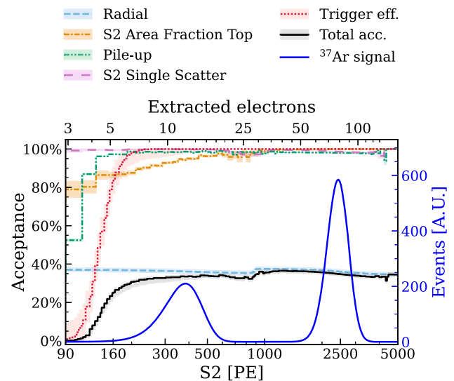
Fig. 9 Acceptances (fraction of ^{37}\text{Ar} events accepted) of the quality cuts and trigger efficiency depending on S2 size for the slice -50 \text{ cm} < z < -30 \text{ cm} . The bands around the lines represent the \pm 1\sigma uncertainties. The ^{37}\text{Ar} signal model (without acceptances applied) is shown with a blue solid line. The number of extracted electrons corresponding to S2 is reported on top axis
