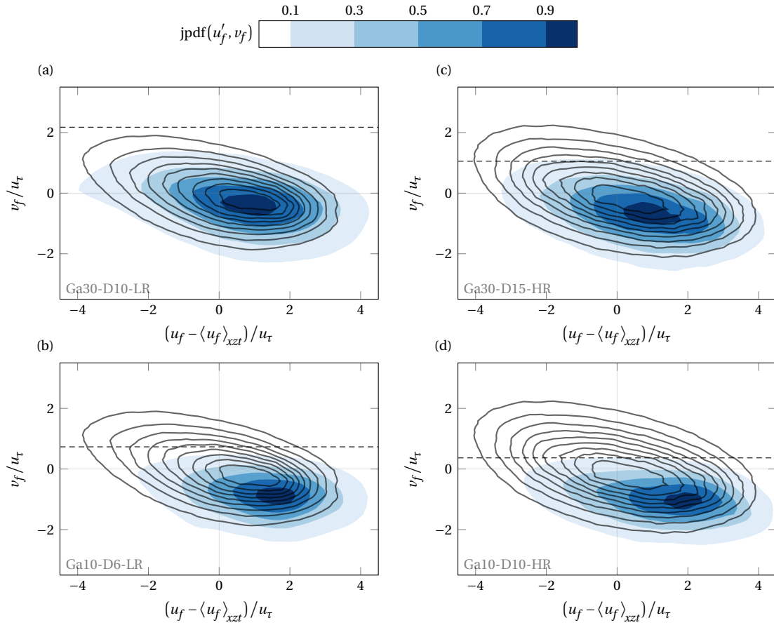
Figure 5.10: Joint probability density function of the streamwise and vertical components of the fluid velocity conditioned to the contaminants, \text{jpdf}([u'_f]_{\mathcal{S}X_1}, [v'_f]_{\mathcal{S}X_1}) (shaded regions) and the unconditioned fluid velocity, \text{jpdf}(u'_f, v'_f) , (contour lines) at y = 0.3H_f for all downward crossings. The data is presented as a function of the velocity fluctuations, which means that the mean unconditioned streamwise velocity at the position shown is subtracted from the conditioned and unconditioned streamwise velocities alike. The colouring corresponds to \{0.1, 0.3, 0.5, 0.7, 0.9\} times the respective maximum value of the distribution. An indicator for the inverse of the relative turbulence intensity for each case is given by the dashed line which is located at v_f = v_{p,\infty} (---). The following cases are arranged in column-major order: (a) G30-D10-LR, (b) G10-D6-LR, (c) G30-D15-HR and (d) G30-D10-HR.
