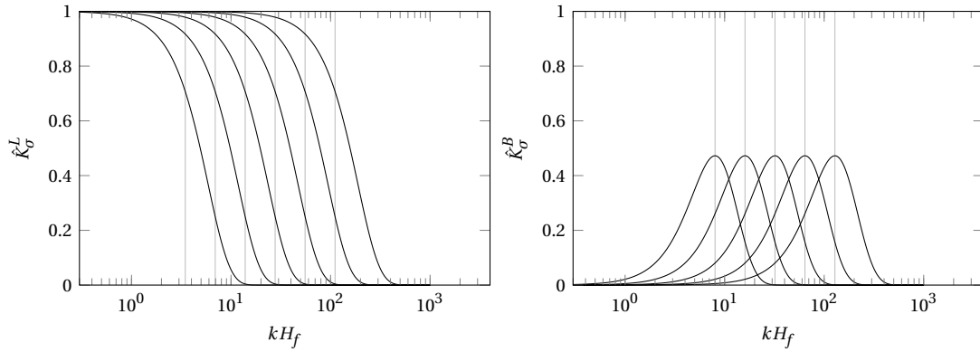
Figure C.1: Spectral support of the low-pass filters (left) and the derived band-pass filters (right).
