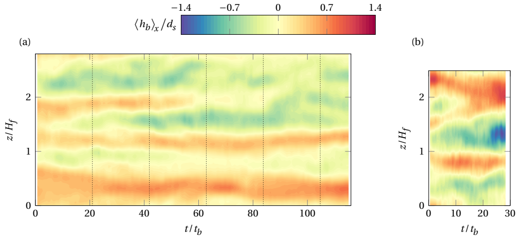
Figure 3.3: Temporal evolution of the streamwise-averaged fluid-sediment interface \langle h_b(x, z, t) \rangle_x for the featureless background flows. (a) LR, Re_\tau = 241 . (b) HR, Re_\tau = 838 . The dotted vertical lines mark the initial conditions for the transient settling problem aside from t = 0 , cf. §3.6. The evolution of the bed is shown in absence of contaminant particles.
