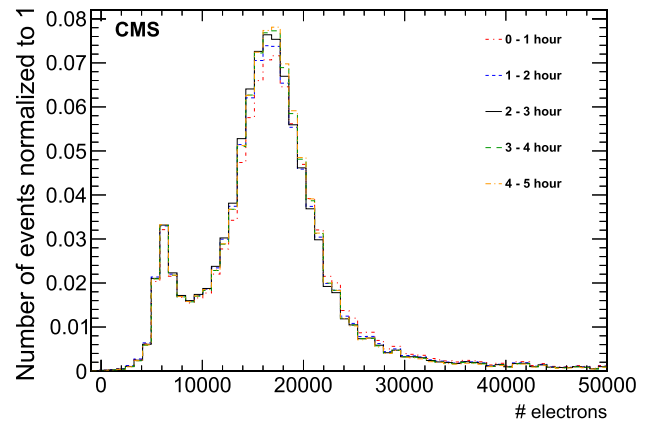
Fig. 12 Pulse height distributions for fill 6035 in 2016, divided into 1-h intervals, where each color represents a separate interval. Since each interval may not contain the same number of events, each individual histogram is normalized to a total of 1
