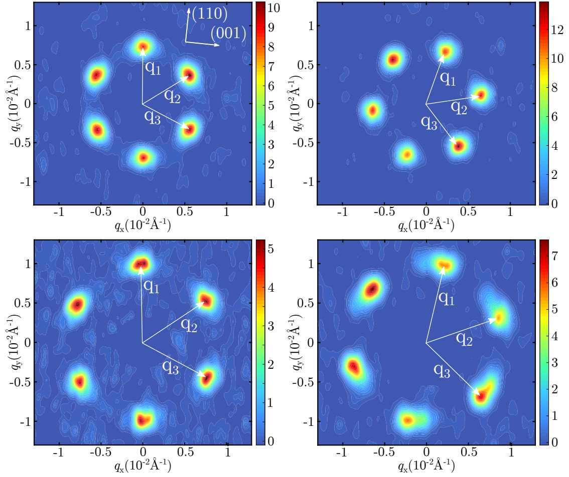
Figure 1: Diffraction patterns from the VL at several fields and different thermodynamic preparation paths. (a) VL at 0.2 T after ZFC. (b) VL at 0.2 T after decreasing the magnetic field from 1 T. (c) VL at 0.4 T after ZFC. (d) VL at 0.4 T after decreasing the field from 1 T.
