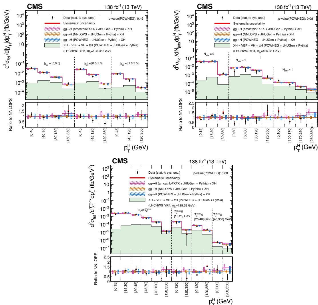
Figure 24. Double differential cross sections in bins of |y_{\text{H}}| vs. p_{\text{T}}^{\text{H}} (upper left), number of associated jets vs. p_{\text{T}}^{\text{H}} (upper right), and \mathcal{T}_{\text{C}}^{\text{max}} vs. p_{\text{T}}^{\text{H}} (lower). The binnings of the various measurements are reported in table 6. The content of each plot is described in the caption of figure 6.
