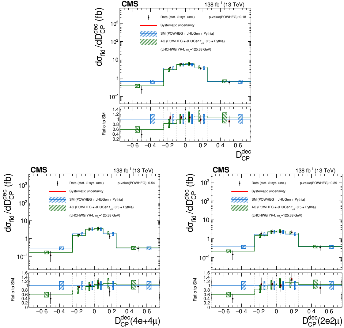
Figure 20. Differential cross sections as functions of the matrix element kinematic discriminant D_{CP}^{dec} in the 4 \ell (upper) and in the same-flavor (lower left) and different-flavor (lower right) final states. The green histogram shows the distribution of the discriminant for the HVV anomalous coupling scenario corresponding to f_{a3} = 0.5 . The subdominant component of the signal (VBF + VH + t\bar{t}H ) is fixed to the SM prediction. The hatched areas correspond to the systematic uncertainties in the theoretical predictions. Black points represent the measured fiducial cross sections in each bin, black error bars the total uncertainty in each measurement, red boxes the systematic uncertainties. The lower panels display the ratios of the measured cross sections and of the predictions from POWHEG and MADGRAPH5_aMC@NLO to the NNLOPS theoretical predictions.
