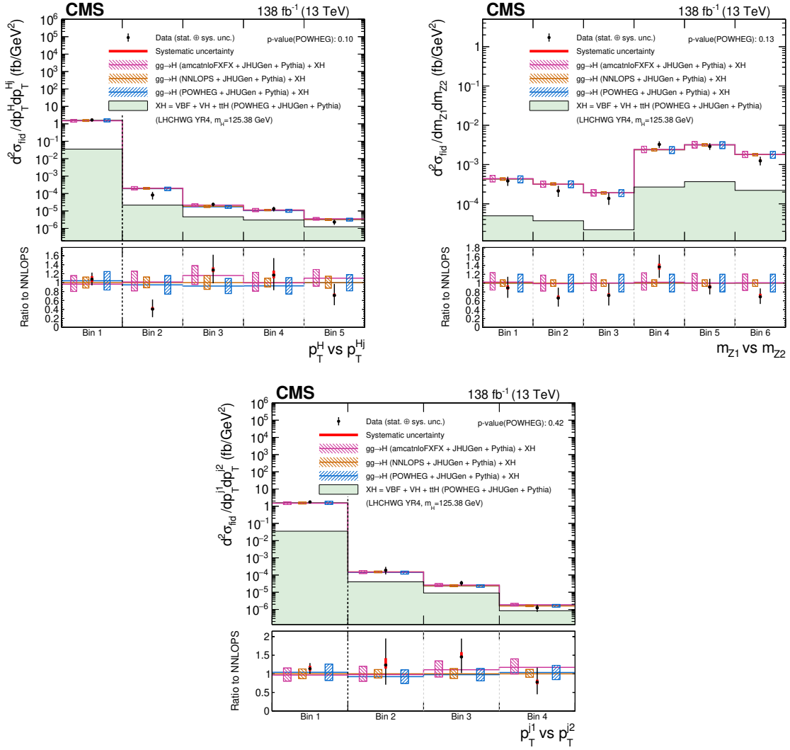
Figure 25. Double differential cross sections in bins of p_T^{Hj} vs. p_T^H (upper left), m_{Z1} vs. m_{Z2} (upper right), and p_T of the leading vs. subleading jet (lower). The binnings of the various measurements are reported in table 6. The content of each plot is described in the caption of figure 6.
