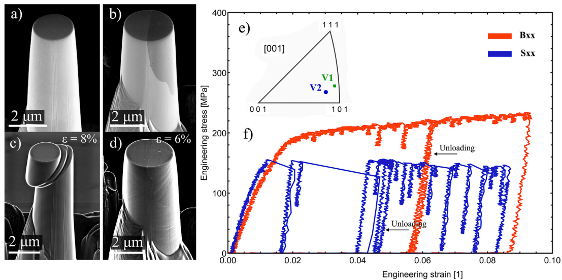
Fig. 6. Pre- and post-mortem SEM micrographs of a Sxx a) and c), and Bxx pillar b) and d) in [1\bar{3}\bar{4}] direction. The post-mortem images are sharpened for better visibility of slip traces. e) Inverse pole figure of the compression direction of the two grains. f) shows the stress–strain curve of the Sxx and Bxx. The Bxx deforms at higher stresses and shows fewer load drops. Arrows mark the intentional unloading steps.
