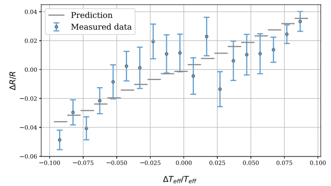
Fig. 8 Plot depicting the predicted and measured relative neutrino rate against the relative temperature variations bins. The slope corresponds to \alpha . The prediction is made using MCEq with the SIBYLL 2.3c hadronic interaction model
