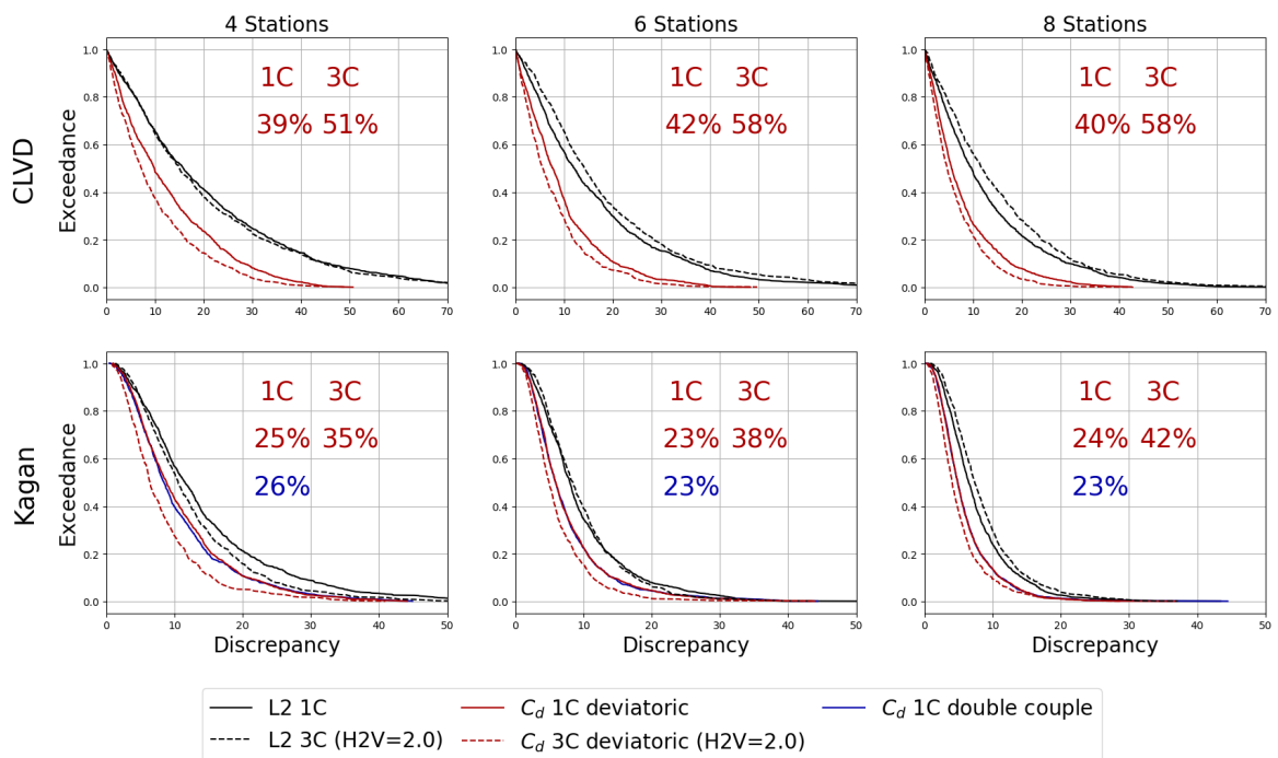
Figure 8: Comparison of a vertical trace (1C) data restricted inversion versus a three component (3C) inversion in a synthetic noise test at 50% vertical base amplitude. Displayed PDF curves follow the same notation as in figure 6.
