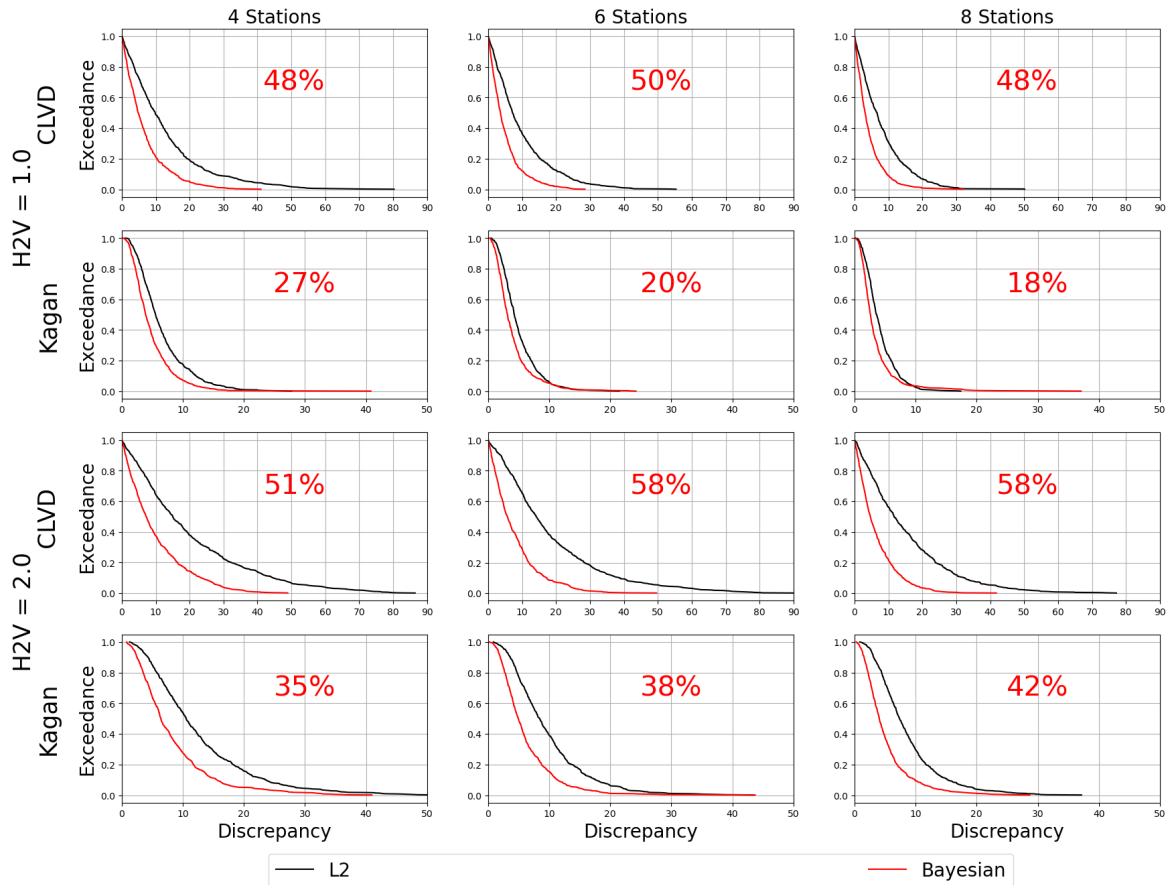
Figure 6: Synthetic noise test with base amplitude level at 50% of vertical peak signal. Surveyed in a random study (station location, noise, and true source mechanism) are the discrepancies in Kagan angle and CLVD percentage between the true solution and the inversion results. The examinations were conducted for a random network consisting of 4, 6, and 8 stations at a horizontal H2V amplification factor of 1.0 and 2.0. Displayed PDF curves represent the ascending discrepancy normalized at the absolute number of the result samples (>1000). Marked as black curves are the results for a simple linear inversion while red is a Bayesian formulation using a data covariance matrix C_d in a deviatoric tree-importance sampling. Corresponding percentage values are the relative reduction of the curve integral between the L2 to the Bayesian formulation.
