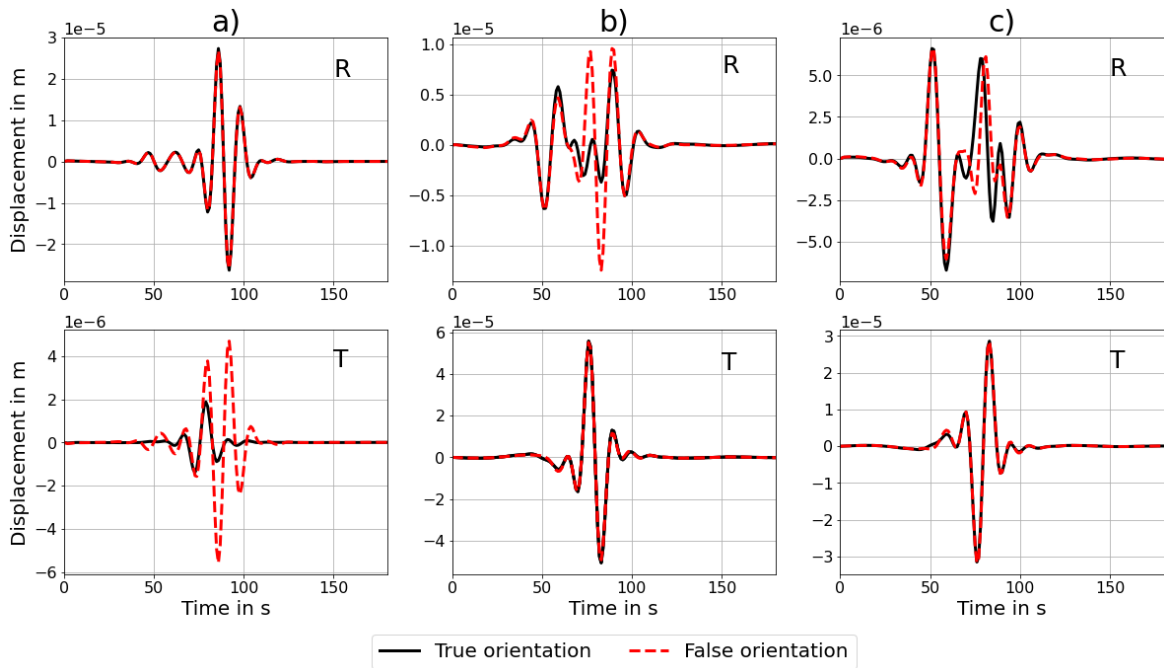
Figure 2: Influence of d\alpha = 10^\circ station alignments of horizontal recordings for different source mechanism and station azimuth \theta from a synthetic test. R = Radial; T = Transverse component. a) Dip-Slip (\psi, \delta, \lambda) = (0, 90, 90) , \theta = 80^\circ near p-axis ( 90^\circ ), energy on T gets minimal b) Strike-Slip (\psi, \delta, \lambda) = (0, 90, 0) , \theta = 20^\circ near n-axis ( 0^\circ ), energy on R gets minimal c) Normal Fault (\psi, \delta, \lambda) = (0, 45, -90) , \theta = 30^\circ near p-axis ( 45^\circ ), energy on R gets minimal
