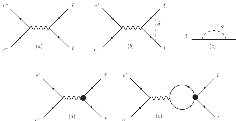
Figure 1: e^+e^- \rightarrow t\bar{t} in a toy model. (a): Lowest-order amplitude. (b), (c): Leading corrections from S -scalar exchange (mass M ) in the full theory. (d), (e): Contributions needed to reproduce the 1/M^2 corrections of the full theory within the EFT. The black dots represent local operators of dimension 6. They contribute at tree level ( Q_2, Q_3 in (d)) and at one loop ( Q_1 in (e)). See text for further explanation.
