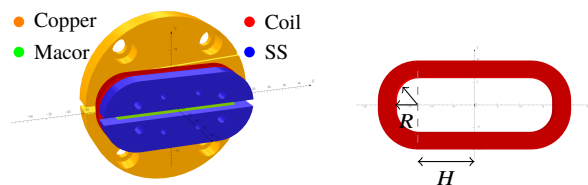
Figure 1: 3D drawing of the model of the SC coil. Markers in the legend indicate different parts by their color (left panel). 2D drawing in the xy plane for the racetrack coil. The symbols H and R show the coil's half length and arc radius, respectively (right panel).
