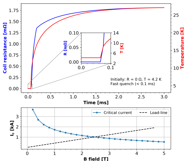
Figure 3: Resistance (blue) and hot spot temperature (red) of the NbTi coil over the pulse time. A magnifying inset is showing the moment when the coil switches to resistive mode around 75 \mu\text{s} (upper panel). The critical current of NbTi as a function of the B field at a fixed temperature of 4.2 K (blue) together with the load-line (black) estimated for the existing coil geometry (lower panel).
