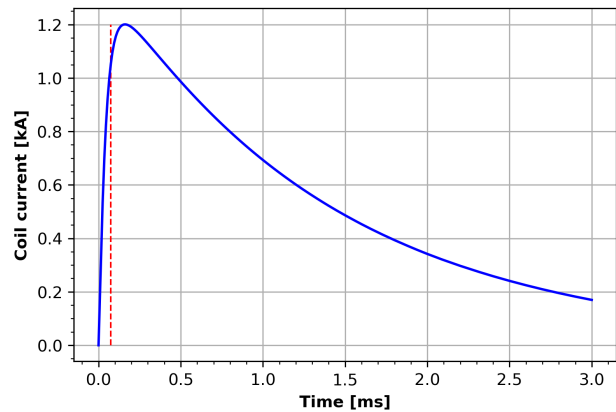
Figure 2: Generated pulse wave-form (blue). The dashed line indicates the time when transition to normal state occurs.
