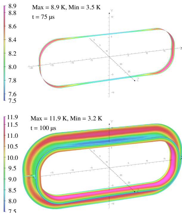
Figure 4: Local distribution for the coil's temperature at the times 75 \mu\text{s} (upper panel) and 100 \mu\text{s} (lower panel). Values of the coil's hot and cold spots at each time are indicated. A constraint on the minimum temperature set to 7.5 K is made to demonstrate the quench propagation in different directions.
