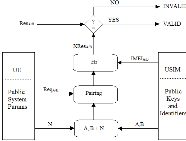
Figure 3: User-to-User authentication
