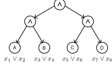
Figure 1: Merge construction tree
