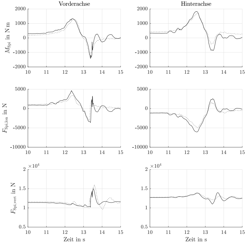
Abbildung C.11: Messung #578
