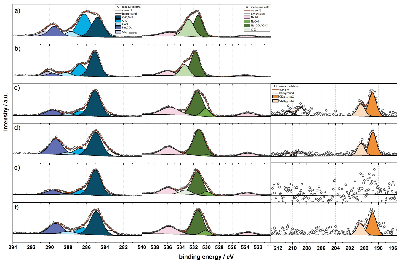
Figure 13. C 1s, O 1s and Cl 2p spectra of the sodium surfaces after storage in different electrolytes: pure PC solvent for 2 min (a) and 2 h (b), 0.75 M PC NaClO 4 for 2 min (c) and 2 h (d), 0.75 M PC-VC NaClO 4 for 2 min (e) and 2 h (f). The binding energy scale is calibrated versus the hydrocarbon peak at 285 eV.
