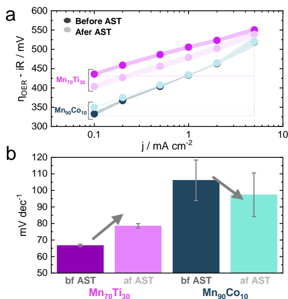
Figure 5: Tafel analysis of \text{Mn}_{70}\text{Ti}_{30}\text{O}_x and \text{Mn}_{90}\text{Co}_{10}\text{O}_x . (a) Tafel plot for both samples before and after AST. Standard deviation calculated from duplicates. (b) Tafel slopes calculated from (a) before and after the AST.
