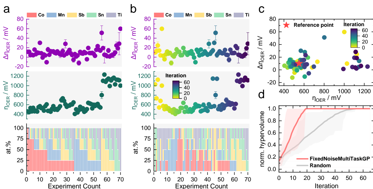
Figure 2: Simulated MOBO on a data set from a grid search campaign. (a) Summary grid search data showing overpotential, overpotential change, and corresponding composition. Standard deviation calculated from two duplicates. (b) Rearrangement of data shown in (a) as a result of MOBO sampling. Color code indicating MOBO iterations. (c) Pareto plot of \Delta\eta_{\text{OER}} against \eta_{\text{OER}} for each composition with a color map indicating MOBO iterations. (d) Normalized hypervolume plotted against MOBO iterations. MOBO is benchmarked against random sampling.
