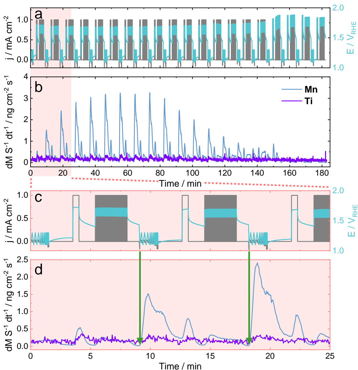
Figure S 11: Operando dissolution of \text{Mn}_{70}\text{Ti}_{30}\text{O}_x . (a) Current density and potential. (b) Dissolution rate of Mn and Ti. (c) Exploded view of highlighted area in (a). (d) Exploded view of highlighted area in (b). Green arrow indicating time where potentiostat switch from galvanostatic to potentiostatic mode.
