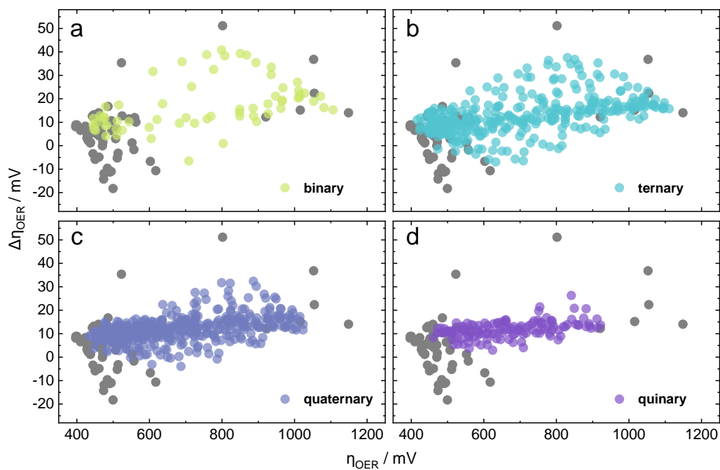
Figure S 9: Prediction of FixedNoiseMultitaskGP on remaining compositions after training on observations made during the MOBO experiments (grey). (a) Binary. (b) Ternary. (c) Quaternary. (d) Quinary.
