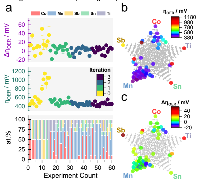
Figure 4: Experimental optimization of the Co-Mn-Sb-Sn-Ti oxide composition for OER in 0.1 M HNO 3 with MOBO. (a) Measured \eta_{\text{OER}} and \Delta\eta_{\text{OER}} of initial and subsequent compositions suggested by MOBO. Color mapping indicating MOBO iteration. Standard deviation calculated from triplicates. (b) MDS plot of \eta_{\text{OER}} for compositions shown in panel (a) (colored points). The grey points indicate the total composition space available for MOBO sampling. (c) Similar to panel (b) but plotting \Delta\eta_{\text{OER}} .
