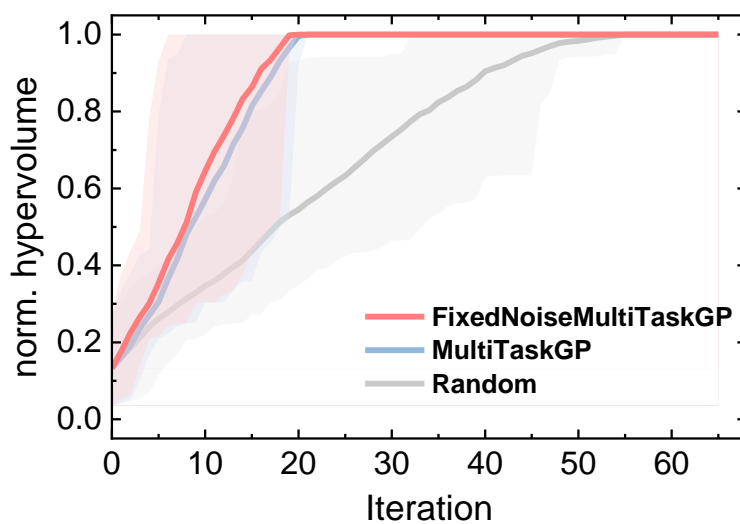
Figure S2: MOBO performance of different models based on the grid search data set.
