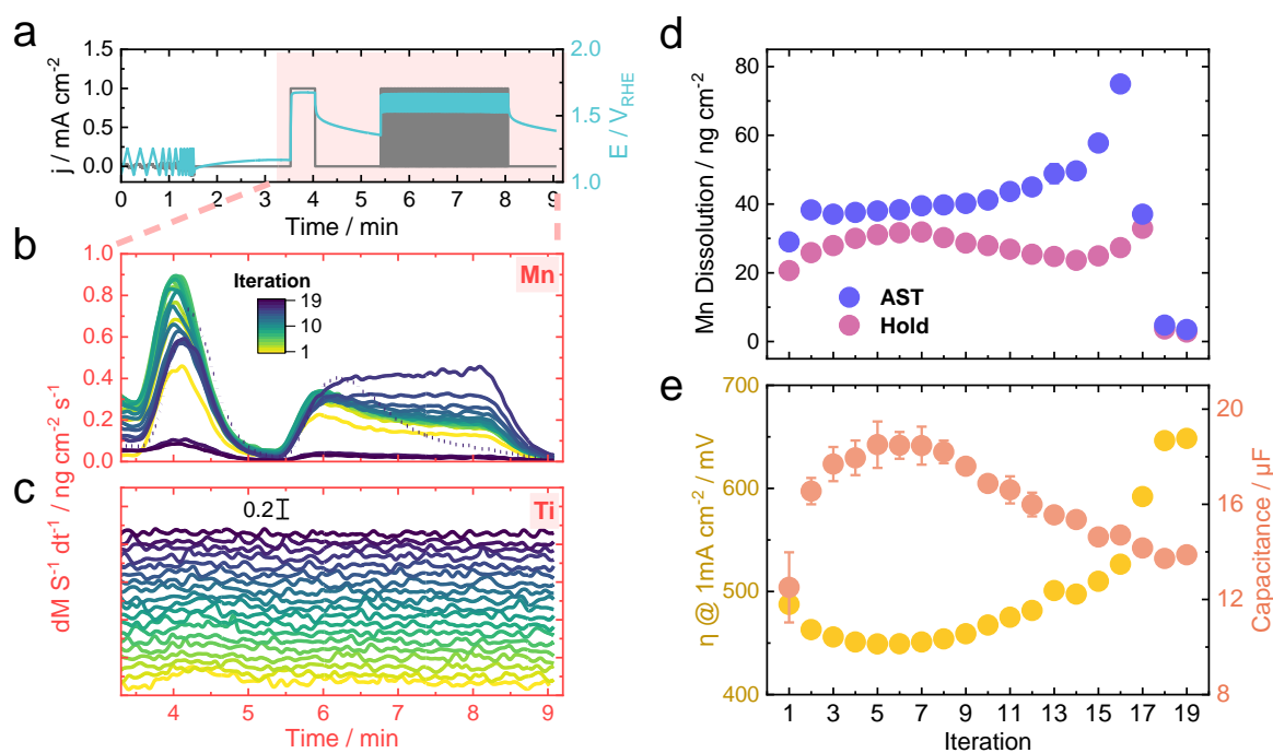
Figure 6: Operando ICP-MS measurement of \text{Mn}_{70}\text{Ti}_{30}\text{O}_x in 0.1 M \text{HNO}_3 . (a) Applied electrochemical protocol. The protocol was repeated 19 times. (b) Dissolution rate of Mn during CP hold and AST. Dotted line highlighting full deactivation of the catalyst. (c) Dissolution rate of Ti during CP hold and AST. (d) Amount of dissolved Mn during the CP hold and AST. (e) Measured overpotential at the first 1 \text{mA cm}^{-2} hold and the extracted capacitance from the initial CVs. Standard deviation calculated from duplicates.
