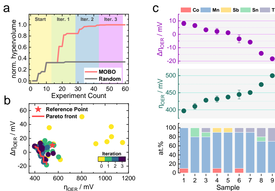
Figure 3: Performance and Pareto front extracted during Experimental optimization of the Co-Mn-Sb-Sn-Ti oxide composition. (a) Normalized hypervolume plotted against MOBO iterations. MOBO is benchmarked against random sampling. (b) Plotting \Delta\eta_{\text{OER}} against \eta_{\text{OER}} for each composition with a color map indicating MOBO iterations. (c) \eta_{\text{OER}} and \Delta\eta_{\text{OER}} for the observed Pareto compositions. Standard deviation calculated from triplicates.
