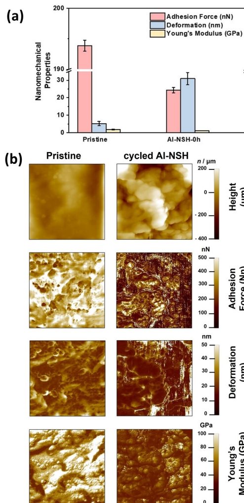
Figure 12. (a) Summary of the nanomechanical characterization results before and after cycling (without any pretreatment). Nanomechanical properties of pristine and cycled Al foil in [\text{EMIm}]\text{Cl}/\text{AlCl}_3 ILE. Error bars reflect standard deviations from data for three different spots at one sample. (b) Nanomechanical characterization of pristine and cycled Al-NHS (non-pretreated), recorded image of height, adhesion force, deformation, and Young's modulus. Scale = 5 \times 5 \mu\text{m}^2 .
